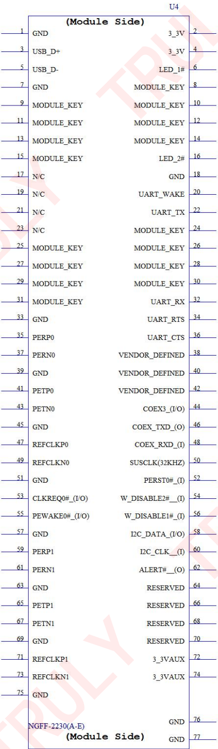
Figure 2.Pin Diagram of TR7R922P2-M
