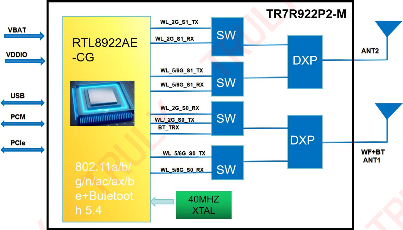
Figure 1. Block Diagram of TR7R922P2-M
