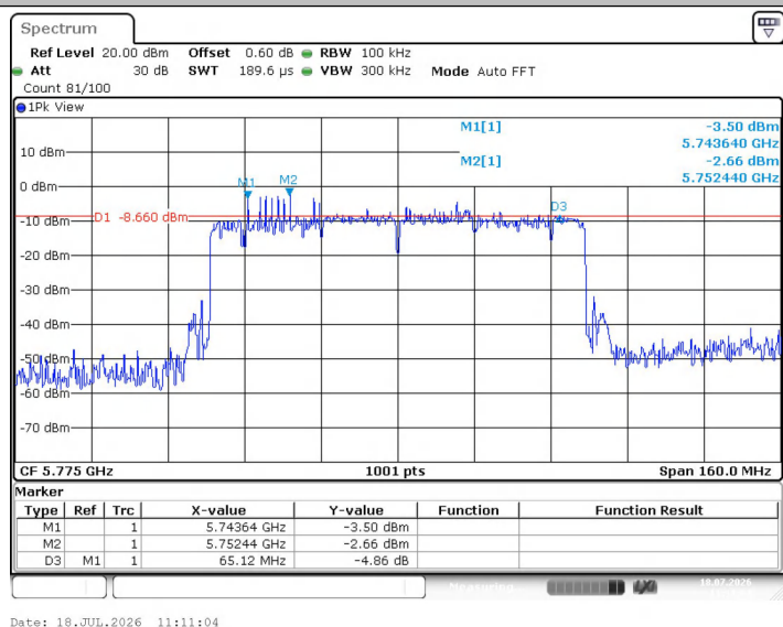
11AX80SISO_Ant2_5775
