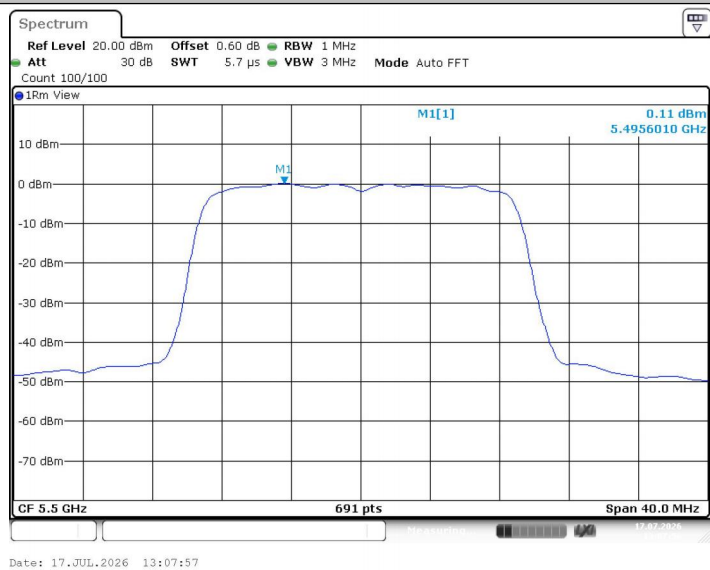
11AC20SISO_Ant2_5500
