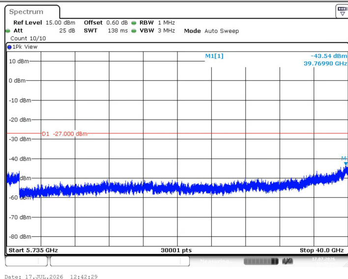
11N40SISO_Ant2_5550_5735~40000
