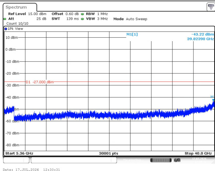
11N40SISO_Ant2_5190_5360~40000
