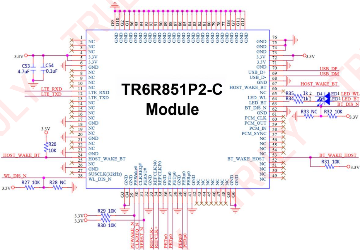
Figure 3. Application Schematic Diagram of TR6R851P2-C
