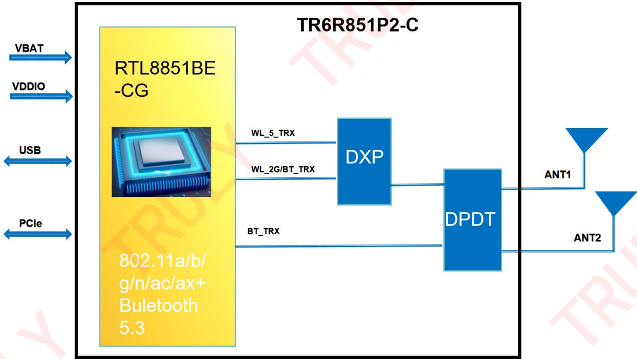
Figure 1. Block Diagram of TR6R851P2-C
