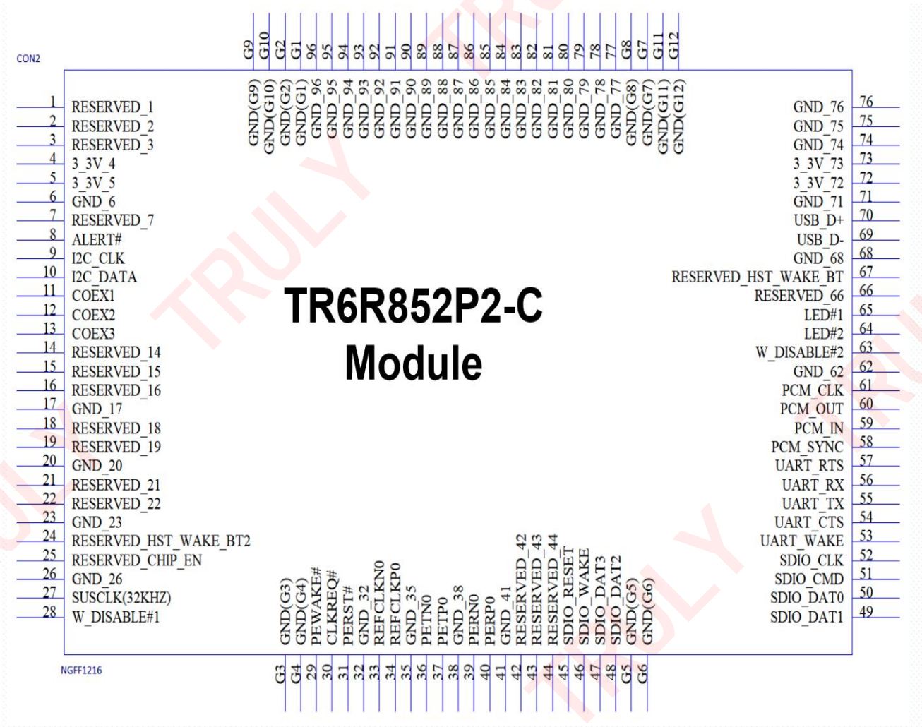
Figure 2.Pin Diagram of TR6R852P2-C
