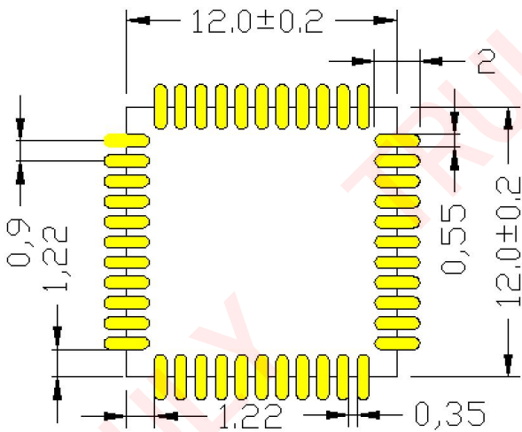
Figure 5. On Board Pad Suggest: (Unit: mm)
