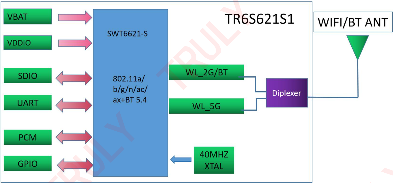
Figure 1. Block Diagram of TR6S621S1
