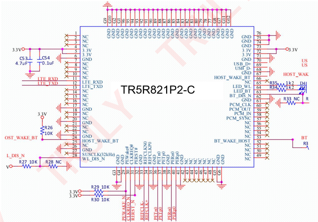
Figure3. Application Schematic Diagram of TR5R821P2-C
