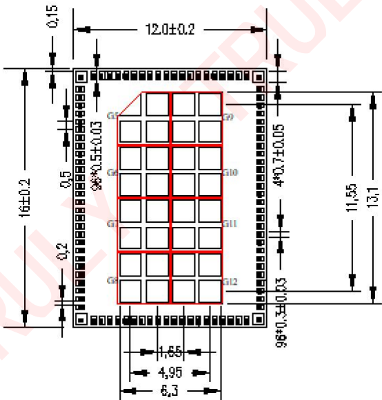
Figure 5. On Board Pad Suggest: 0.5*0.3 (Unit: mm)
