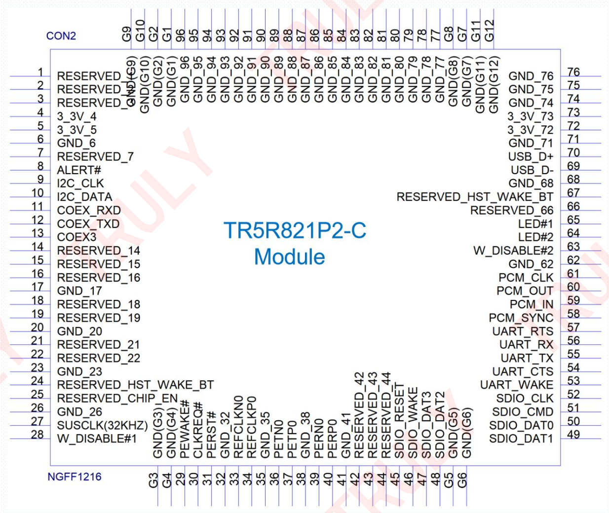
Figure 2.Pin Diagram of TR5R821P2-C
