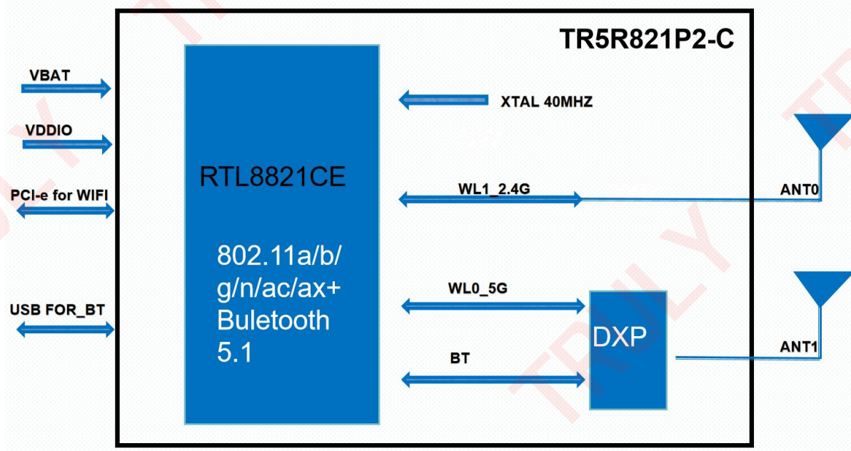
Figure 1. Block Diagram of TR5R821P2-C
