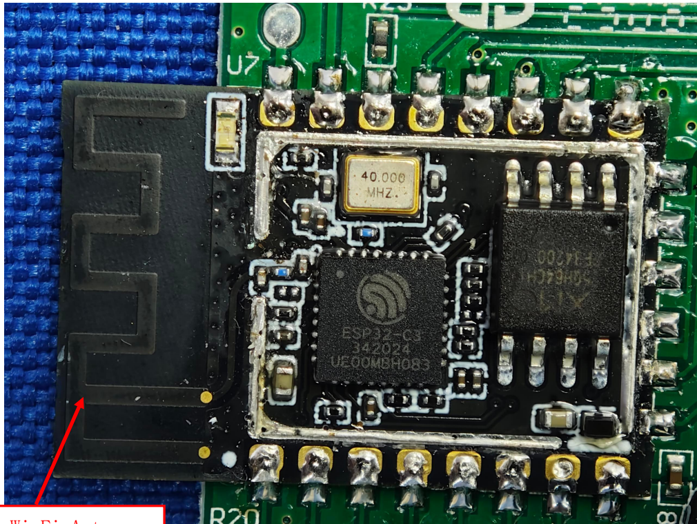
BLE/2.4G Wi-Fi Antenna
