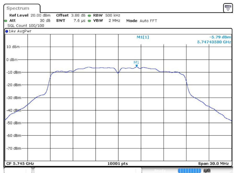
PSD ac20 5745MHz Ant1
