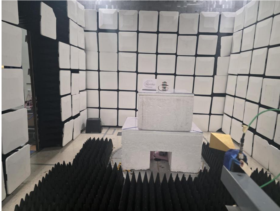
Figure 7 - Radiated emissions above 1 GHz (26 – 40 GHz), front view.
