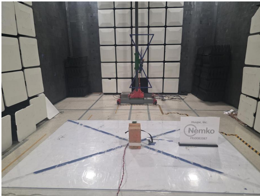
Figure 2 - Radiated emissions below 1 GHz (0.03 – 1 GHz), rear view.
