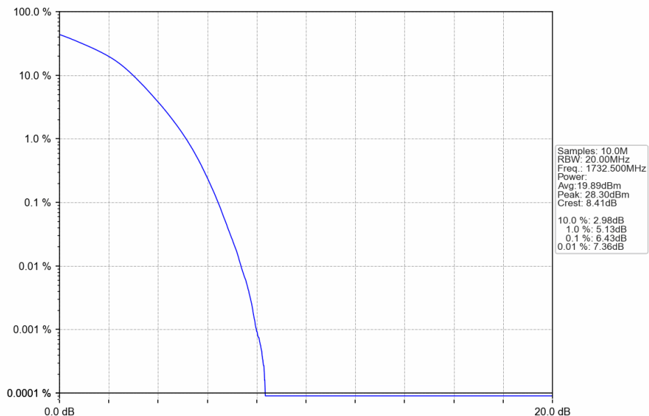
Band4_20MHz_16QAM_MCH_1732.5MHz_RB_100_0_NTNV
