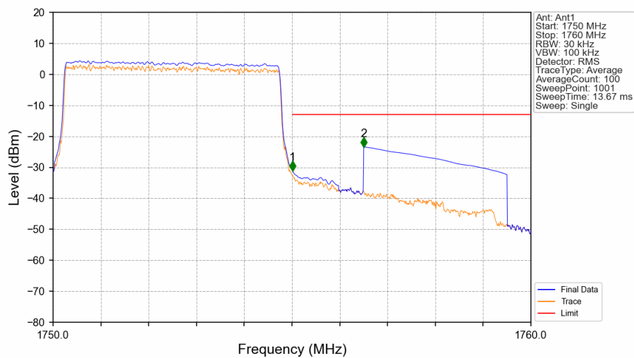
Band4_5MHz_QPSK_HCH_1752.5MHz_RB_25_0_NTNV
