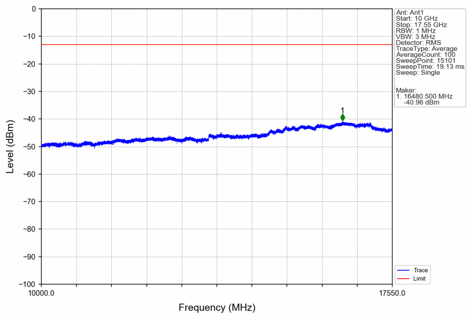
Band4_1.4MHz_16QAM_MCH_1732.5MHz_RB_1_0_NTNV
