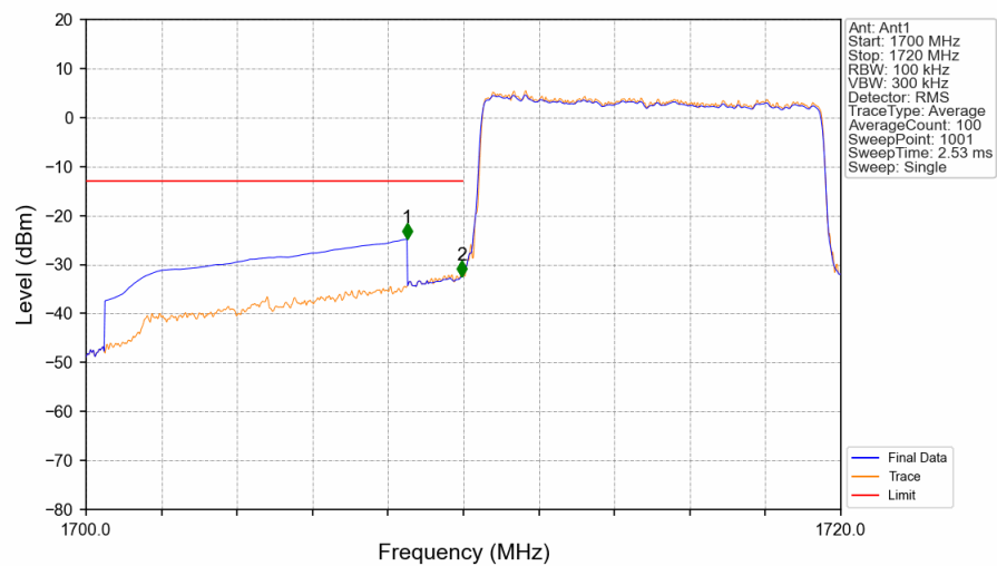
Band4_10MHz_QPSK_LCH_1715MHz_RB_50_0_NTNV
