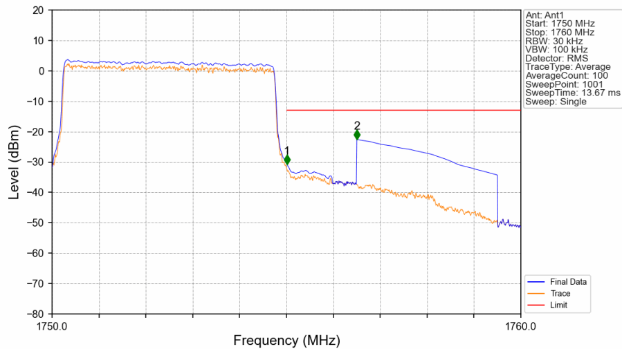
Band4_5MHz_16QAM_HCH_1752.5MHz_RB_25_0_NTNV
