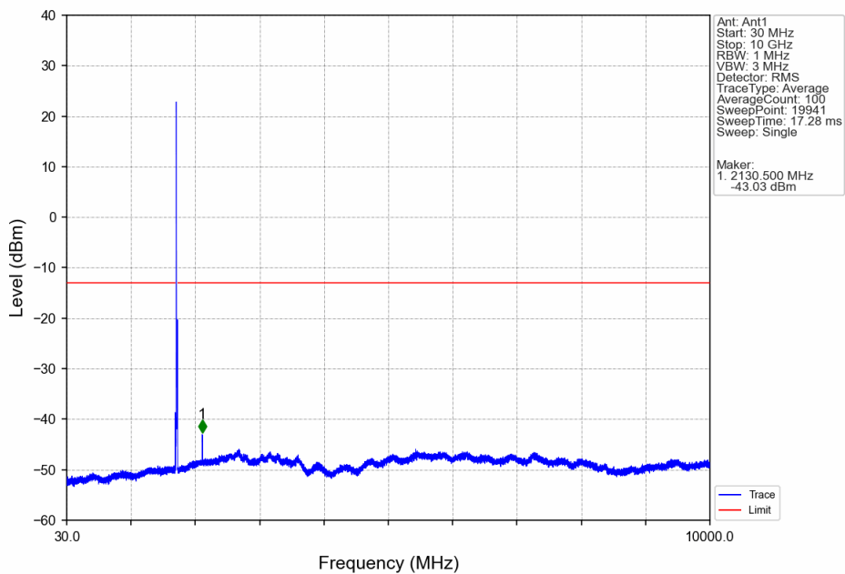
Band4_10MHz_QPSK_MCH_1732.5MHz_RB_1_0_NTNV
