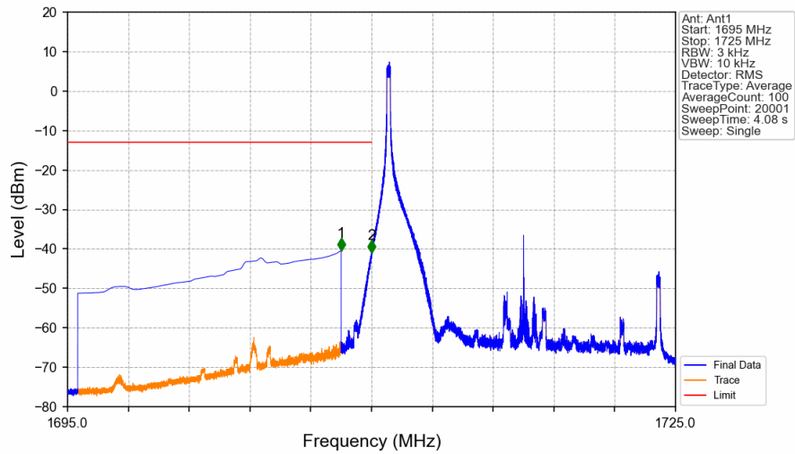
Band4_15MHz_16QAM_LCH_1717.5MHz_RB_1_0_NTNV
