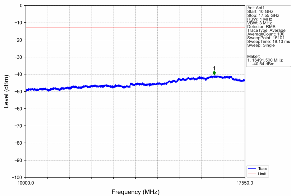
Band4_1.4MHz_16QAM_HCH_1754.3MHz_RB_1_0_NTNV
