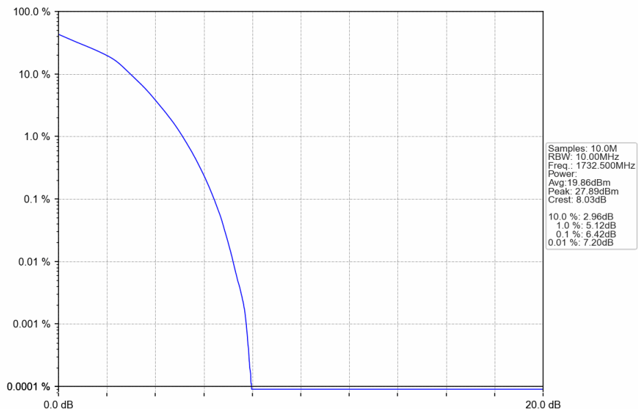
Band4_10MHz_16QAM_MCH_1732.5MHz_RB_50_0_NTNV
