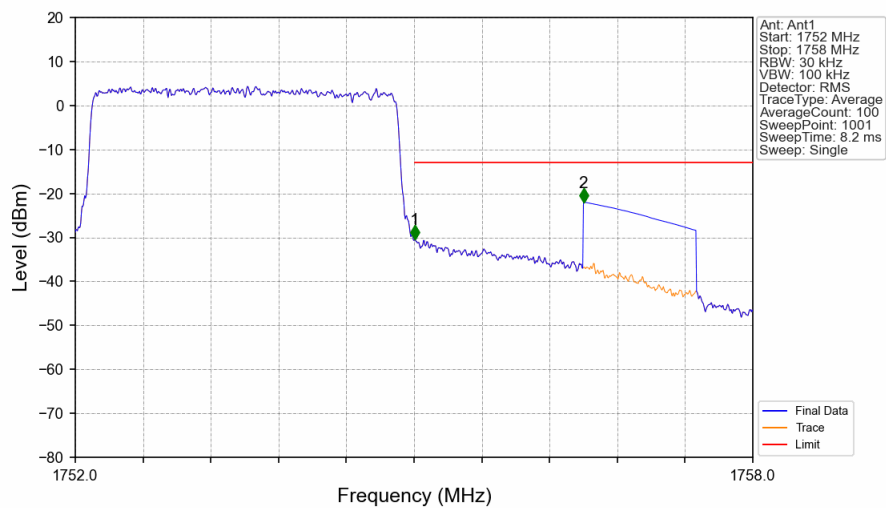
Band4_3MHz_16QAM_HCH_1753.5MHz_RB_15_0_NTNV
