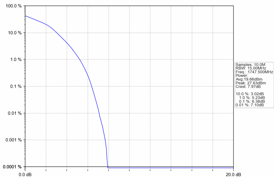
Band4_15MHz_16QAM_HCH_1747.5MHz_RB_75_0_NTNV
