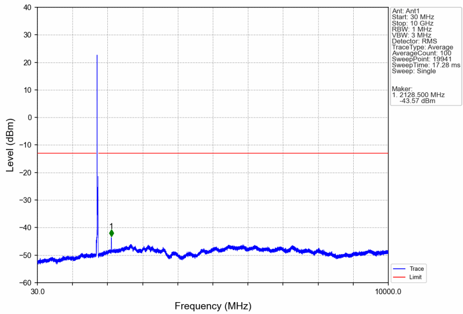
Band4_15MHz_QPSK_MCH_1732.5MHz_RB_1_0_NTNV
