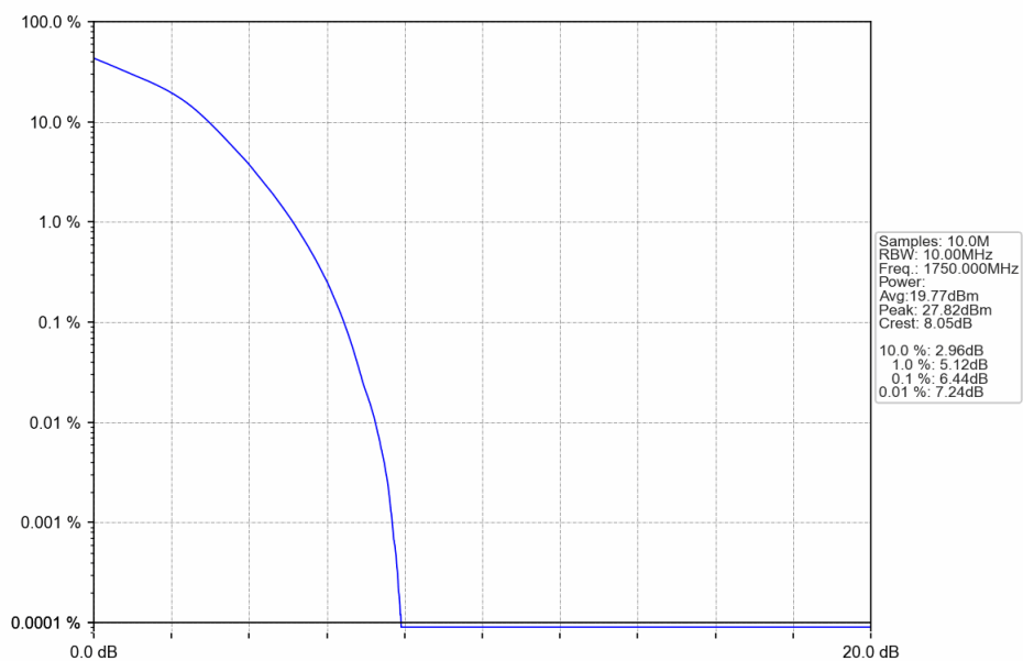
Band4_10MHz_16QAM_HCH_1750MHz_RB_50_0_NTNV
