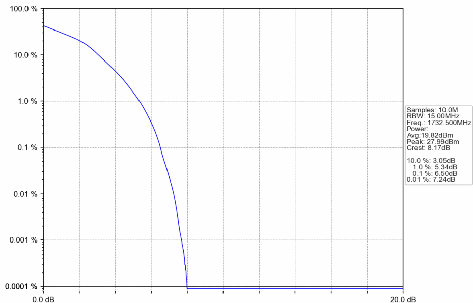
Band4_15MHz_16QAM_MCH_1732.5MHz_RB_75_0_NTNV
