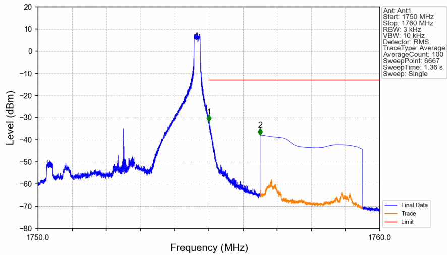
Band4_5MHz_QPSK_HCH_1752.5MHz_RB_1_24_NTNV
