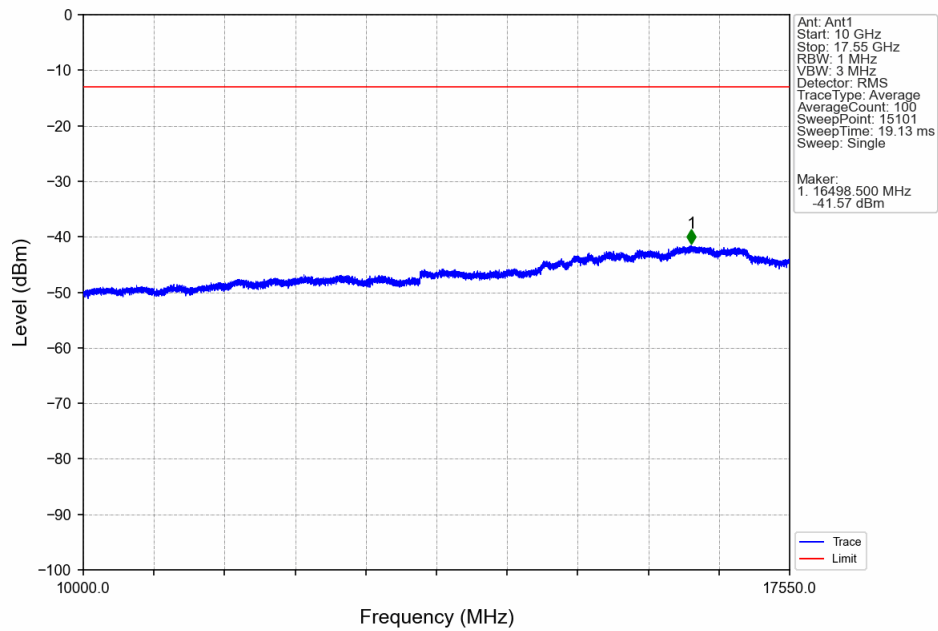
Band4_3MHz_QPSK_LCH_1711.5MHz_RB_15_0_NTNV
