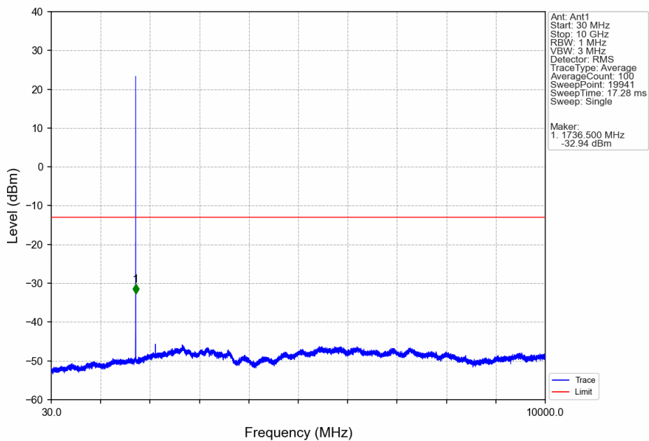
Band4_1.4MHz_QPSK_MCH_1732.5MHz_RB_1_0_NTNV
