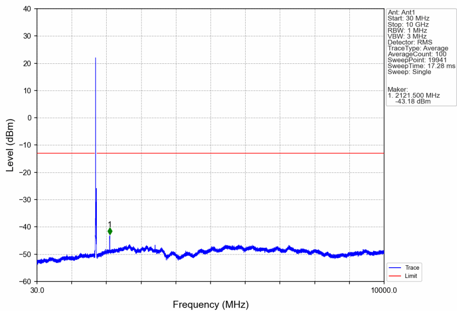
Band4_15MHz_16QAM_LCH_1717.5MHz_RB_1_0_NTNV
