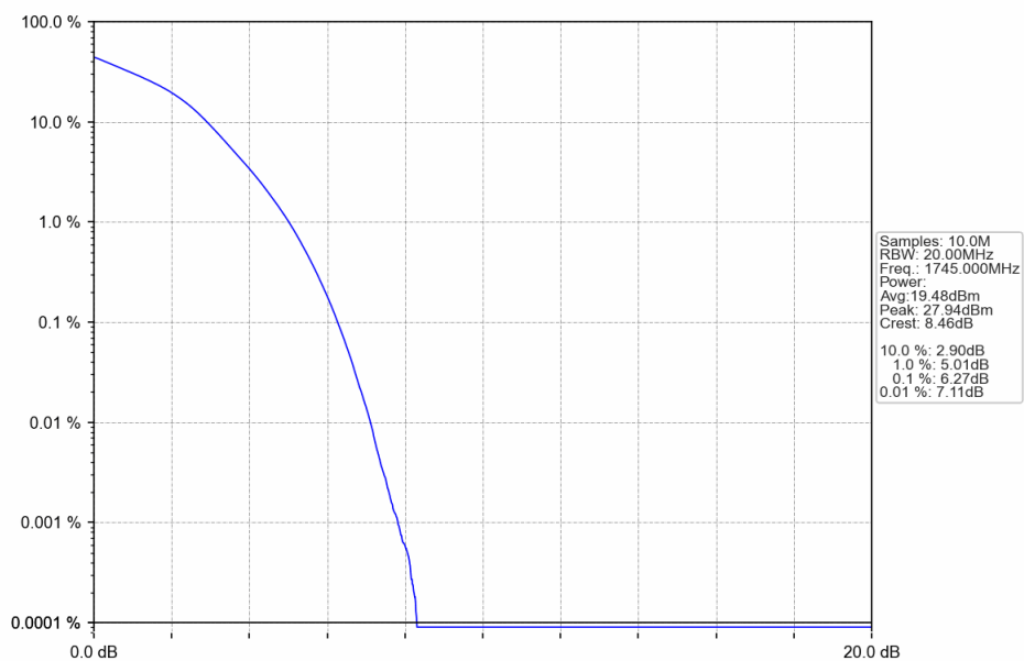
Band4_20MHz_16QAM_HCH_1745MHz_RB_100_0_NTNV
