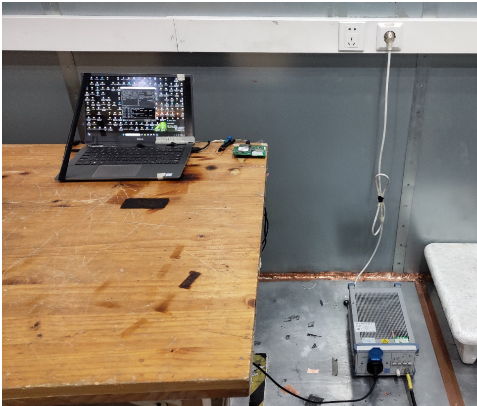
Picture 2 Conducted Emission Test Setup
