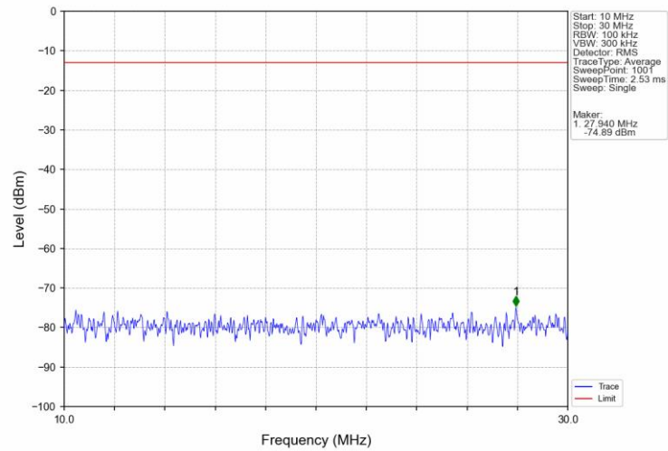
Band12_1.4MHz_16QAM_MCH_707.5MHz_RB_1_0_NTNV
