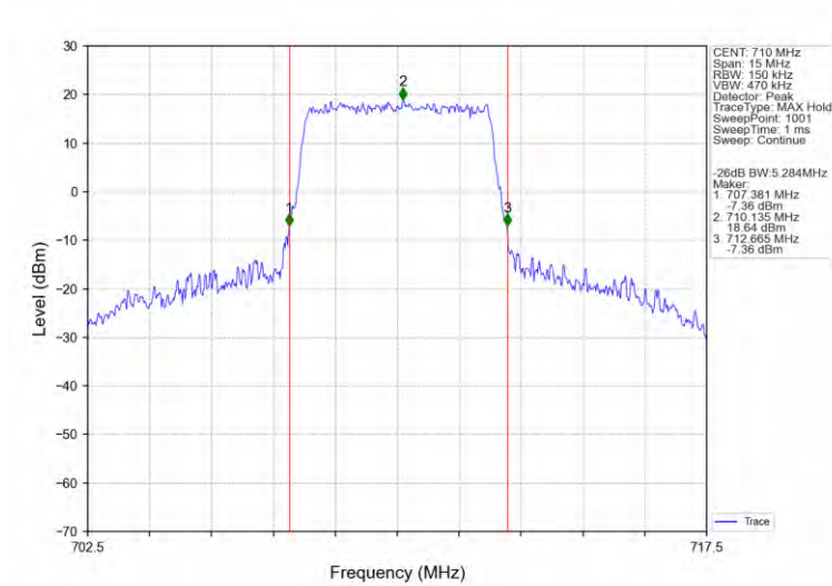
Band17_5MHz_QPSK_MCH_710MHz_RB_25_0_NTNV
