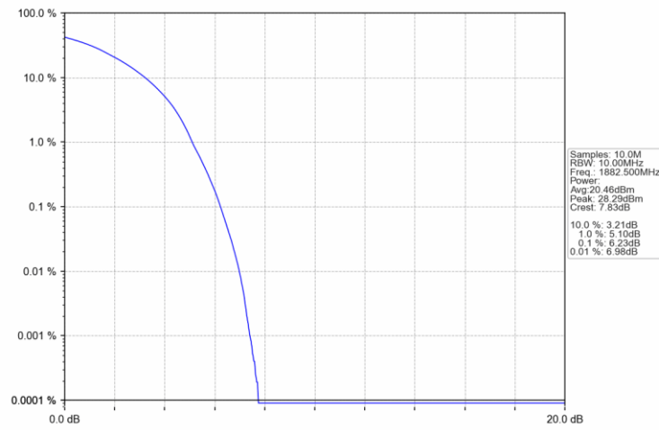
Band25_15MHz_16QAM_MCH_1882.5MHz_RB_75_0_NTNV
