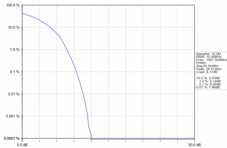
Band25_15MHz_16QAM_HCH_1907.5MHz_RB_75_0_NTNV
