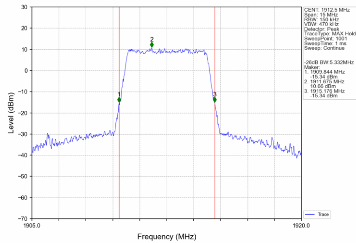
Band25_5MHz_16QAM_HCH_1912.5MHz_RB_25_0_NTNV
