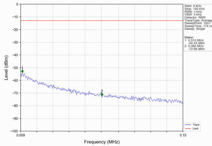
Band66_15MHz_16QAM_LCH_1717.5MHz_RB_1_0_NTNV
