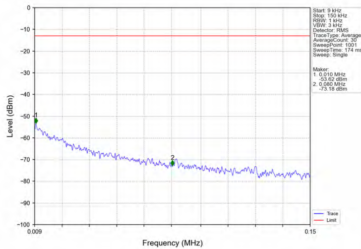
Band5_RMC_LCH_826.4MHz_12.2kbps RMC_NTNV
