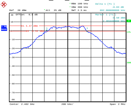
BLE_1M_Low_Channel
