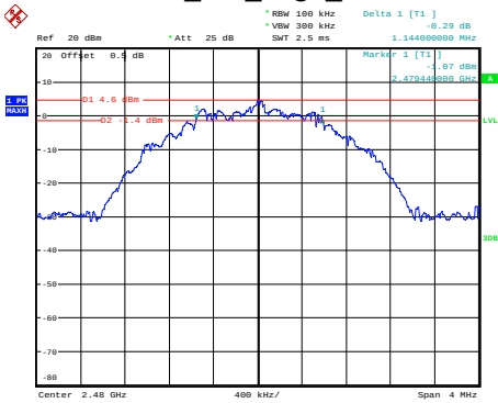
BLE_2M_High_Channel
