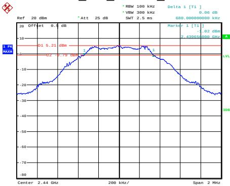
BLE_1M_Middle_Channel
