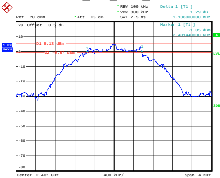
BLE_2M_Low_Channel
