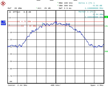
BLE_2M_Middle_Channel
