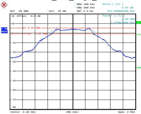
BLE_1M_High_Channel
