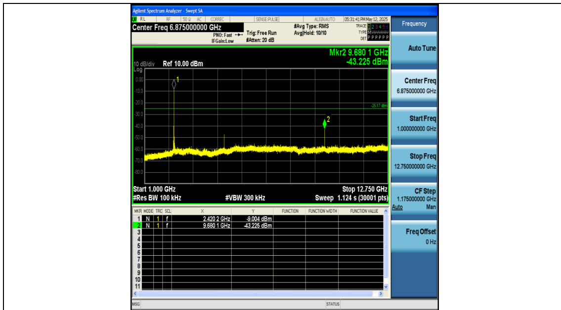
SRD-Ant1-2420-1000~12750-PASS
