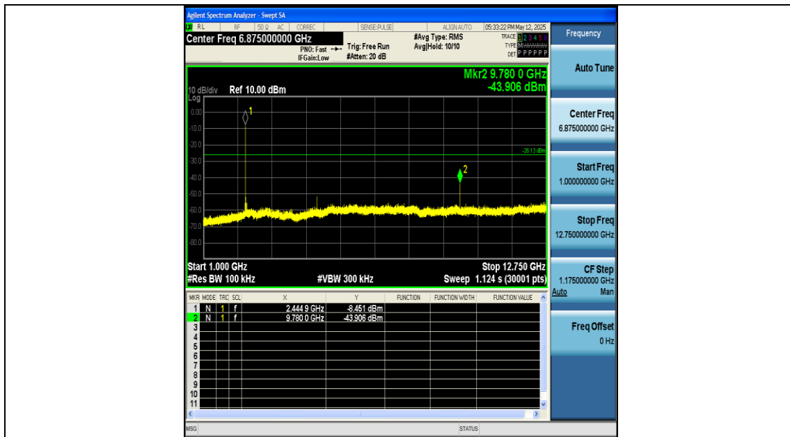
SRD-Ant1-2445-1000~12750-PASS
