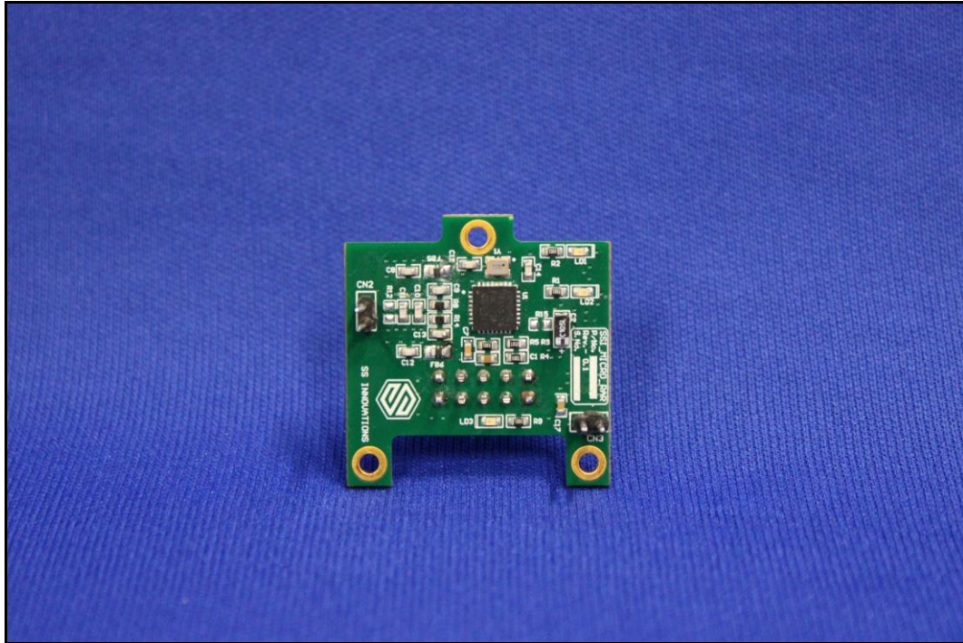
Photo 7: MODULE Rare View without Antenna
