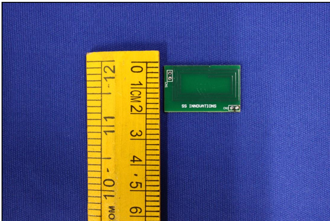
Photo 14: Antenna Dimensional View
