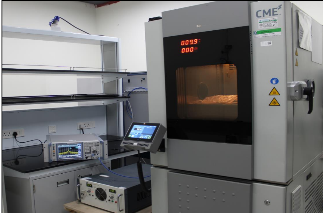
Conducted Test Setup: Extreme Temperature 10°C
