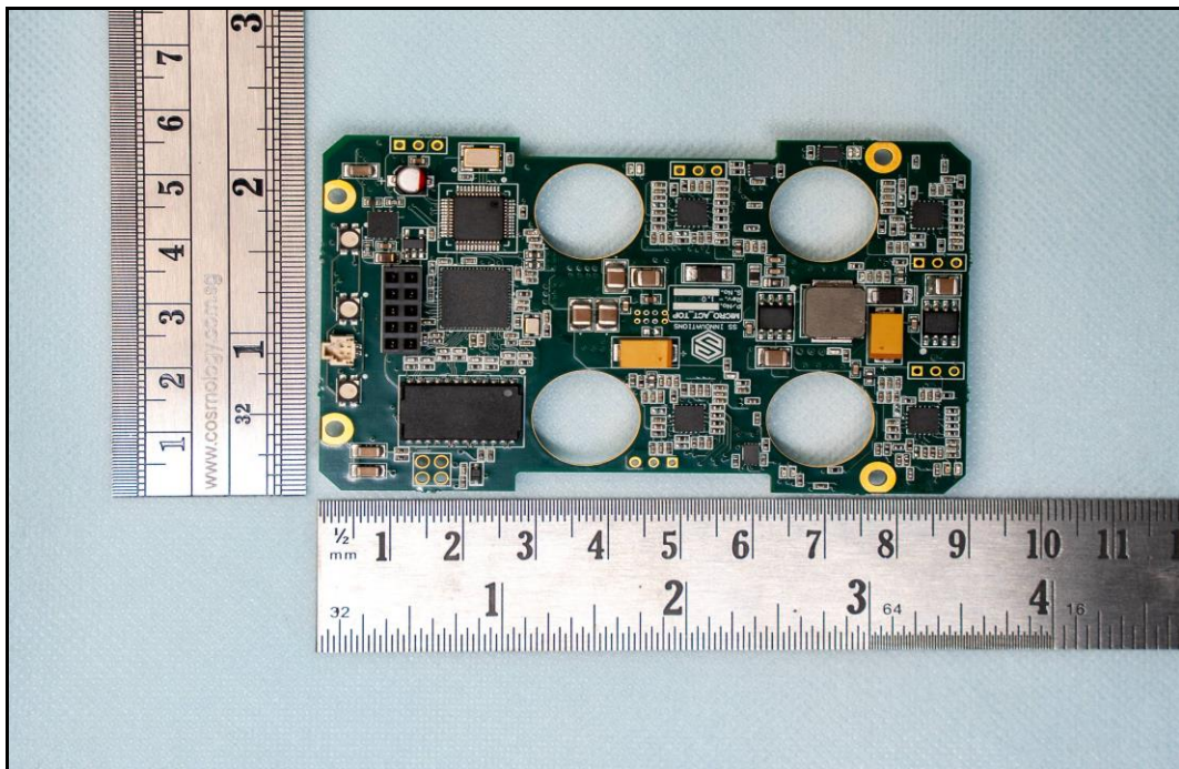
Photo 6: Actuator PCB Top View
