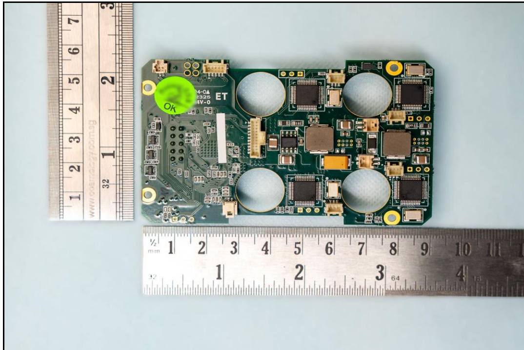
Photo 7: Actuator PCB Rare View
