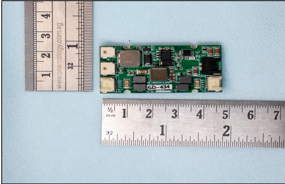
Photo 11: PCB2 Rare View
