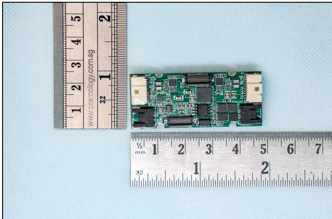
Photo 10: PCB2 Front View
