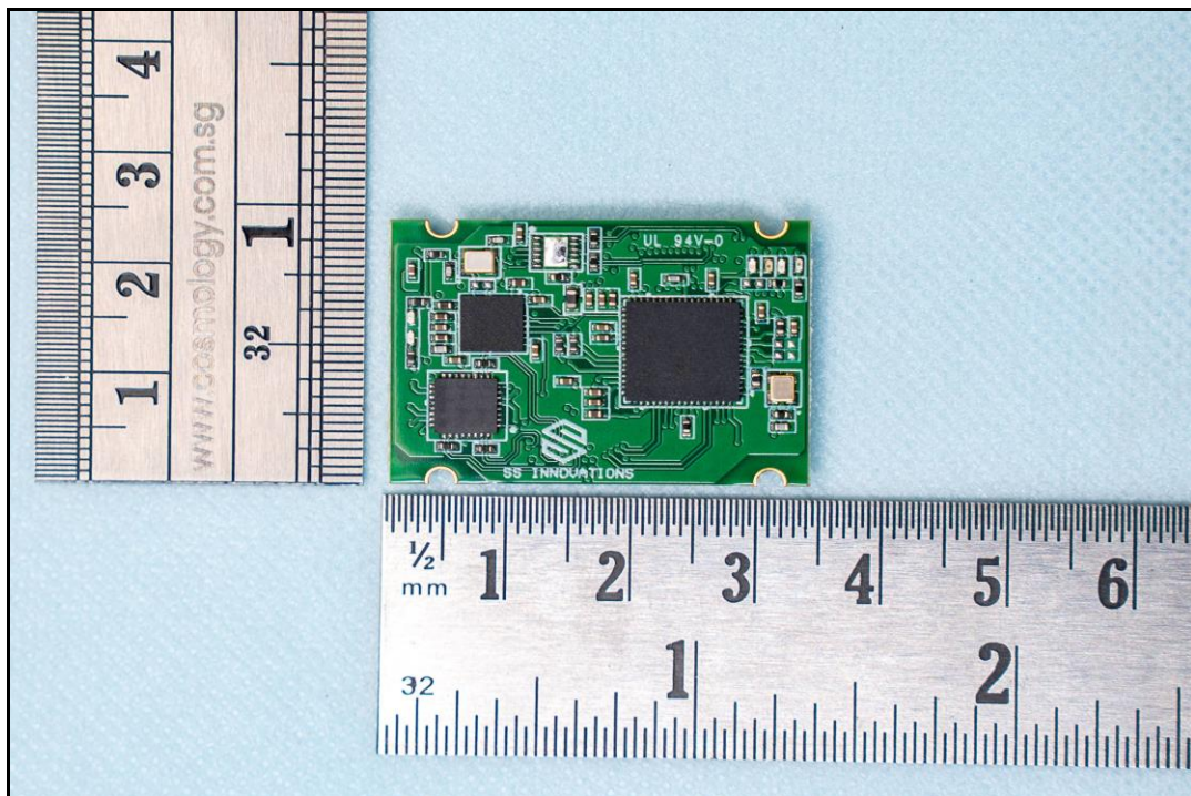
Photo 8: PCB1 Front View
