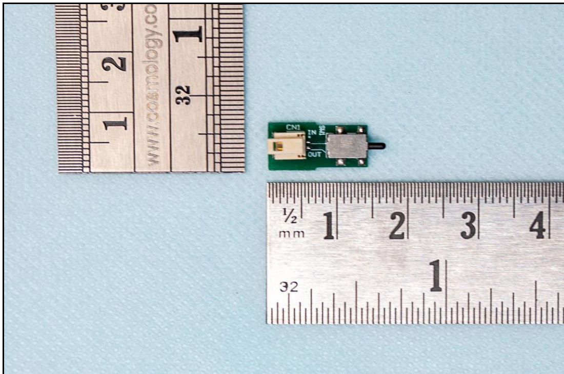
Photo 12: PCB3 Front View
