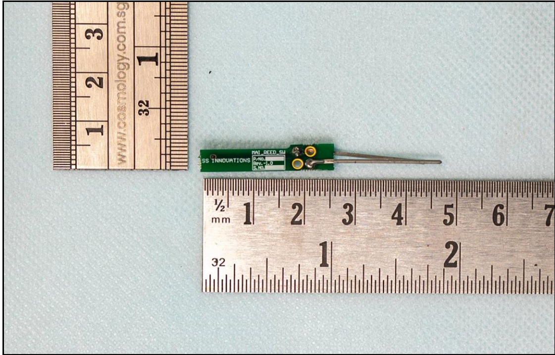
Photo 15: PCB4 Rare View
