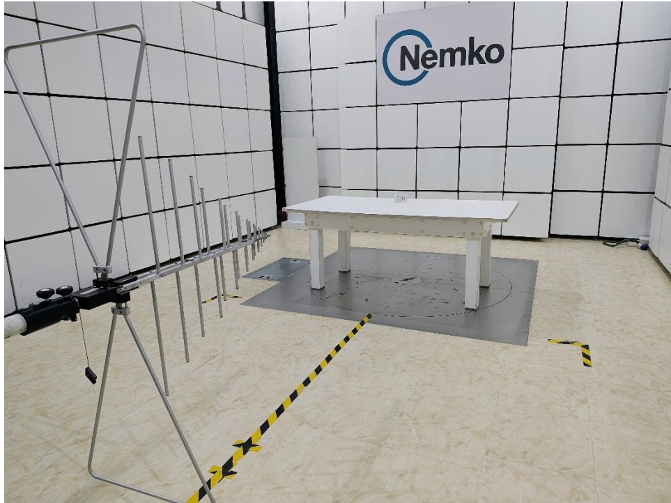
30MHz to 1GHz Test Setup
