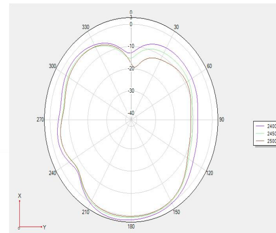
Theta 90 2D
