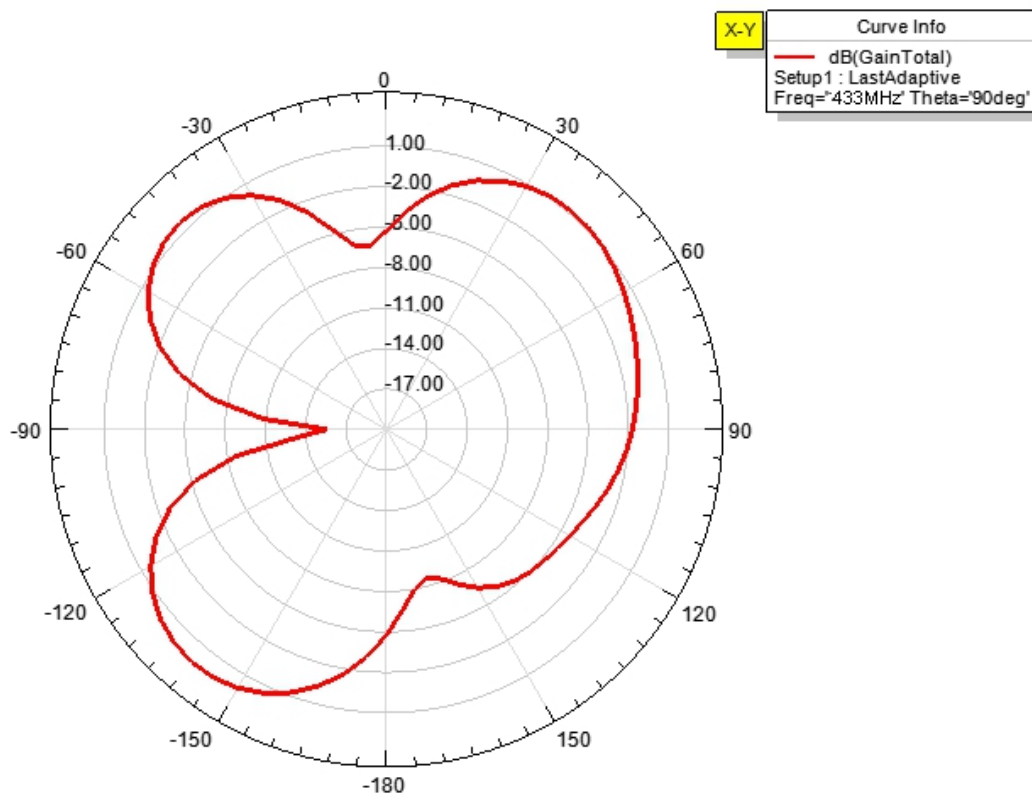
Radiation Pattern 2
