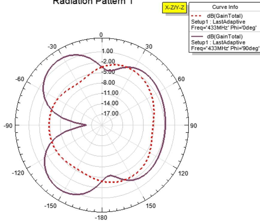
Radiation Pattern 1
