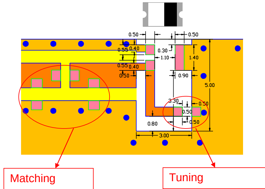
FootPrint (Unit : mm)
