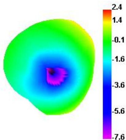
Bluetooth 39 TRP
