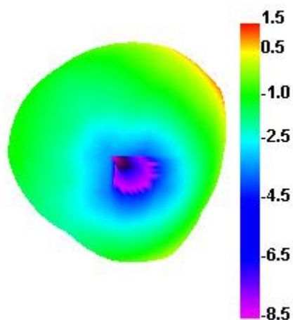
Bluetooth 78 TRP
