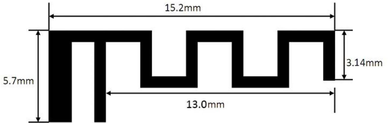
Antenna Dimensions
