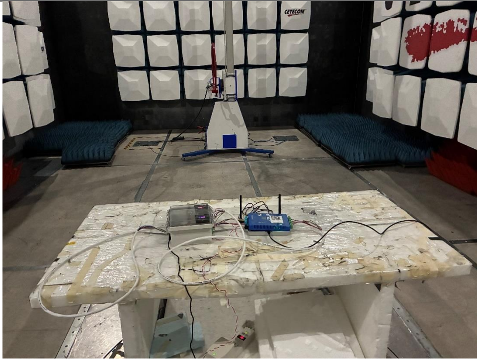
Radiated Emission 9kHz – 30MHz Front View
