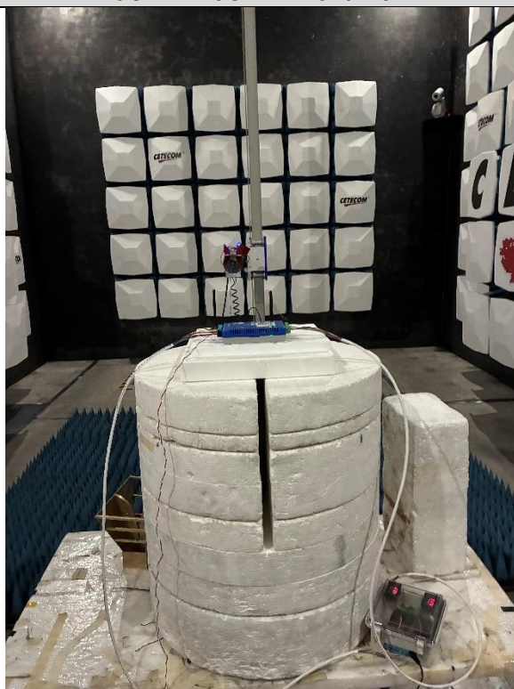
3GHz – 18GHz Front View
