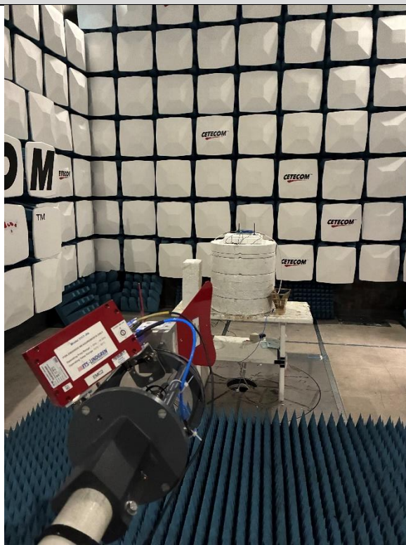
3GHz – 18GHz Rear View
