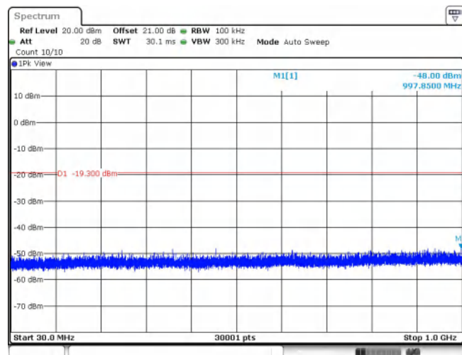
11G_Ant1_2462_0~Reference
