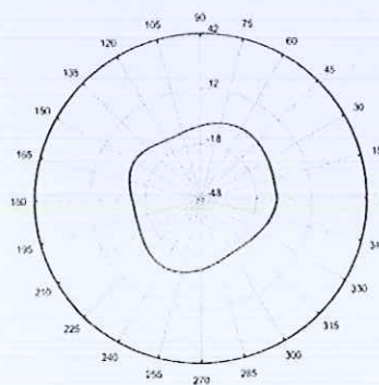
Total_Polar_E2_2.45GHz
