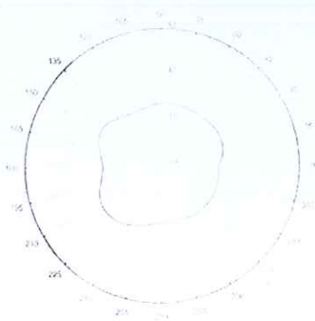
Total_Polar_E1_2.45GHz
