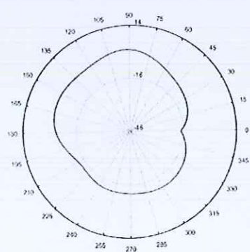
Total_Polar_E2_5.5GHz
