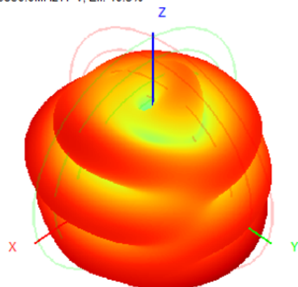
5850.0MHz H+V, Eff. 40.3%
