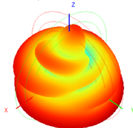
5550.0MHz H+V, Eff. 47.5%
