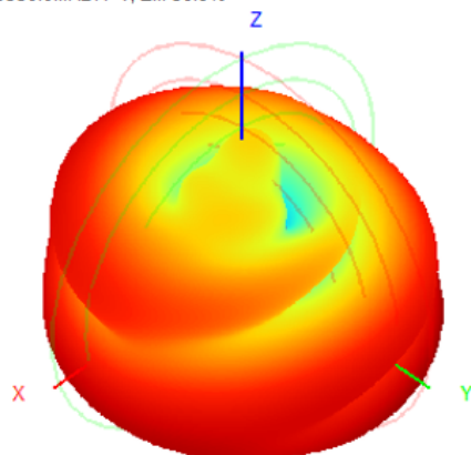
5350.0MHz H+V, Eff. 36.9%
