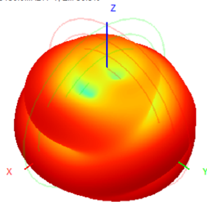
5150.0MHz H+V, Eff. 36.5%
