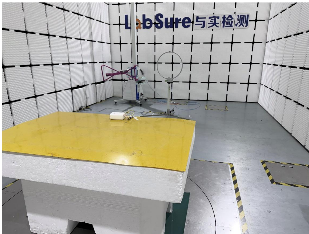
RSE Setup for 9kHz-30MHz
