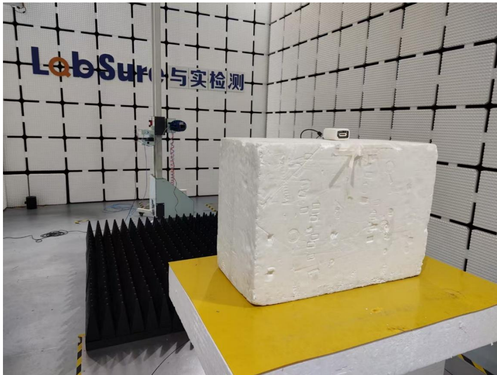
RSE Setup for 18GHz -26GHz
