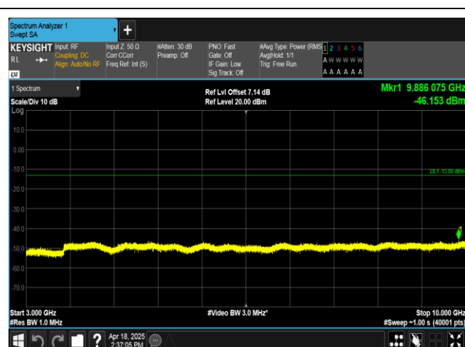
Band12-3MHz-OPSK-23025-1BB#14-3000~10000-PASS
