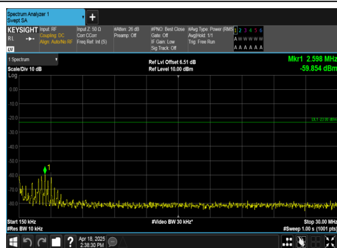
Band12-3MHz-OPSK-23025-15RB#0-0.15~30-PASS
