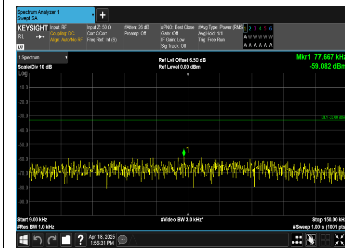
Band12-1.4MHz-16QAM-23095-6RB#0-0.009~0.15-PASS
