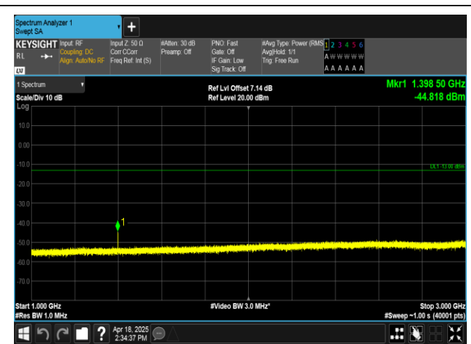
Band12-3MHz-QPSK-23025-1RB#0-1000~3000-PASS
