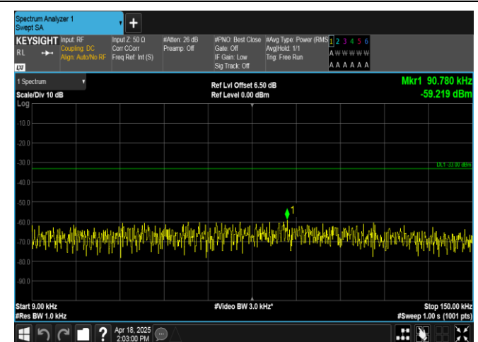
Band12-1.4MHz-16QAM-23173-6RB#0-0.009~0.15-PASS
