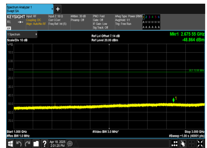
Band12-1.4MHz-16QAM-23173-1RB#5-1000~3000-PASS
