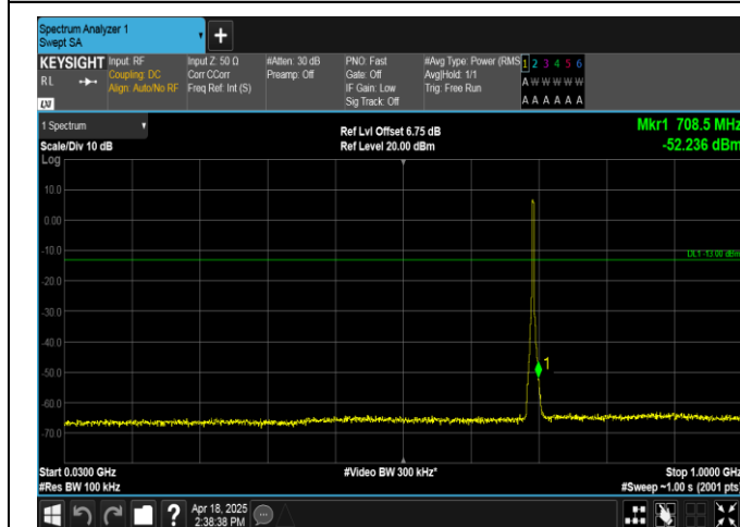
Band12-3MHz-QPSK-23025-15RB#0-30~1000-PASS
