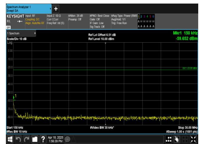
Band12-1.4MHz-16QAM-23095-6RB#0-0.15~30-PASS
