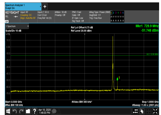
Band12-1.4MHz-16QAM-23017-1RB#0-30~1000-PASS
