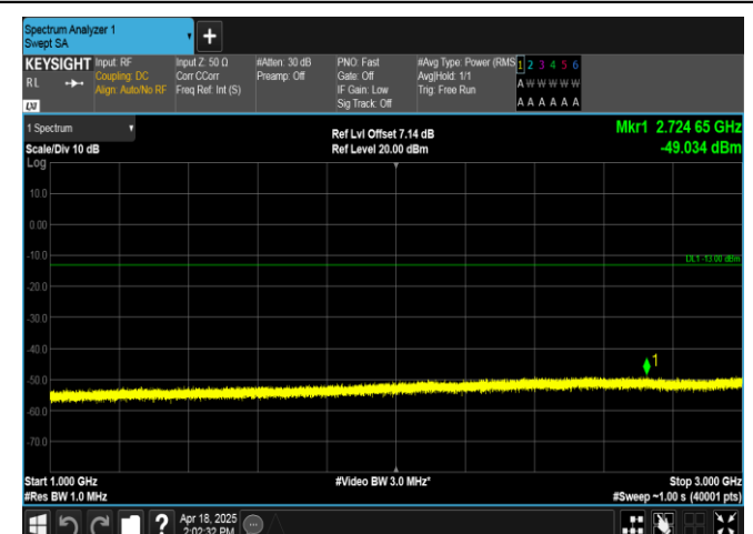
Band12-1.4MHz-QPSK-23173-6RB#0-1000~3000-PASS
