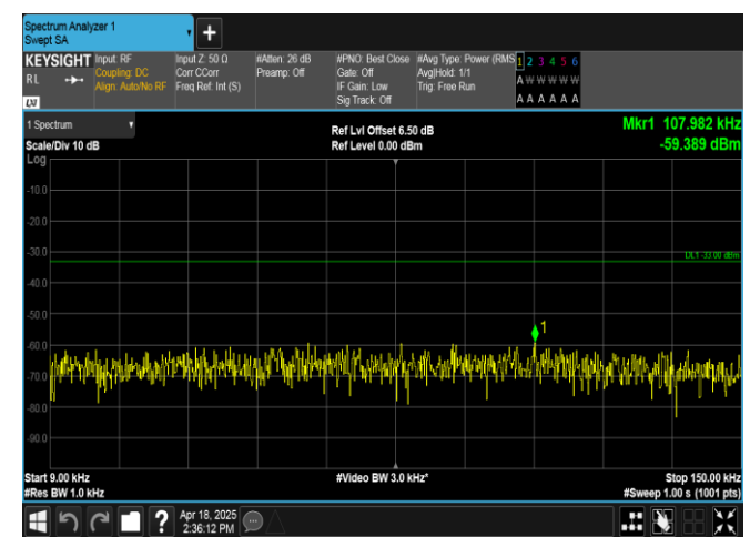
Band12-3MHz-QPSK-23025-1RB#14-0.009~0.15-PASS
