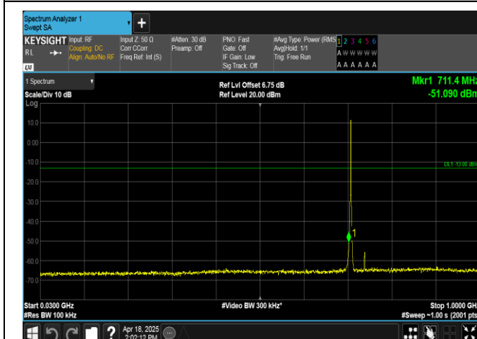
Band12-1.4MHz-QPSK-23173-6RB#0-30~1000-PASS
