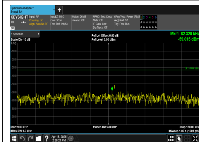
Band12-3MHz-OPSK-23025-15RB#0-0.009~0.15-PASS
