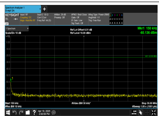
Band12-1.4MHz-16QAM-23173-1RB#5-0.15~30-PASS
