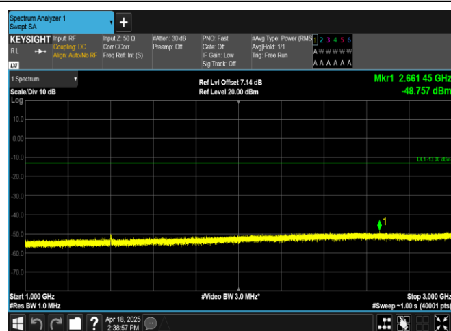
Band12-3MHz-QPSK-23025-15RB#0-1000~3000-PASS
