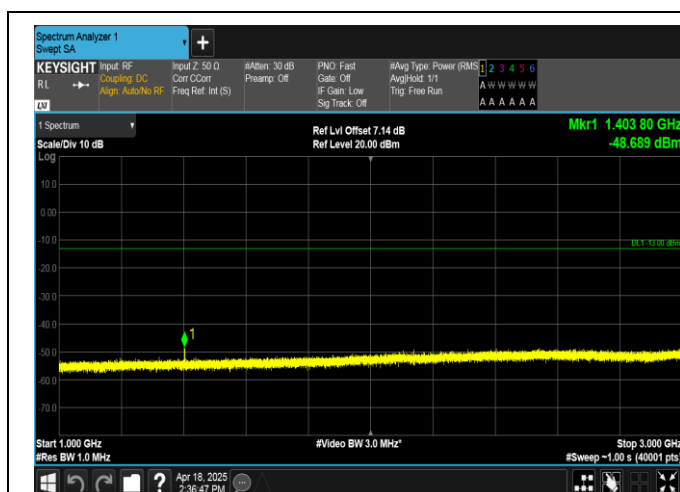
Band12-3MHz-OPSK-23025-1BB#14-1000~3000-PASS
