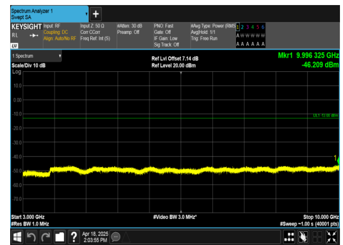
Band12-1.4MHz-16QAM-23173-6RB#0-3000~10000-PASS
