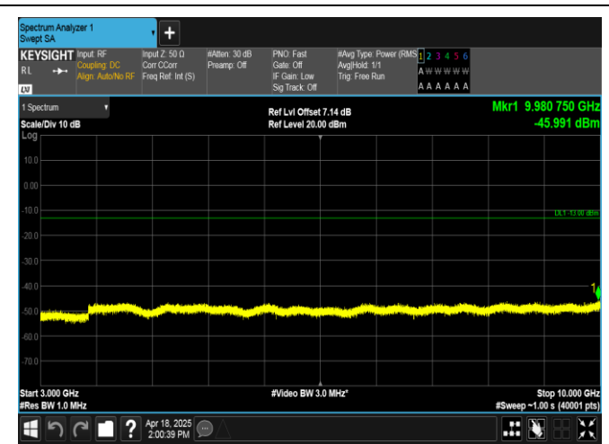
Band12-1.4MHz-QPSK-23173-1RB#5-3000~10000-PASS
