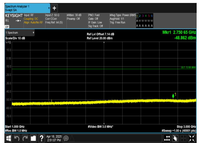
Band12-3MHz-16QAM-23165-1RB#14-1000~3000-PASS
