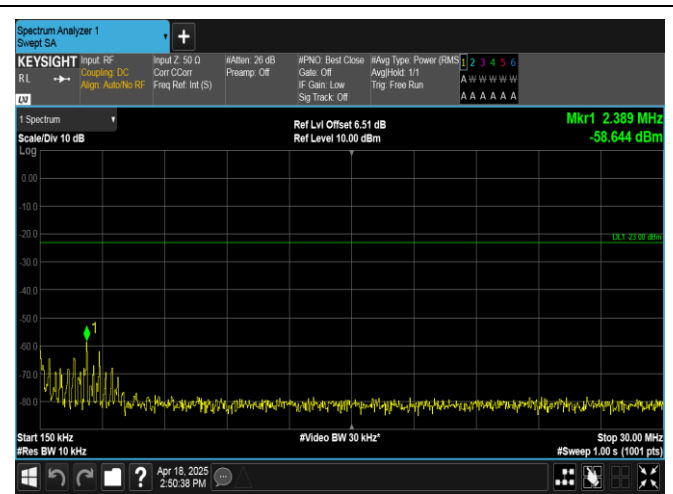
Band12-3MHz-16QAM-23165-1RB#14-0.15~30-PASS
