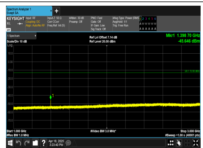
Band12-5MHz-QPSK-23035-1RB#0-1000~3000-PASS
