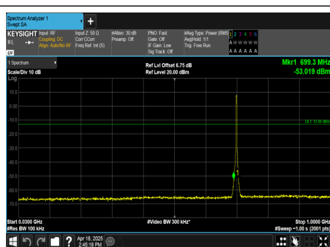
Band12-3MHz-OPSK-23095-15RB#0-30~1000-PASS
