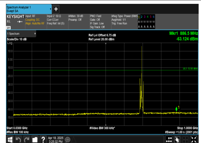
Band12-5MHz-QPSK-23035-1RB#24-30~1000-PASS
