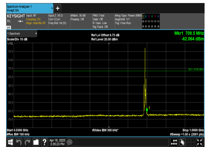
Band12-3MHz-16QAM-23025-1RB#0-30~1000-PASS
