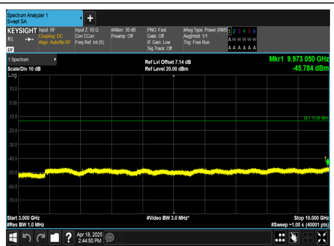
Band12-3MHz-16QAM-23095-1RB#14-3000~10000-PASS
