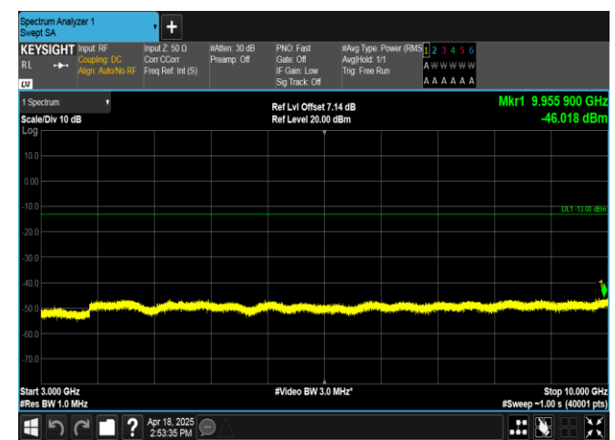
Band12-3MHz-16QAM-23165-15RB#0-3000~10000-PASS
