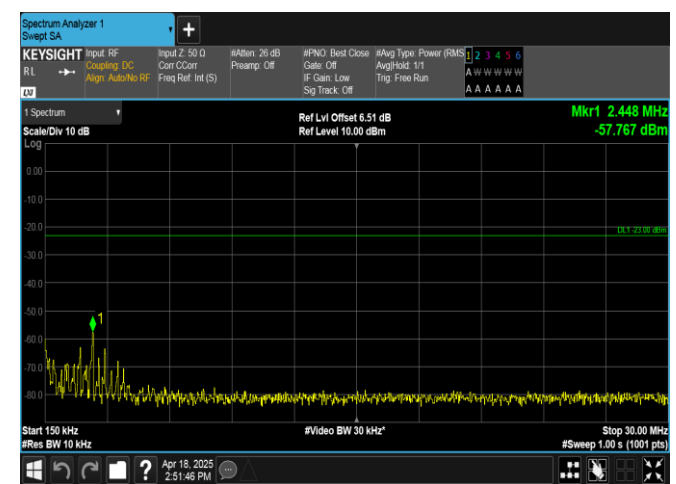
Band12-3MHz-QPSK-23165-15RB#0-0.15~30-PASS
