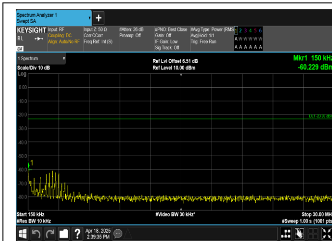
Band12-3MHz-16QAM-23025-15RB#0-0.15~30-PASS
