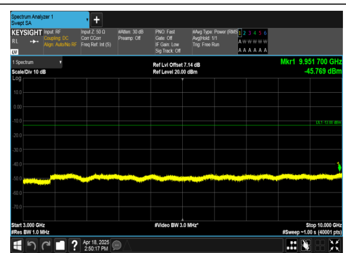
Band12-3MHz-QPSK-23165-1RB#14-3000~10000-PASS
