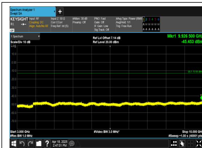
Band12-3MHz-16QAM-23095-15RB#0-3000~10000-PASS
