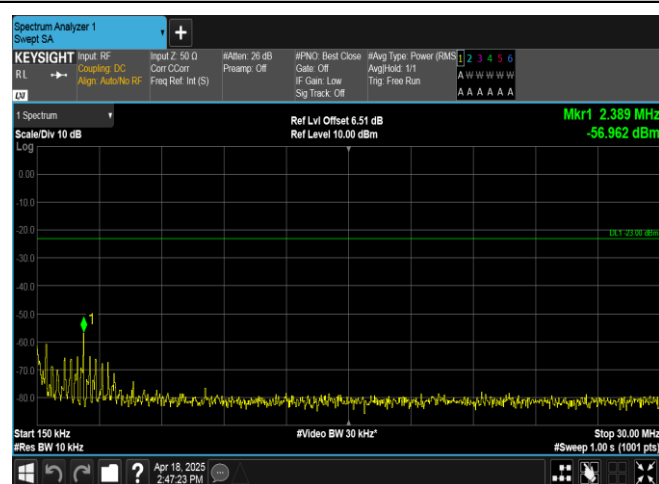
Band12-3MHz-QPSK-23165-1RB#0-0.15~30-PASS
