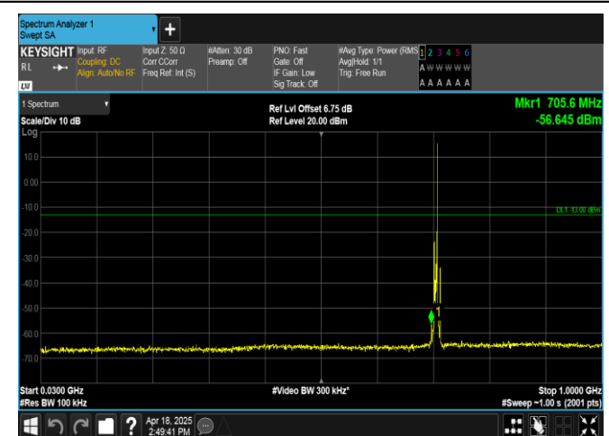
Band12-3MHz-QPSK-23165-1RB#14-30~1000-PASS
