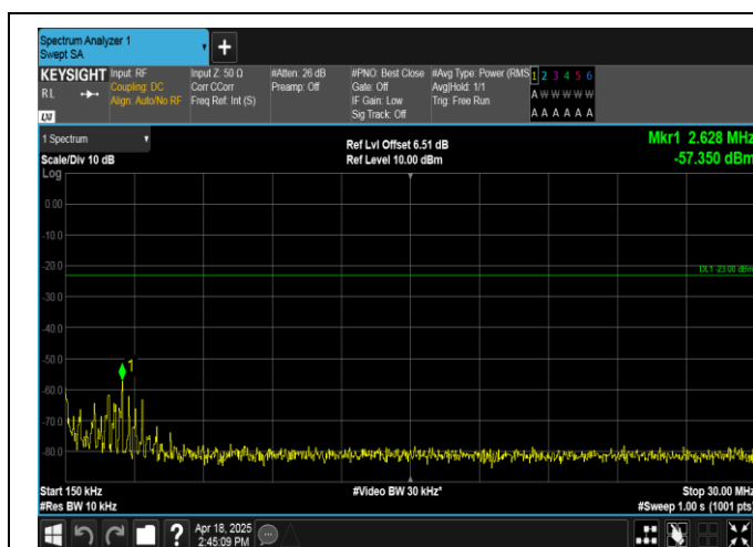
Band12-3MHz-OPSK-23095-15RB#0-0.15~30-PASS
