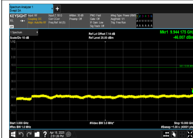
Band12-3MHz-16QAM-23165-1RB#14-3000~10000-PASS
