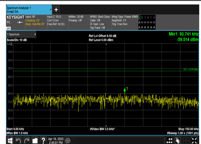
Band12-3MHz-QPSK-23095-15RB#0-0.009~0.15-PASS
