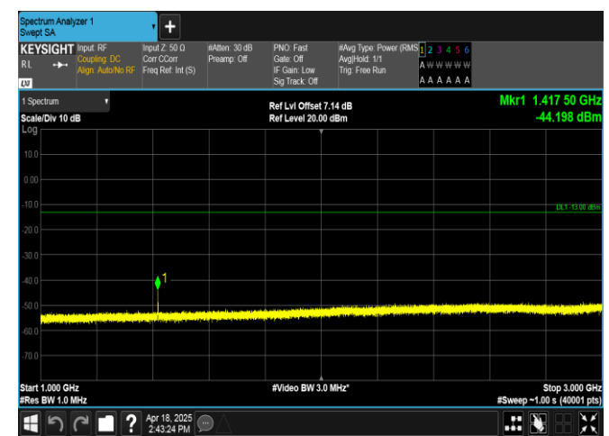
Band12-3MHz-QPSK-23095-1RB#14-1000~3000-PASS
