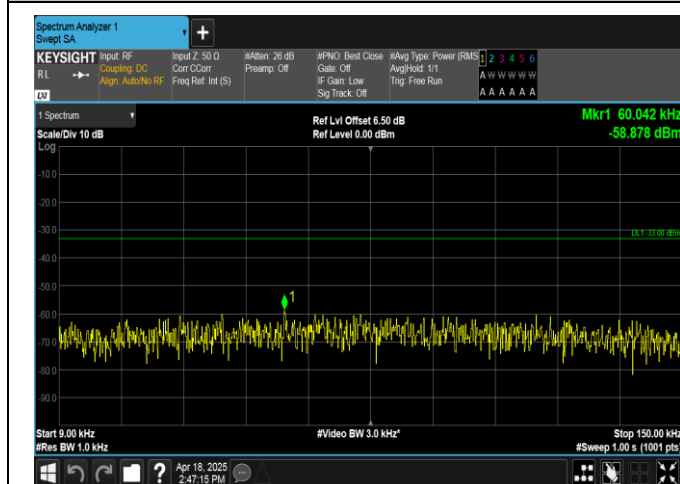
Band12-3MHz-QPSK-23165-1RB#0-0.009~0.15-PASS
