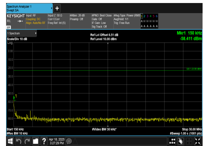
Band12-5MHz-QPSK-23035-25RB#0-0.15~30-PASS
