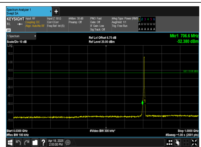
Band12-3MHz-16QAM-23165-15RB#0-30~1000-PASS
