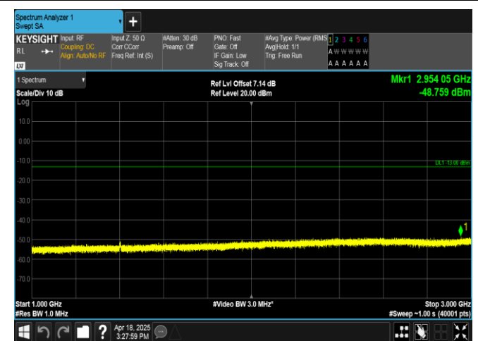
Band12-5MHz-QPSK-23035-25RB#0-1000~3000-PASS
