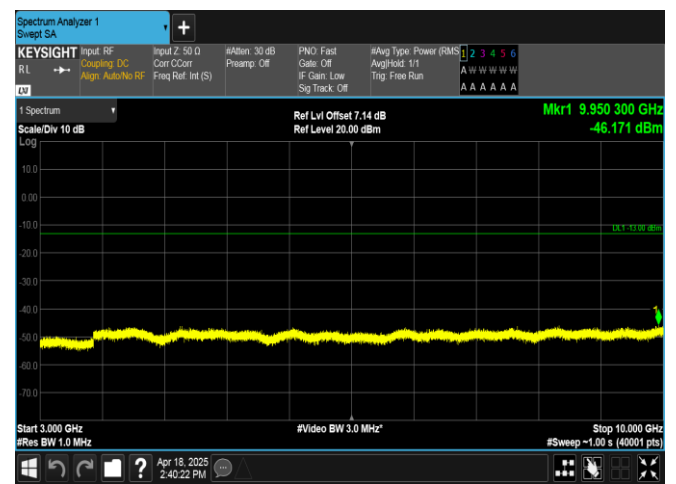
Band12-3MHz-16QAM-23025-15RB#0-3000~10000-PASS
