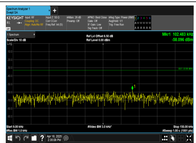
Band12-3MHz-16QAM-23025-1RB#0-0.009~0.15-PASS
