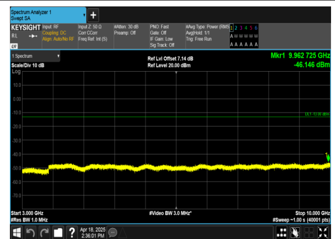
Band12-3MHz-16QAM-23025-1RB#0-3000~10000-PASS
