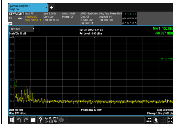
Band12-3MHz-16QAM-23165-1RB#0-0.15~30-PASS
