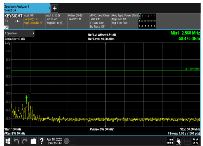
Band12-3MHz-16QAM-23095-15RB#0-0.15~30-PASS
