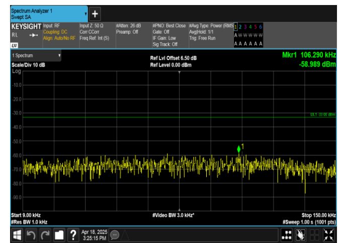
Band12-5MHz-QPSK-23035-1RB#24-0.009~0.15-PASS
