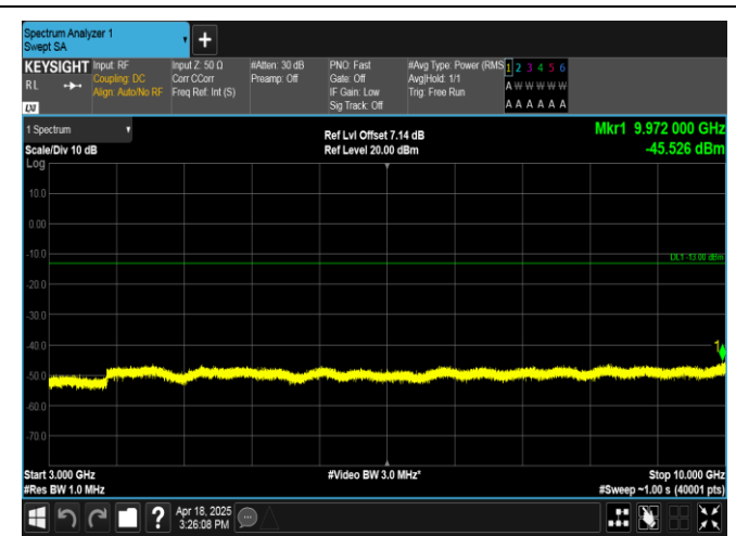
Band12-5MHz-QPSK-23035-1RB#24-3000~10000-PASS
