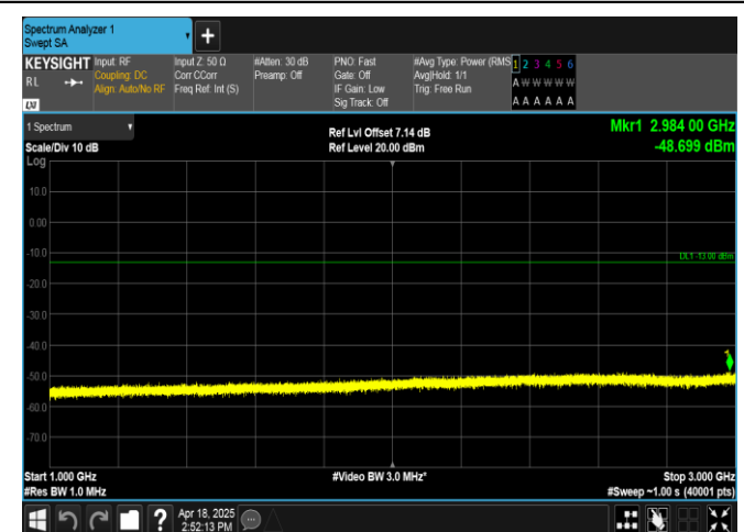
Band12-3MHz-QPSK-23165-15RB#0-1000~3000-PASS
