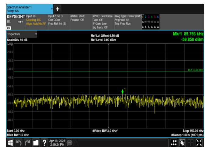
Band12-3MHz-QPSK-23165-1RB#14-0.009~0.15-PASS
