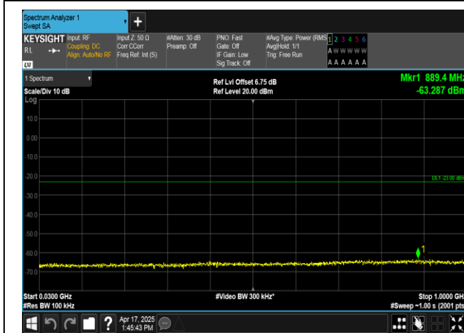
Band2-10MHz-QPSK-18650-1RB#0-30~1000-PASS
