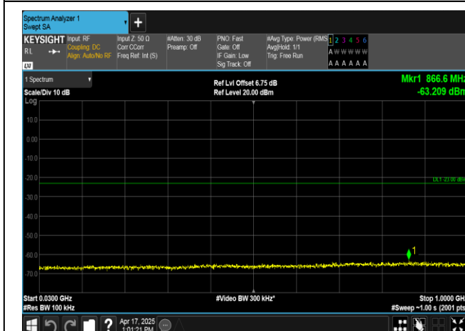
Band2-5MHz-16QAM-19175-1RB#24-30~1000-PASS
