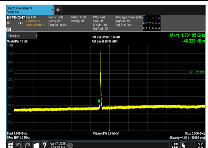
Band2-5MHz-16QAM-19175-1RB#24-1000~3000-PASS
