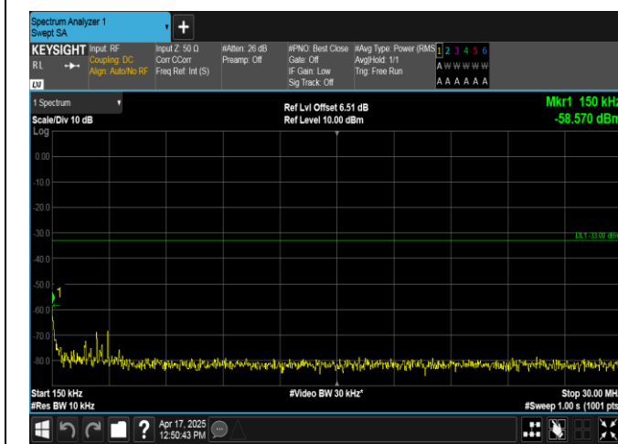
Band2-5MHz-16QAM-18625-25RB#0-0.15~30-PASS
