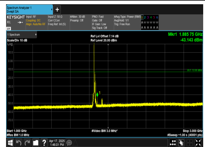
Band2-10MHz-QPSK-18650-1RB#0-1000~3000-PASS
