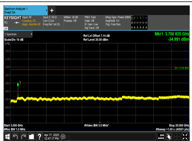
Band2-5MHz-16QAM-18625-1RB#0-3000~20000-PASS
