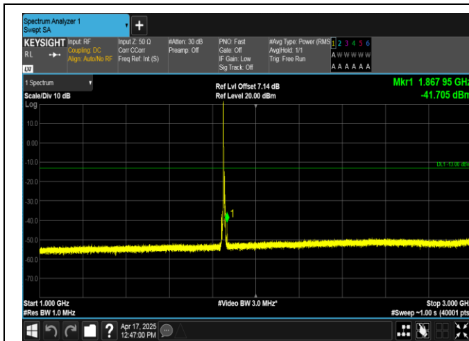
Band2-5MHz-16QAM-18625-1RB#0-1000~3000-PASS
