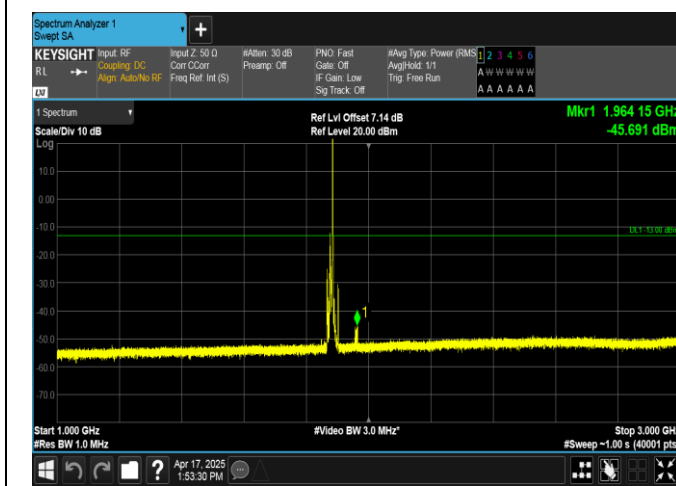
Band2-10MHz-16QAM-18900-1RB#49-1000~3000-PASS
