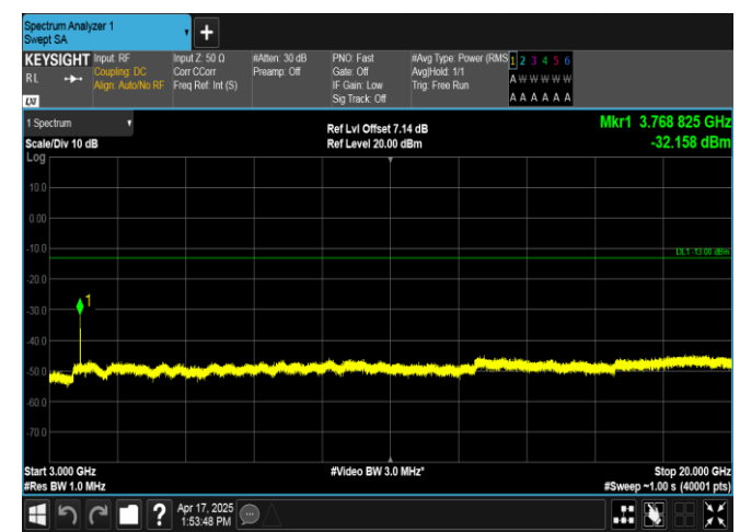
Band2-10MHz-16QAM-18900-1RB#49-3000~20000-PASS
