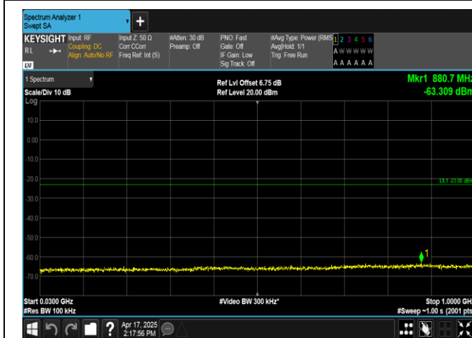
Band2-15MHz-16QAM-18675-1RB#74-30~1000-PASS
