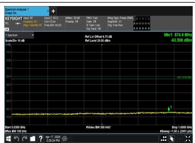
Band2-15MHz-QPSK-19125-1RB#74-30~1000-PASS
