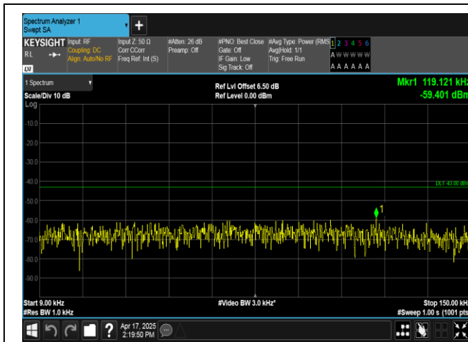
Band2-15MHz-16QAM-18900-1RB#0-0.009~0.15-PASS
