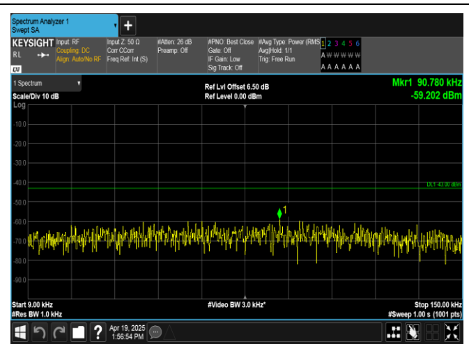
Band2-15MHz-QPSK-18900-75RB#0-0.009~0.15-PASS
