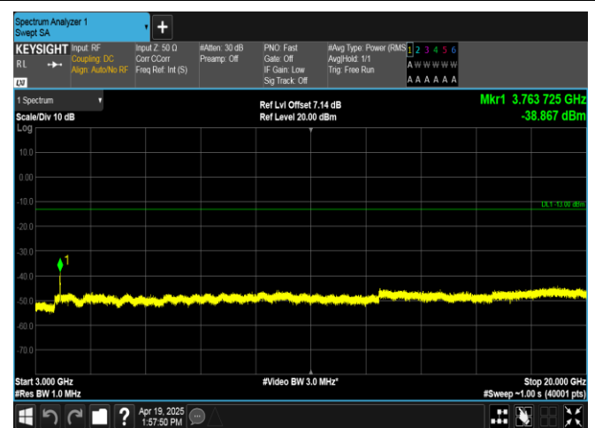
Band2-15MHz-QPSK-18900-75RB#0-3000~20000-PASS
