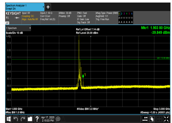
Band2-15MHz-QPSK-18675-1RB#0-1000~3000-PASS
