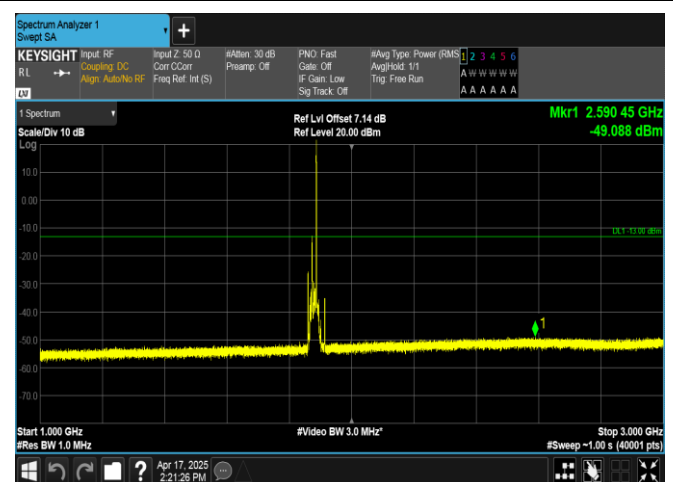
Band2-15MHz-QPSK-18900-1RB#74-1000~3000-PASS
