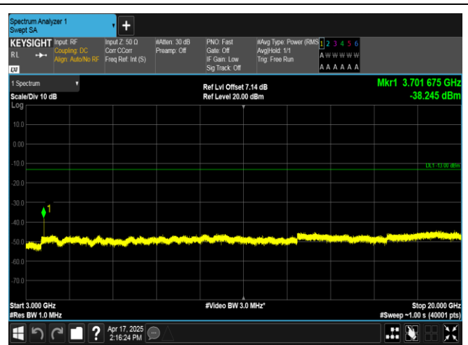
Band2-15MHz-16QAM-18675-1RB#0-3000~20000-PASS
