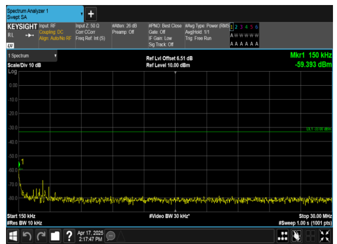
Band2-15MHz-16QAM-18675-1RB#74-0.15~30-PASS
