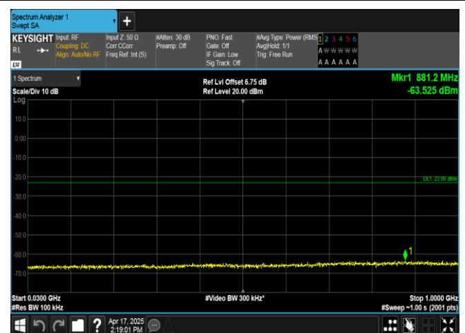
Band2-15MHz-QPSK-18900-1RB#0-30~1000-PASS
