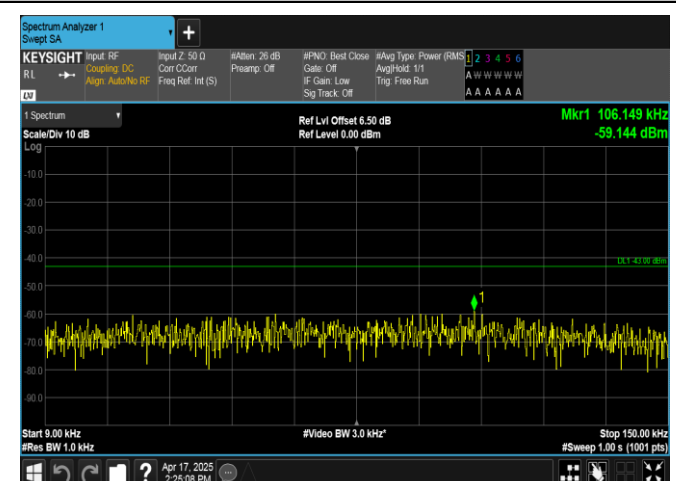
Band2-15MHz-QPSK-19125-1RB#74-0.009~0.15-PASS
