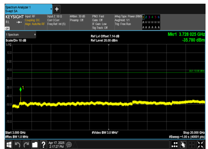
Band2-15MHz-QPSK-18675-1RB#74-3000~20000-PASS
