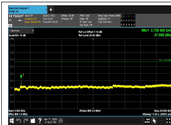
Band2-15MHz-16QAM-18675-1RB#74-3000~20000-PASS
