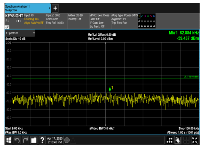
Band2-15MHz-QPSK-18900-1RB#0-0.009~0.15-PASS
