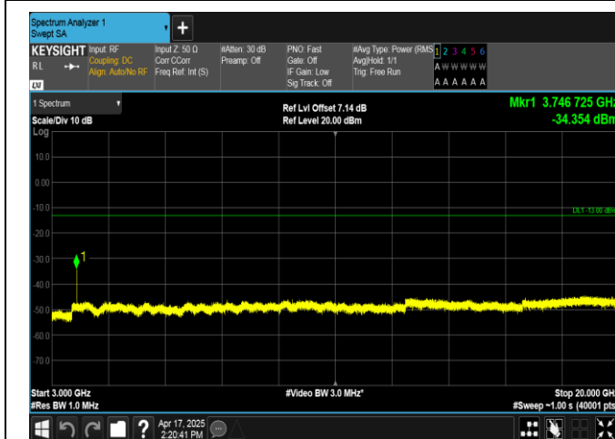
Band2-15MHz-16QAM-18900-1RB#0-3000~20000-PASS
