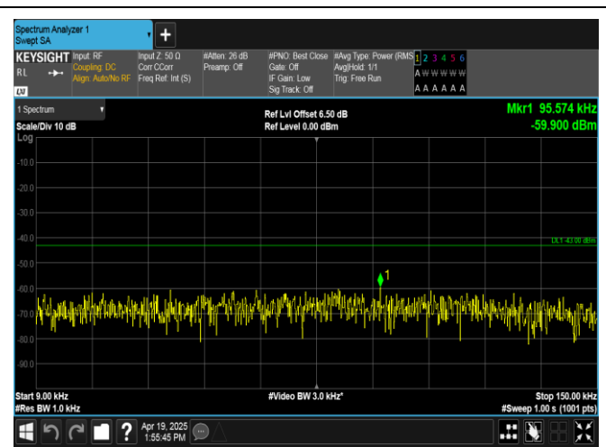
Band2-15MHz-16QAM-18675-75RB#0-0.009~0.15-PASS
