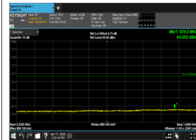
Band2-15MHz-QPSK-19125-1RB#0-30~1000-PASS
