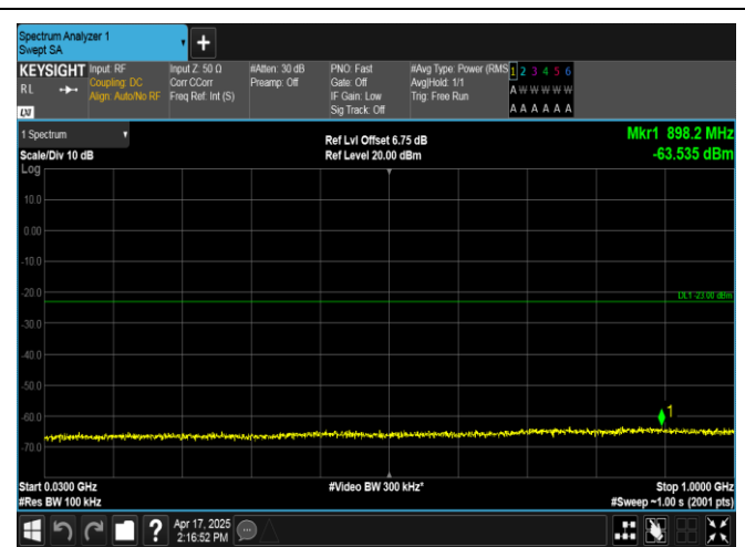
Band2-15MHz-QPSK-18675-1RB#74-30~1000-PASS
