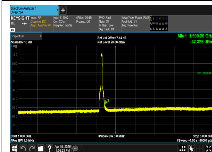
Band2-15MHz-16QAM-18675-75RB#0-1000~3000-PASS
