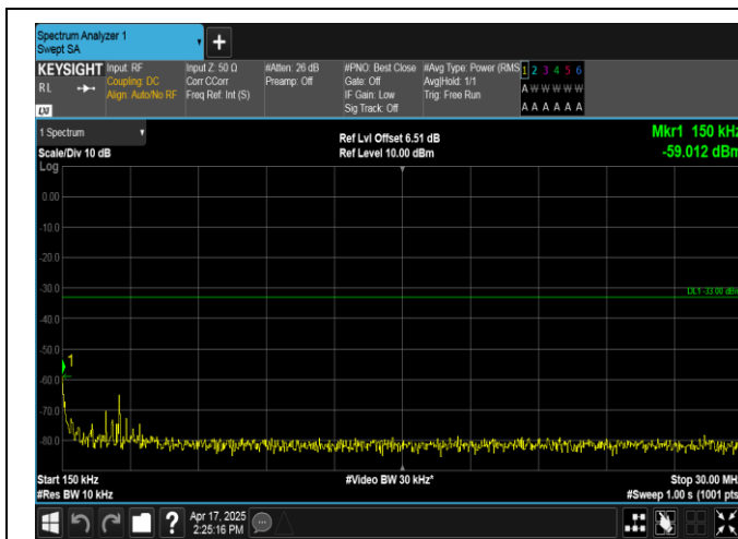
Band2-15MHz-QPSK-19125-1RB#74-0.15~30-PASS
