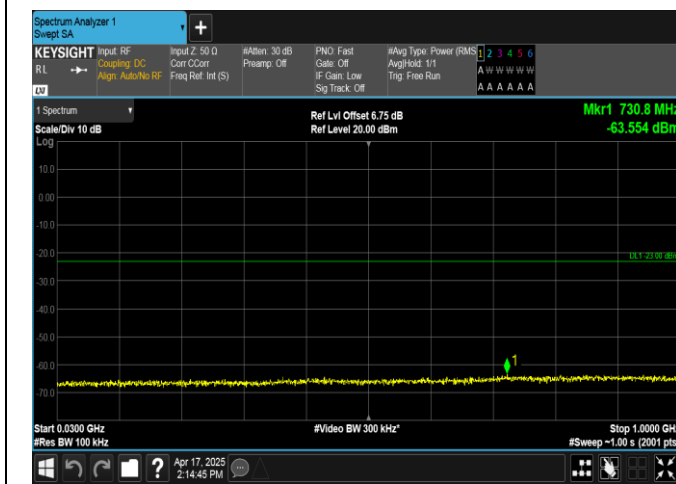
Band2-15MHz-QPSK-18675-1RB#0-30~1000-PASS
