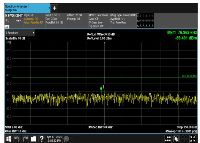
Band2-15MHz-16QAM-18675-1RB#0-0.009~0.15-PASS
