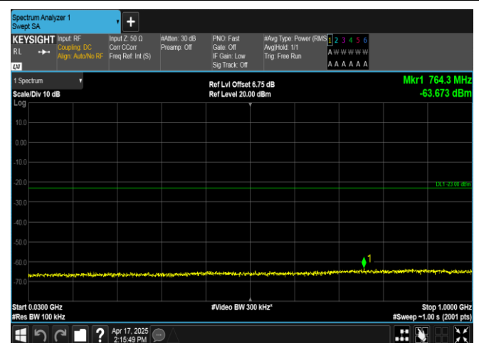
Band2-15MHz-16QAM-18675-1RB#0-30~1000-PASS
