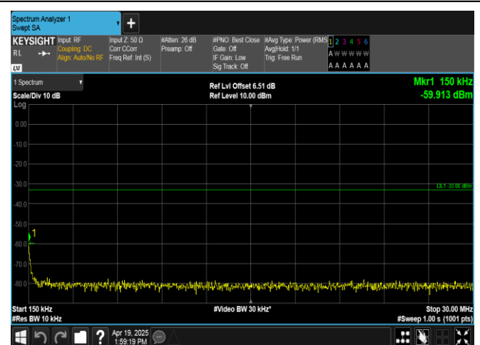
Band2-15MHz-QPSK-19125-75RB#0-0.15~30-PASS
