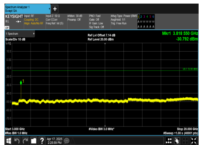
Band2-15MHz-QPSK-19125-1RB#74-3000~20000-PASS
