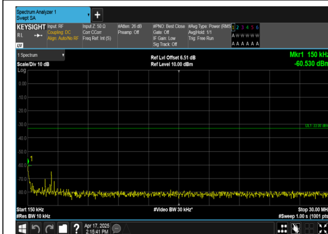
Band2-15MHz-16QAM-18675-1RB#0-0.15~30-PASS
