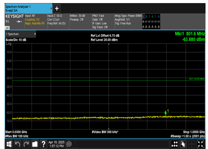
Band2-15MHz-QPSK-18900-75RB#0-30~1000-PASS
