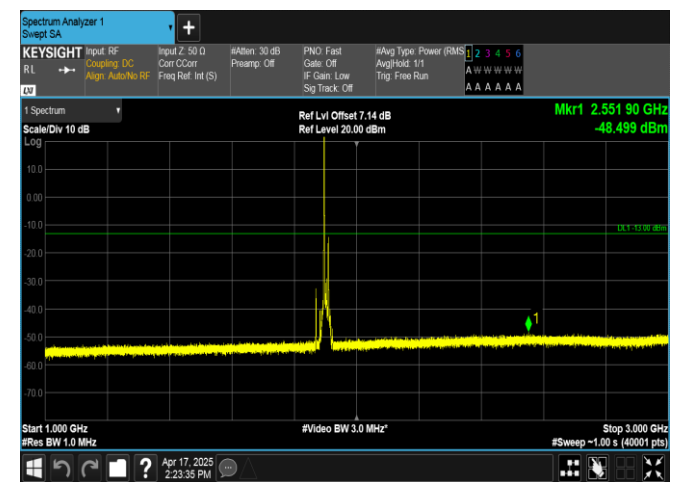
Band2-15MHz-QPSK-19125-1RB#0-1000~3000-PASS
