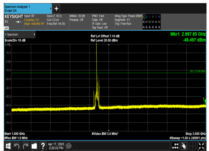
Band2-15MHz-16QAM-18900-1RB#0-1000~3000-PASS
