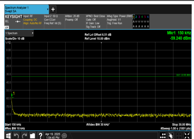
Band2-15MHz-QPSK-18675-75RB#0-0.15~30-PASS
