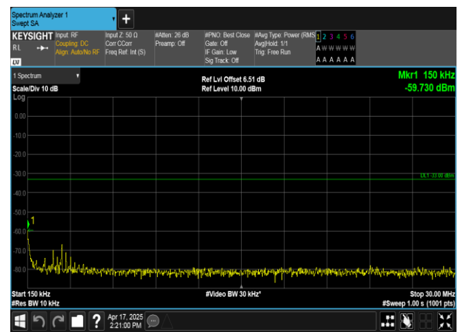
Band2-15MHz-QPSK-18900-1RB#74-0.15~30-PASS
