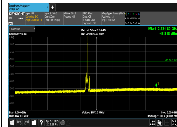
Band2-15MHz-16QAM-18900-1RB#74-1000~3000-PASS
