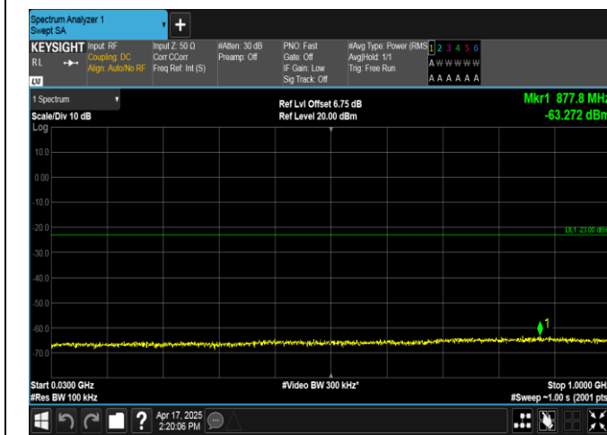
Band2-15MHz-16QAM-18900-1RB#0-30~1000-PASS
