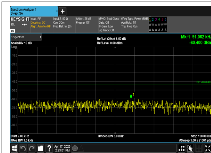
Band2-15MHz-QPSK-19125-1RB#0-0.009~0.15-PASS
