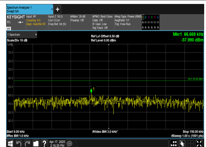
Band2-15MHz-QPSK-18675-1RB#74-0.009~0.15-PASS
