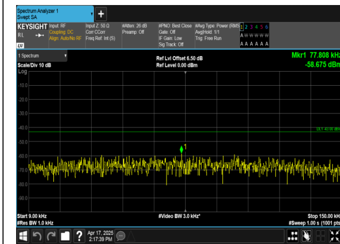
Band2-15MHz-16QAM-18675-1RB#74-0.009~0.15-PASS
