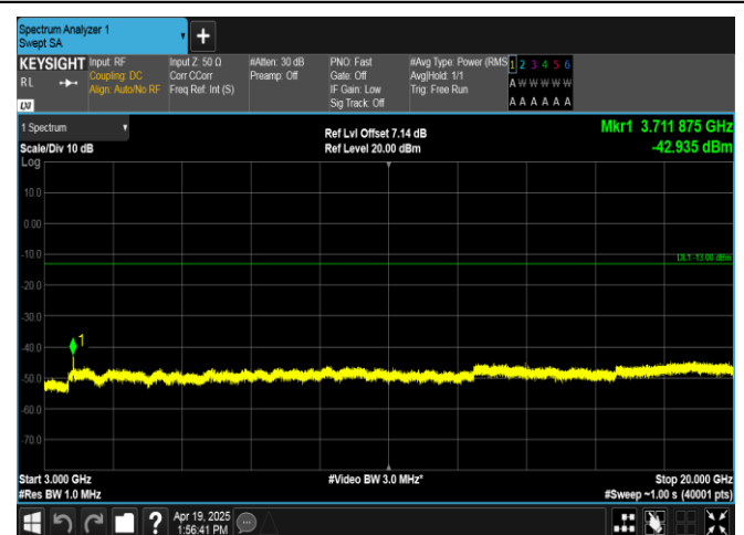
Band2-15MHz-16QAM-18675-75RB#0-3000~20000-PASS
