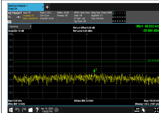
Band2-15MHz-16QAM-18900-75RB#0-0.009~0.15-PASS
