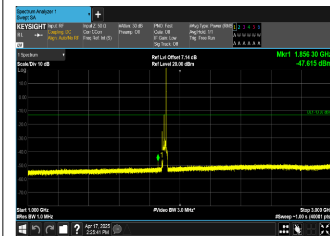
Band2-15MHz-QPSK-19125-1RB#74-1000~3000-PASS
