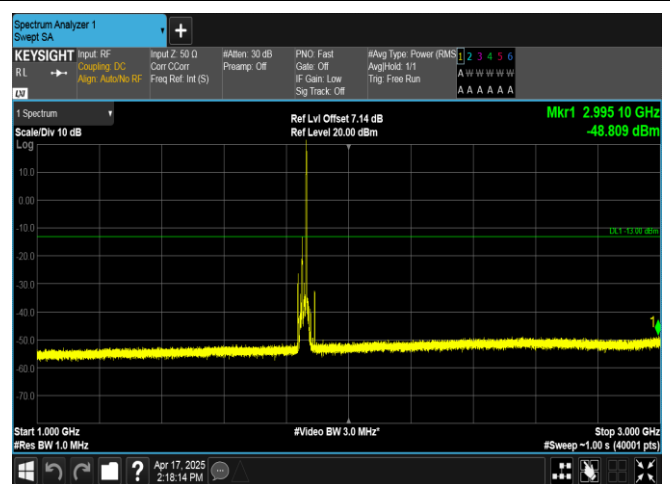
Band2-15MHz-16QAM-18675-1RB#74-1000~3000-PASS
