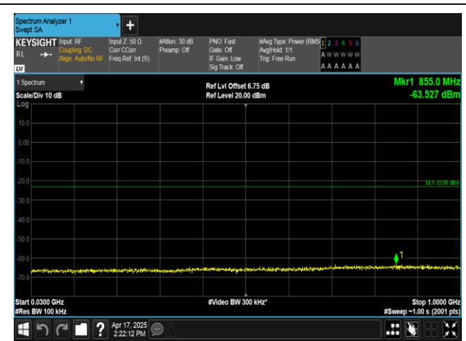
Band2-15MHz-16QAM-18900-1RB#74-30~1000-PASS
