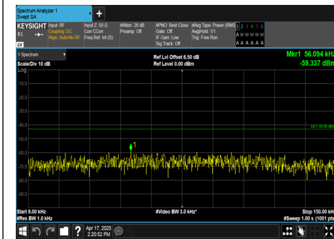
Band2-15MHz-QPSK-18900-1RB#74-0.009~0.15-PASS
