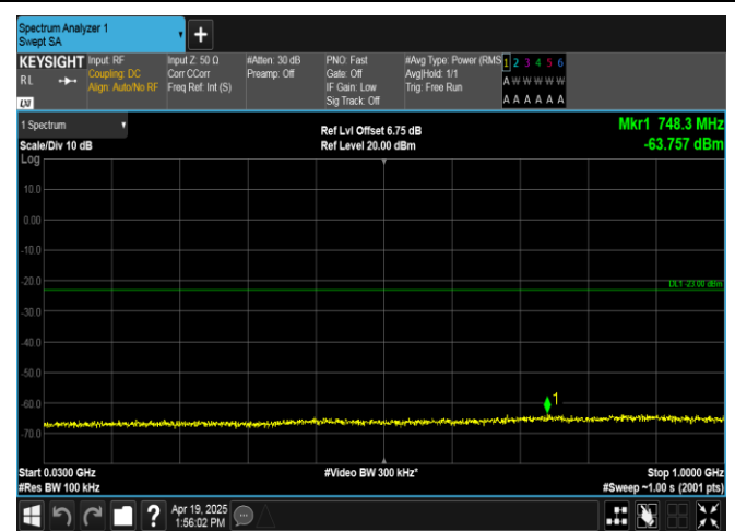
Band2-15MHz-16QAM-18675-75RB#0-30~1000-PASS
