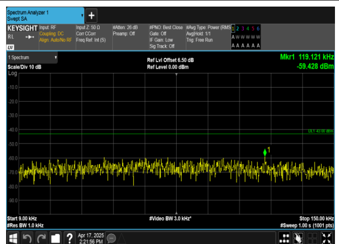
Band2-15MHz-16QAM-18900-1RB#74-0.009~0.15-PASS
