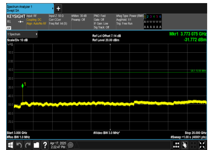
Band2-15MHz-16QAM-18900-1RB#74-3000~20000-PASS
