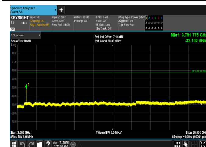
Band2-15MHz-QPSK-19125-1RB#0-3000~20000-PASS
