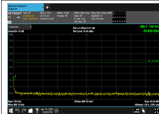
Band2-15MHz-16QAM-18675-75RB#0-0.15~30-PASS
