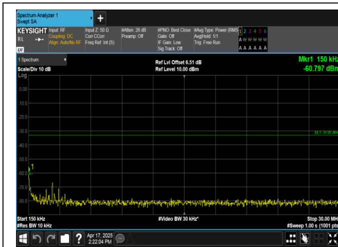
Band2-15MHz-16QAM-18900-1RB#74-0.15~30-PASS
