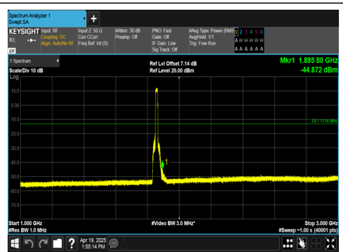
Band2-15MHz-QPSK-18675-75RB#0-1000~3000-PASS
