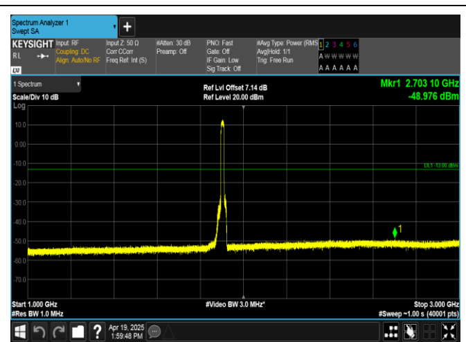
Band2-15MHz-QPSK-19125-75RB#0-1000~3000-PASS
