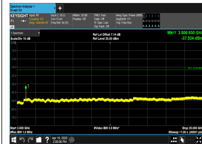
Band2-15MHz-QPSK-19125-75RB#0-3000~20000-PASS
