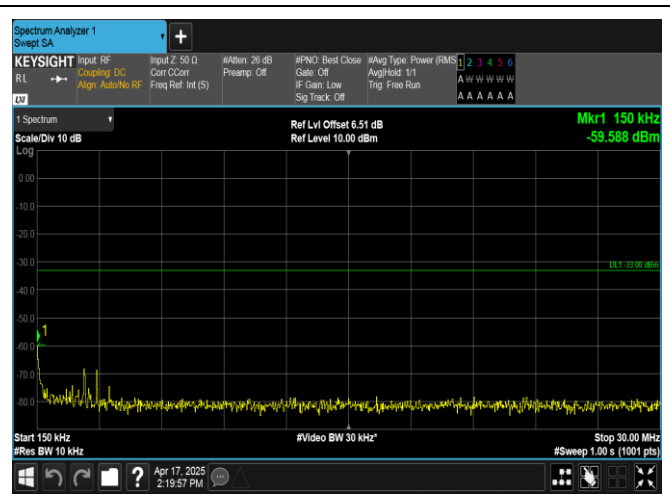
Band2-15MHz-16QAM-18900-1RB#0-0.15~30-PASS
