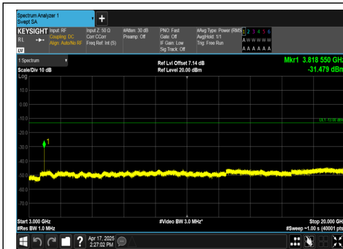
Band2-15MHz-16QAM-19125-1RB#74-3000~20000-PASS
