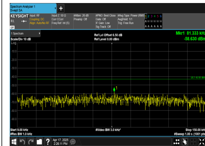
Band2-15MHz-16QAM-19125-1RB#74-0.009~0.15-PASS
