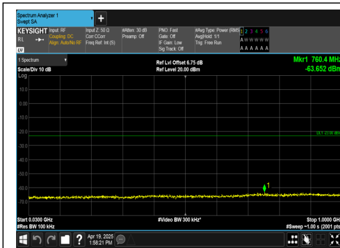
Band2-15MHz-16QAM-18900-75RB#0-30~1000-PASS
