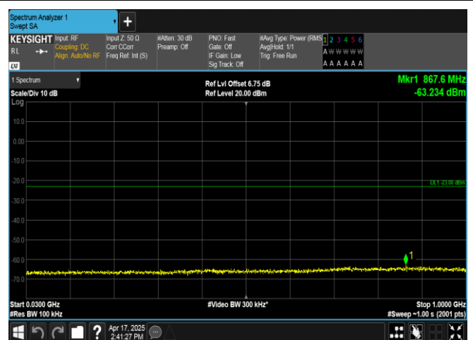
Band2-20MHz-16QAM-18700-1RB#0-30~1000-PASS
