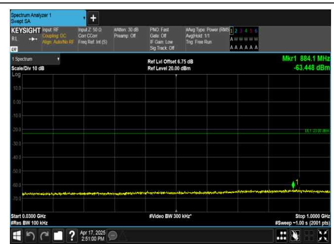
Band2-20MHz-QPSK-19100-1RB#99-30~1000-PASS
