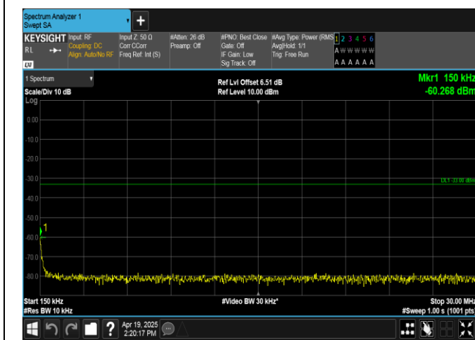
Band2-20MHz-16QAM-18700-100RB#0-0.15~30-PASS
