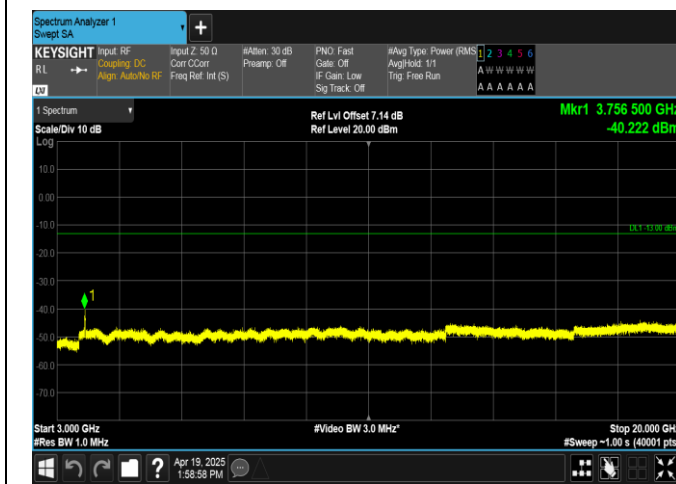
Band2-15MHz-16QAM-18900-75RB#0-3000~20000-PASS
