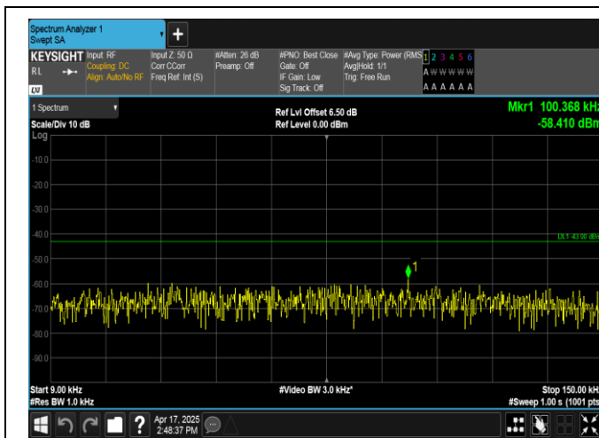
Band2-20MHz-QPSK-19100-1RB#0-0.009~0.15-PASS
