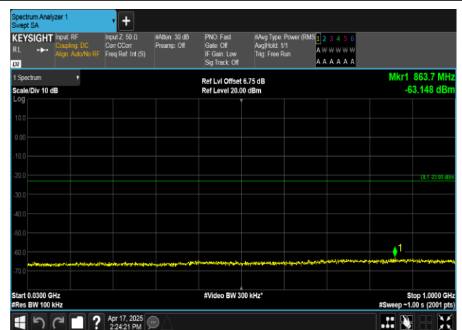
Band2-15MHz-16QAM-19125-1RB#0-30~1000-PASS
