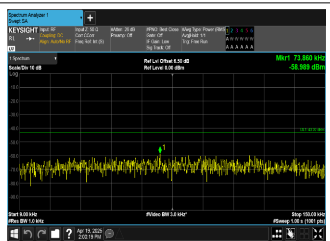
Band2-15MHz-16QAM-19125-75RB#0-0.009~0.15-PASS
