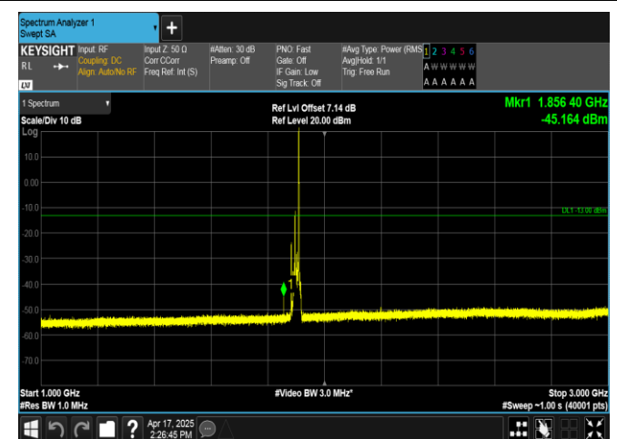
Band2-15MHz-16QAM-19125-1RB#74-1000~3000-PASS
