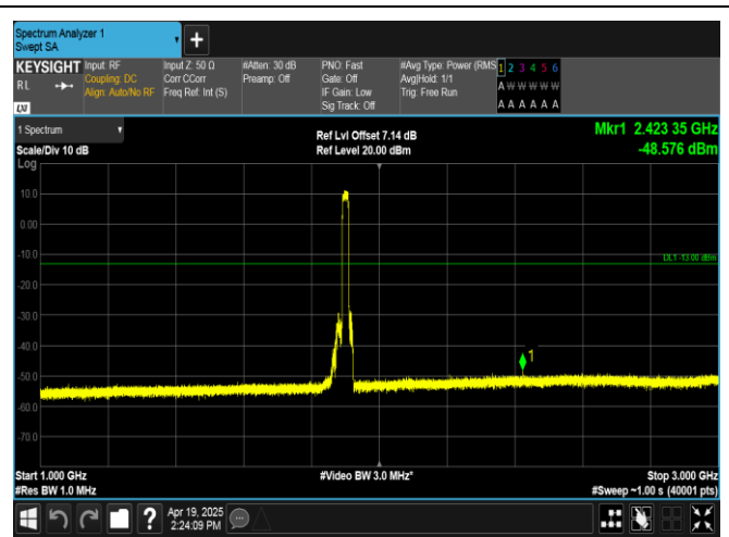
Band2-20MHz-QPSK-19100-100RB#0-1000~3000-PASS
