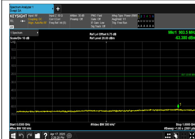
Band2-15MHz-16QAM-19125-1RB#74-30~1000-PASS
