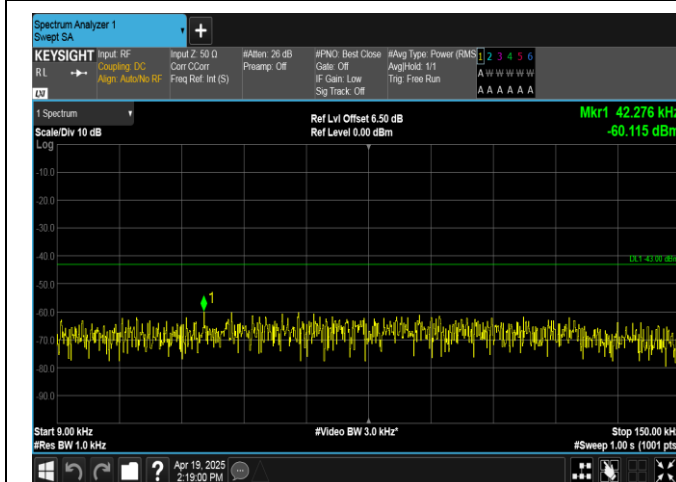
Band2-20MHz-QPSK-18700-100RB#0-0.009~0.15-PASS
