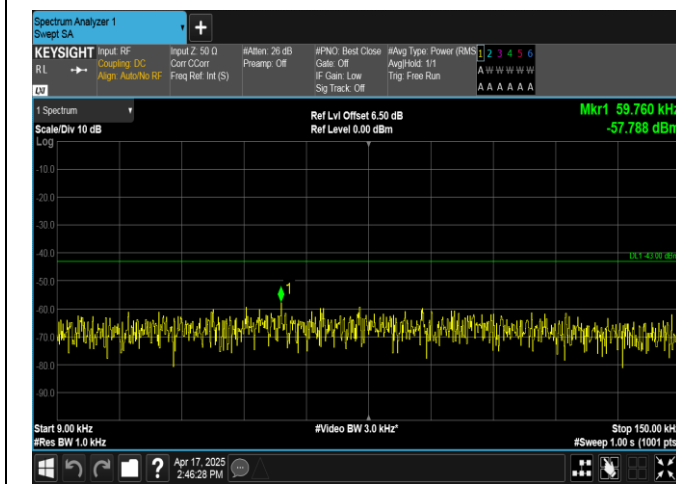
Band2-20MHz-QPSK-18900-1RB#99-0.009~0.15-PASS
