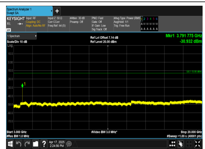
Band2-15MHz-16QAM-19125-1RB#0-3000~20000-PASS
