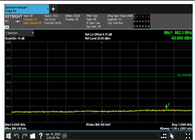
Band2-15MHz-16QAM-19125-75RB#0-30~1000-PASS
