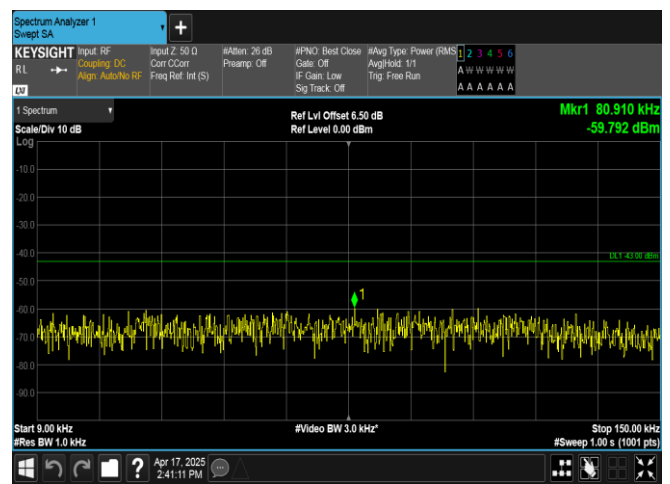
Band2-20MHz-16QAM-18700-1RB#0-0.009~0.15-PASS
