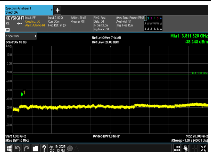
Band2-15MHz-16QAM-19125-75RB#0-3000~20000-PASS
