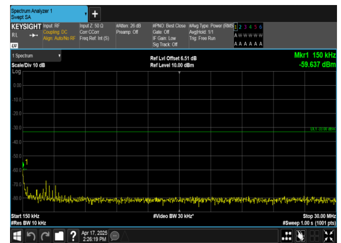
Band2-15MHz-16QAM-19125-1RB#74-0.15~30-PASS
