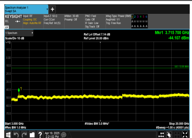
Band2-20MHz-16QAM-18700-100RB#0-3000~20000-PAS
