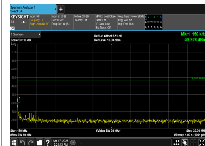
Band2-15MHz-16QAM-19125-1RB#0-0.15~30-PASS
