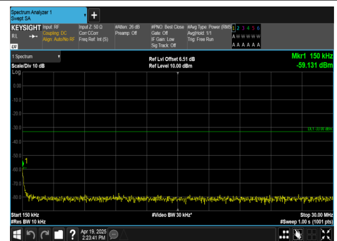
Band2-20MHz-QPSK-19100-100RB#0-0.15~30-PASS
