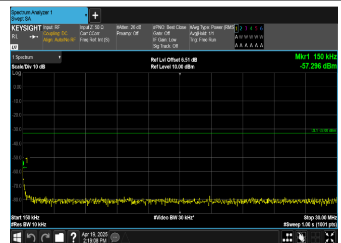
Band2-20MHz-QPSK-18700-100RB#0-0.15~30-PASS
