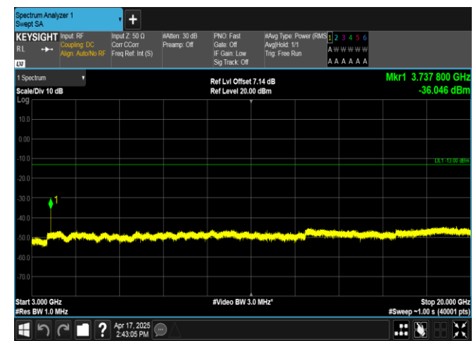
Band2-20MHz-QPSK-18700-1RB#99-3000~20000-PASS
