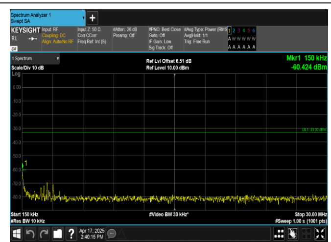
Band2-20MHz-QPSK-18700-1RB#0-0.15~30-PASS
