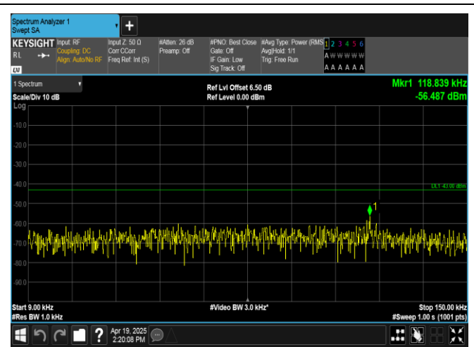
Band2-20MHz-16QAM-18700-100RB#0-0.009~0.15-PASS
