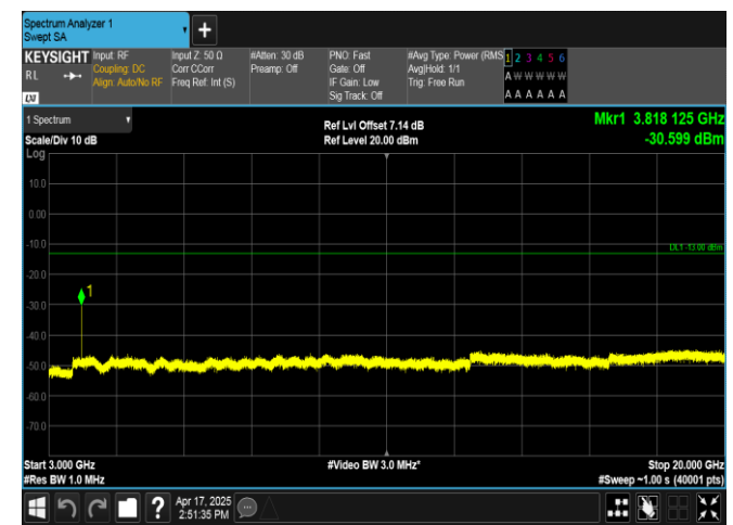
Band2-20MHz-QPSK-19100-1RB#99-3000~20000-PASS
