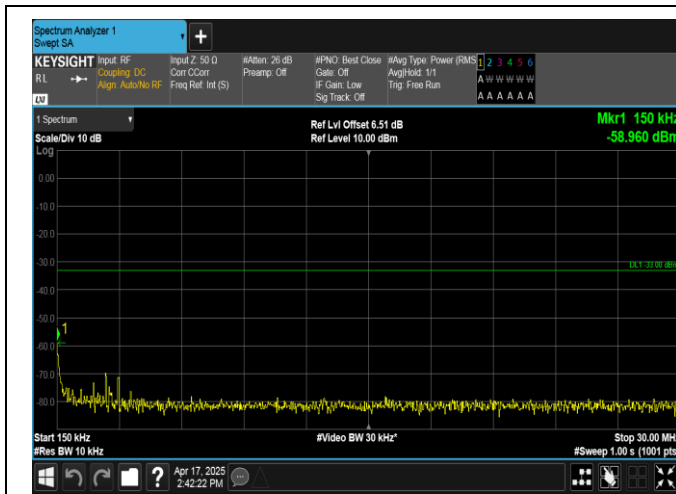
Band2-20MHz-QPSK-18700-1RB#99-0.15~30-PASS
