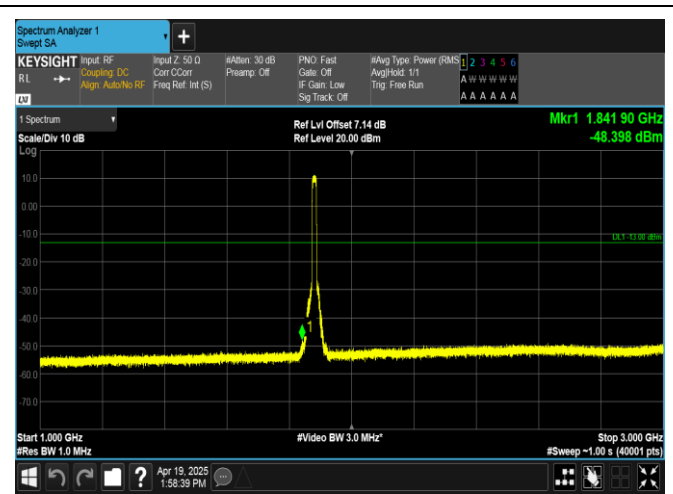
Band2-15MHz-16QAM-18900-75RB#0-1000~3000-PASS
