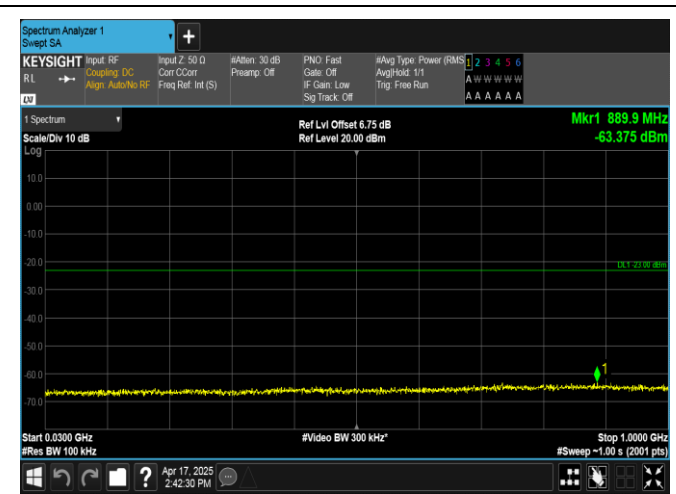
Band2-20MHz-QPSK-18700-1RB#99-30~1000-PASS
