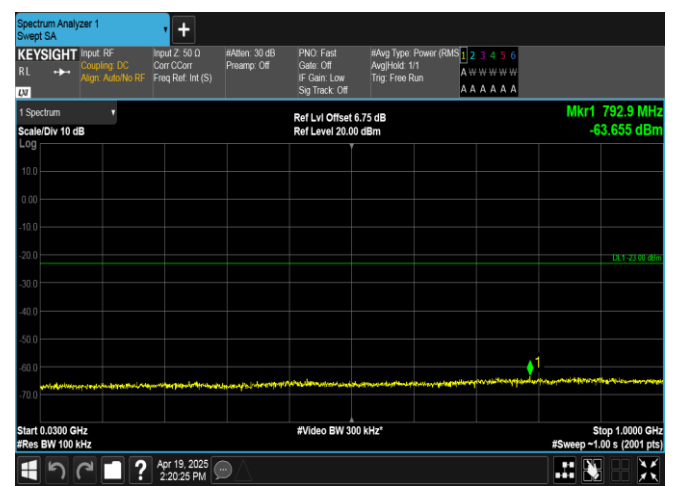
Band2-20MHz-16QAM-18700-100RB#0-30~1000-PASS
