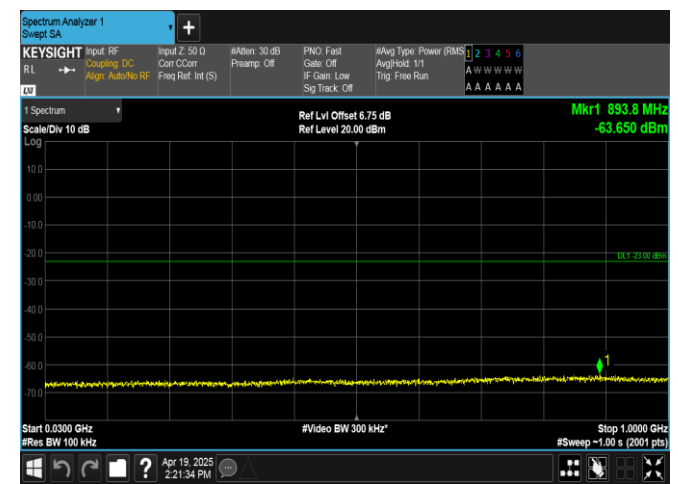
Band2-20MHz-QPSK-18900-100RB#0-30~1000-PASS
