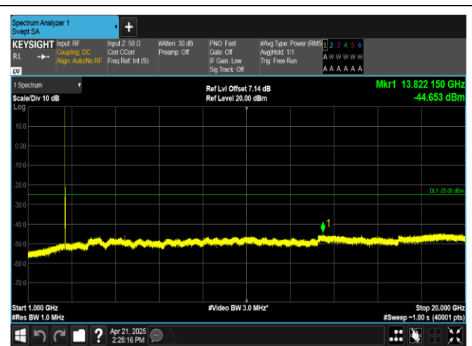
Band38-20MHz-QPSK-38150-1RB#0-1000~20000-PASS
