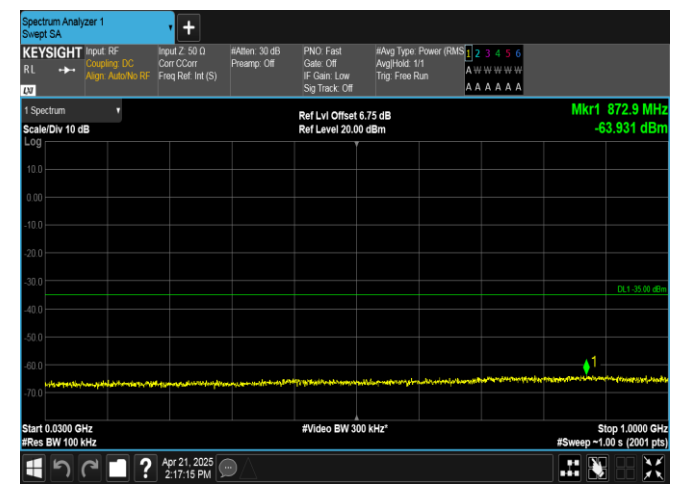
Band38-20MHz-16QAM-37850-1RB#0-30~1000-PASS
