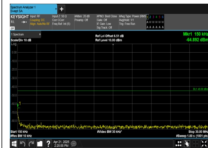
Band38-20MHz-16QAM-38150-1RB#0-0.15~30-PASS
