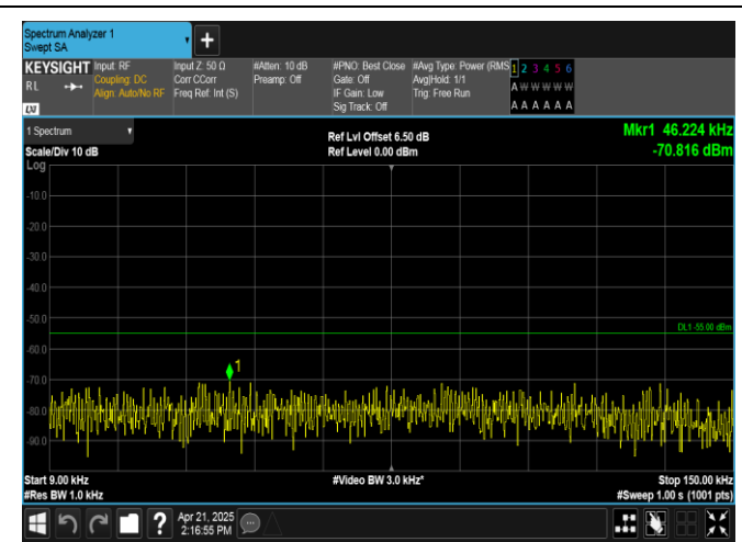
Band38-20MHz-16QAM-37850-1RB#0-0.009~0.15-PASS
