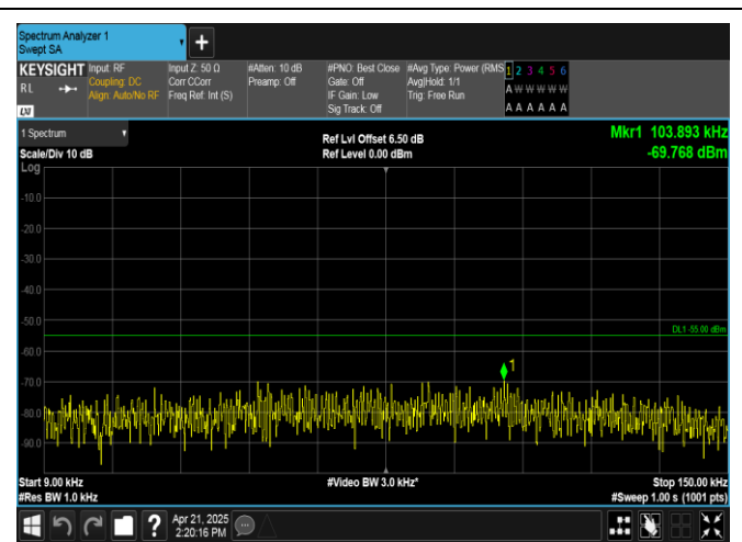
Band38-20MHz-QPSK-38000-1RB#0-0.009~0.15-PASS
