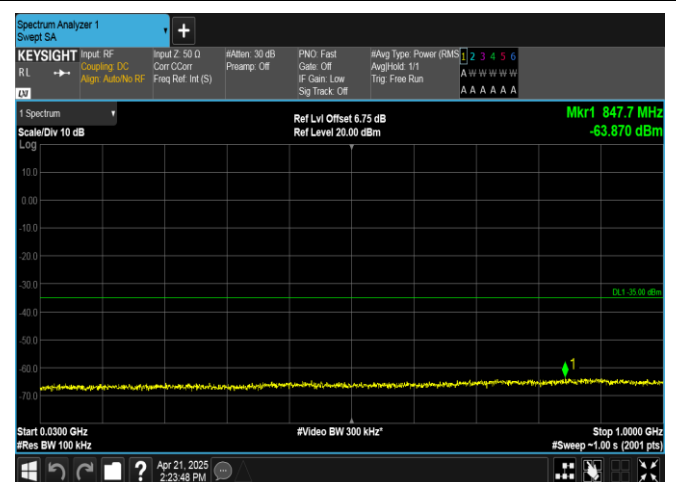
Band38-20MHz-16QAM-38000-1RB#99-30~1000-PASS
