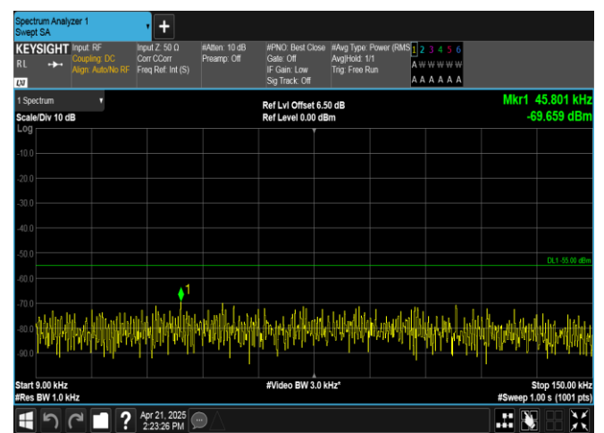
Band38-20MHz-16QAM-38000-1RB#99-0.009~0.15-PASS
