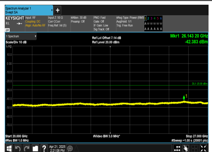
Band38-20MHz-QPSK-38000-1RB#0-20000~27000-PASS
