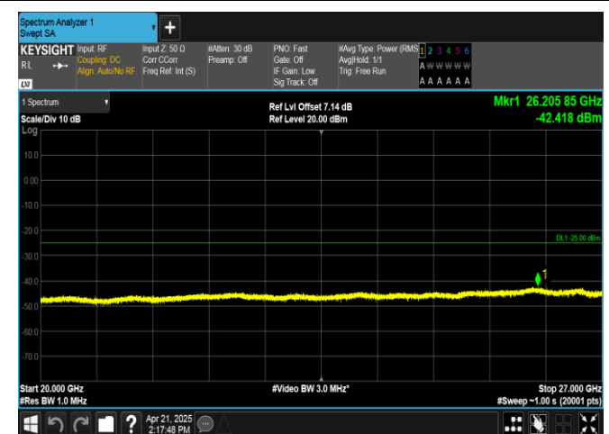
Band38-20MHz-16QAM-37850-1RB#0-20000~27000-PASS
