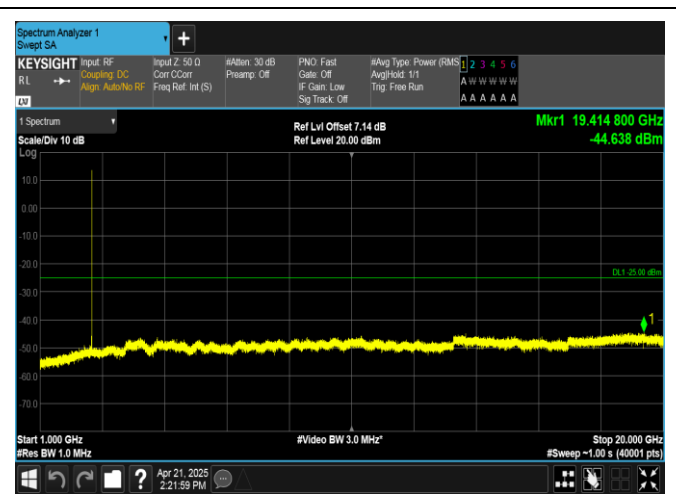
Band38-20MHz-16QAM-38000-1RB#0-1000~20000-PASS
