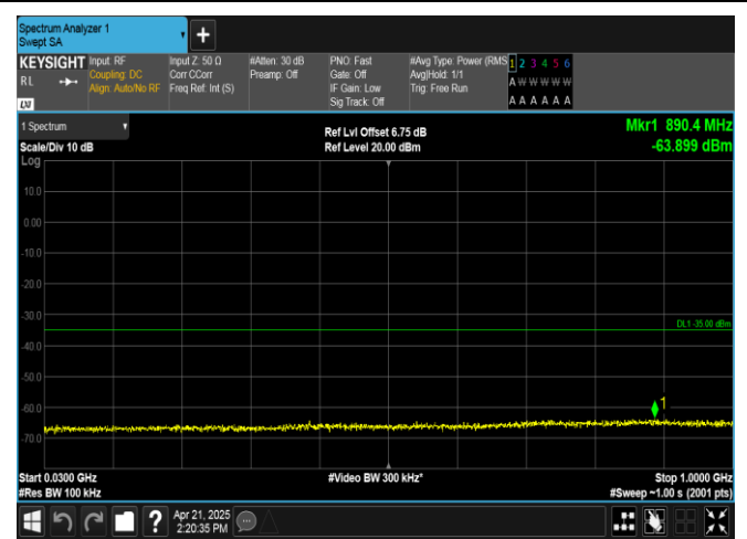
Band38-20MHz-QPSK-38000-1RB#0-30~1000-PASS
