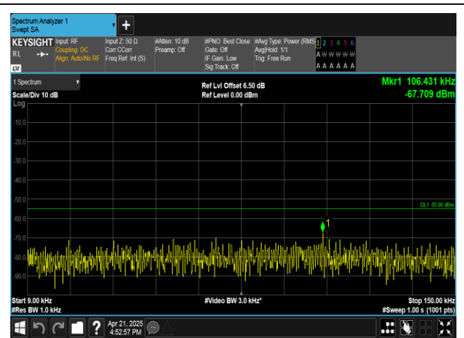
Band41-15MHz-QPSK-40620-1RB#0-0.009~0.15-PASS
