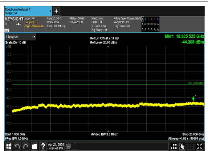
Band41-15MHz-16QAM-40620-1RB#0-1000~20000-PASS
