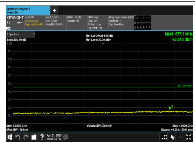
Band41-15MHz-QPSK-40620-75RB#0-30~1000-PASS
