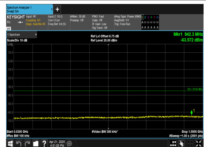
Band41-15MHz-QPSK-39725-1RB#74-30~1000-PASS
