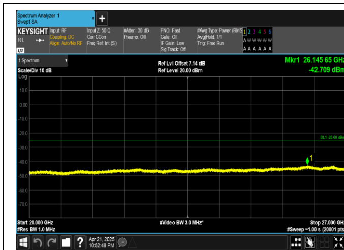
Band41-15MHz-QPSK-39725-75RB#0-20000~27000-PASS
