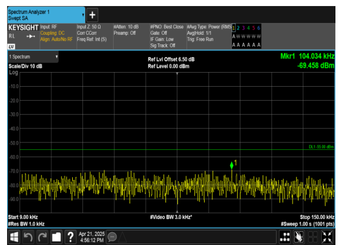
Band41-15MHz-16QAM-40620-1RB#74-0.009~0.15-PASS
