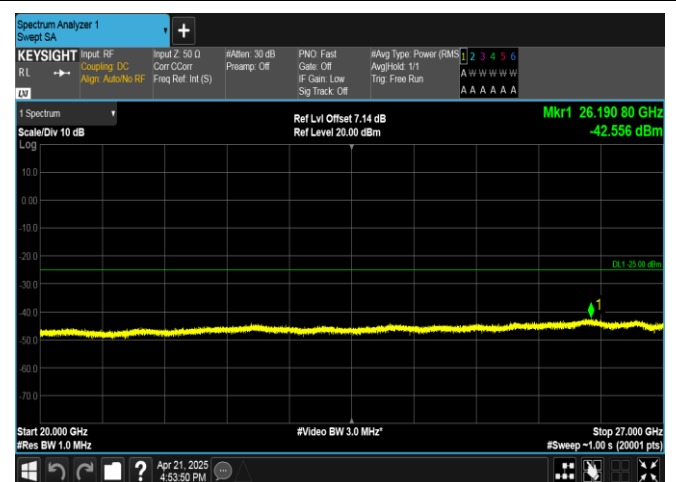
Band41-15MHz-QPSK-40620-1RB#0-20000~27000-PASS
