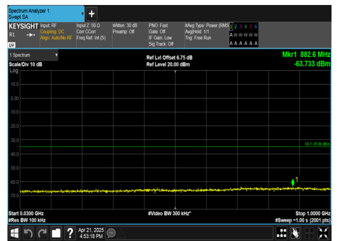
Band41-15MHz-QPSK-40620-1RB#0-30~1000-PASS
