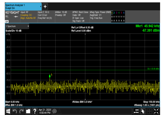
Band41-15MHz-QPSK-39725-1RB#74-0.009~0.15-PASS
