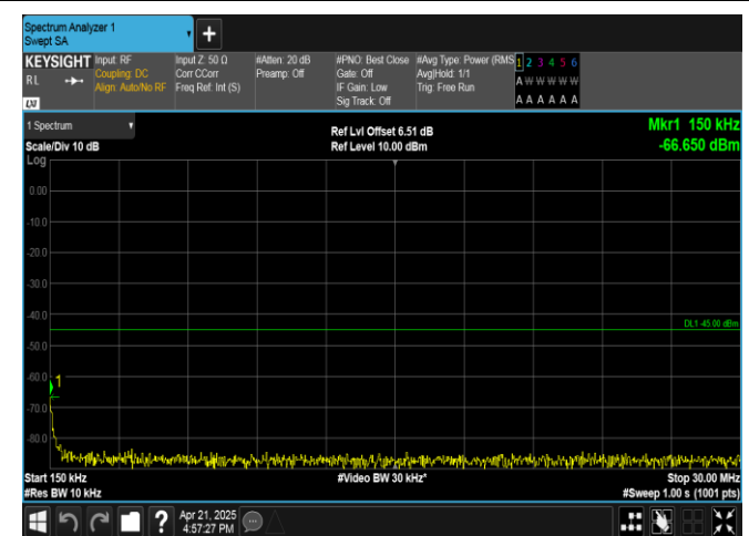
Band41-15MHz-QPSK-41515-1RB#0-0.15~30-PASS
