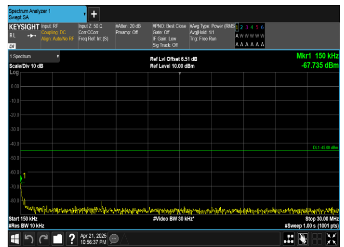
Band41-15MHz-QPSK-41515-75RB#0-0.15~30-PASS
