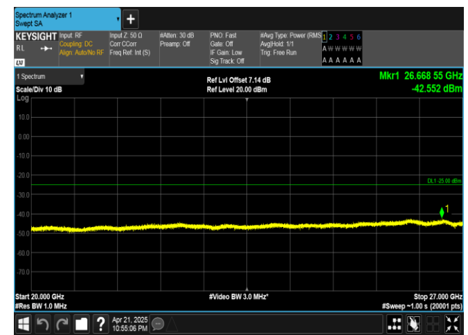
Band41-15MHz-QPSK-40620-75RB#0-20000~27000-PASS
