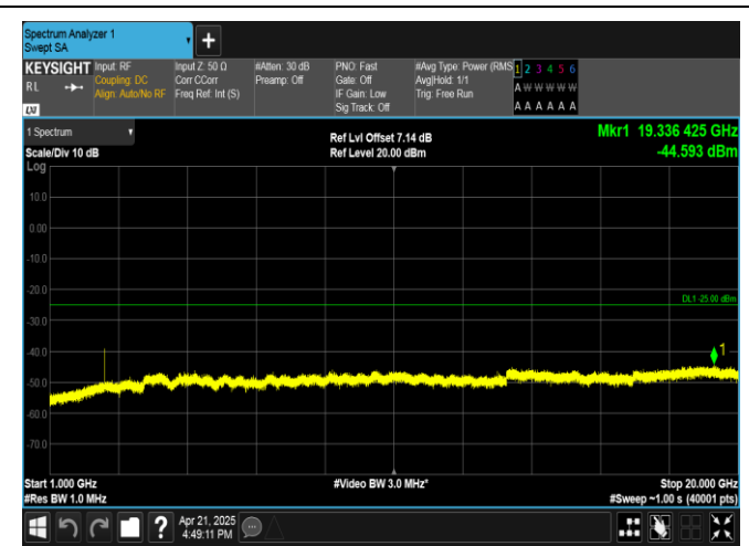
Band41-15MHz-QPSK-39725-1RB#0-1000~20000-PASS
