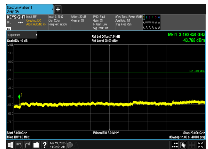
Band66-3MHz-QPSK-132322-15RB#0-3000~20000-PASS
