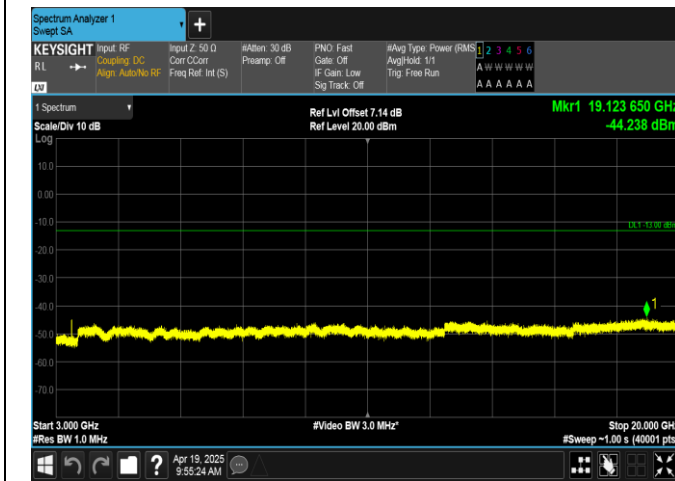
Band66-3MHz-QPSK-131987-15RB#0-3000~20000-PASS
