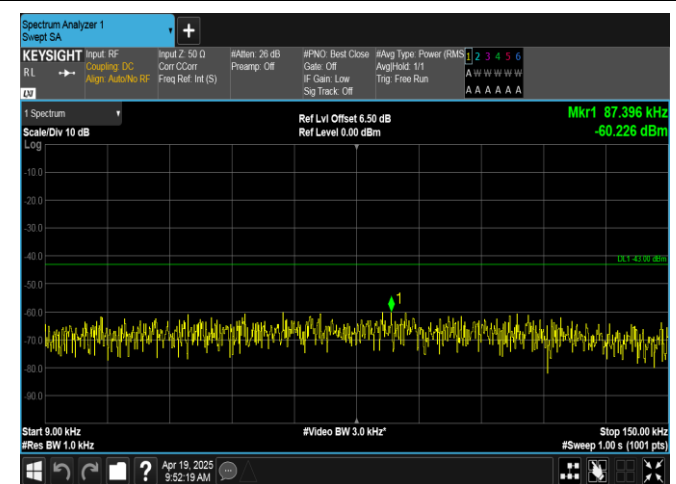
Band66-3MHz-QPSK-131987-1RB#14-0.009~0.15-PASS
