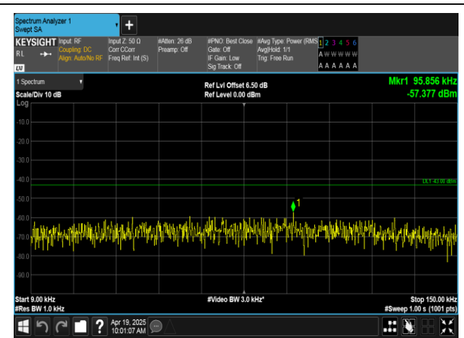
Band66-3MHz-QPSK-132322-15RB#0-0.009~0.15-PASS
