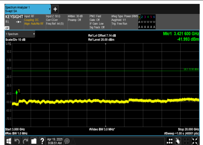
Band66-1.4MHz-16QAM-131979-6RB#0-3000~20000-PASS
