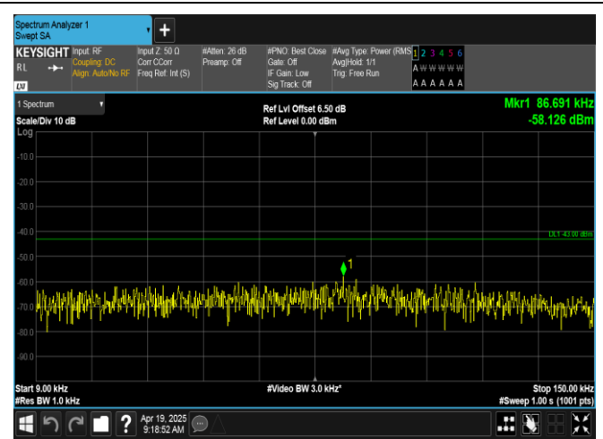
Band66-1.4MHz-16QAM-132665-6RB#0-0.009~0.15-PASS
