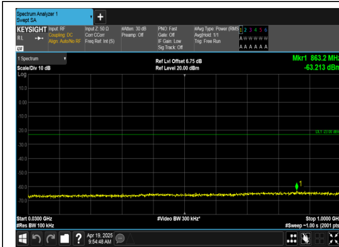
Band66-3MHz-QPSK-131987-15RB#0-30~1000-PASS
