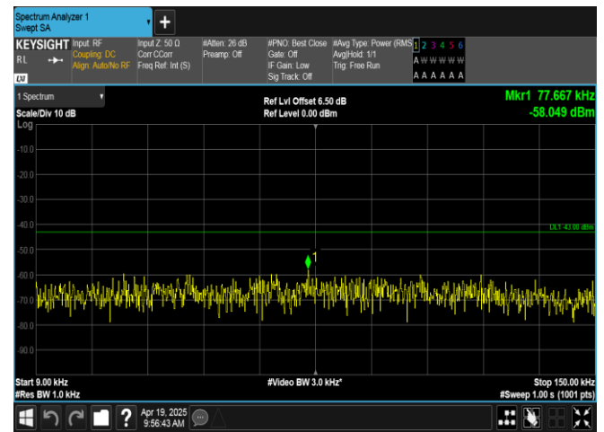
Band66-3MHz-QPSK-132322-1RB#0-0.009~0.15-PASS
