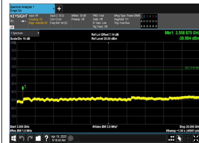
Band66-1.4MHz-QPSK-132665-6RB#0-3000~20000-PASS
