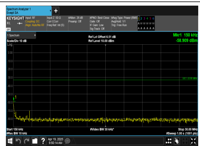
Band66-3MHz-QPSK-131987-1RB#0-0.15~30-PASS
