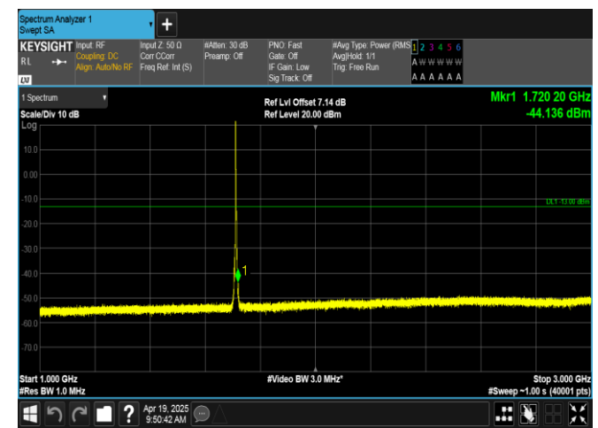
Band66-3MHz-QPSK-131987-1RB#0-1000~3000-PASS
