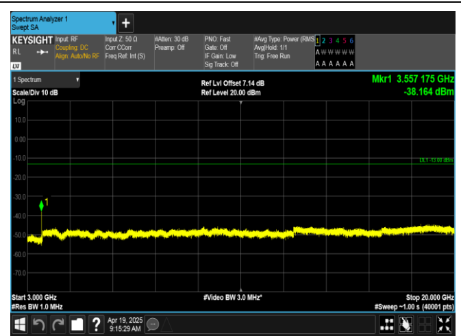
Band66-1.4MHz-16QAM-132665-1RB#0-3000~20000-PASS
