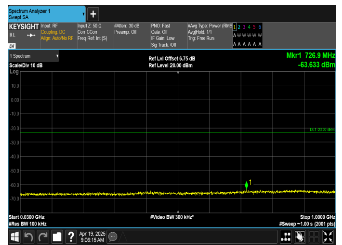
Band66-1.4MHz-16QAM-131979-6RB#0-30~1000-PASS
