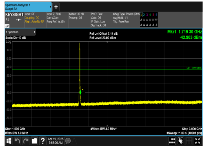
Band66-3MHz-QPSK-131987-15RB#0-1000~3000-PASS
