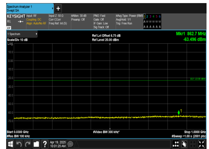
Band66-3MHz-QPSK-132322-15RB#0-30~1000-PASS
