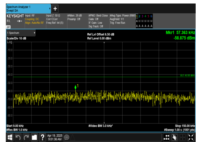
Band66-1.4MHz-16QAM-131979-1RB#0-0.009~0.15-PASS
