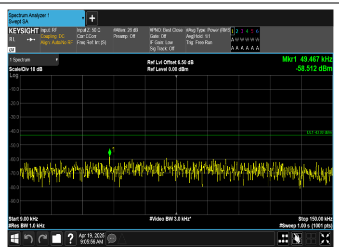
Band66-1.4MHz-16QAM-131979-6RB#0-0.009~0.15-PASS
