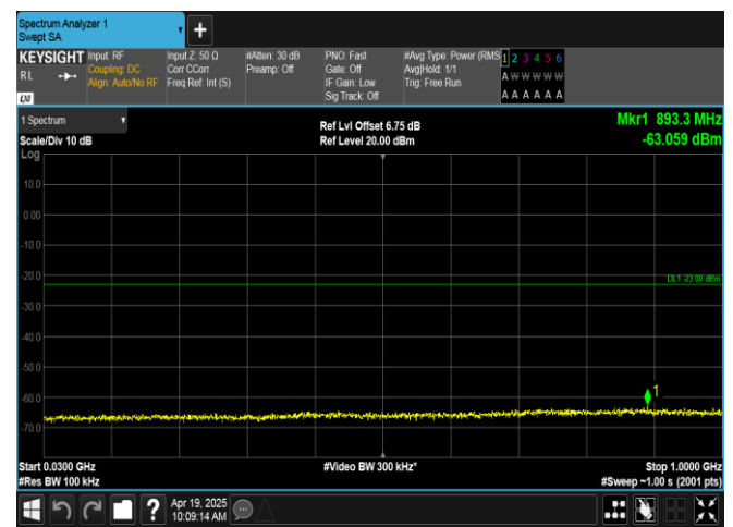
Band66-3MHz-16QAM-132657-15RB#0-30~1000-PASS
