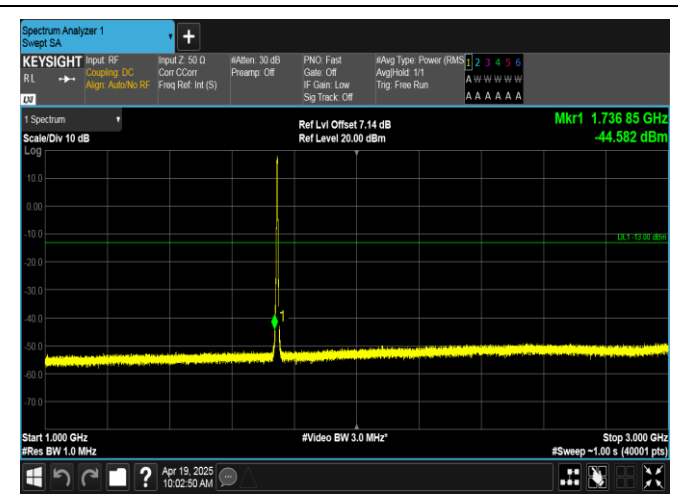
Band66-3MHz-16QAM-132322-15RB#0-1000~3000-PASS
