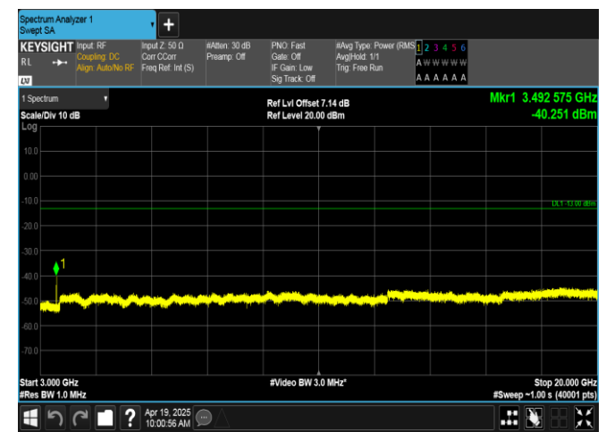
Band66-3MHz-16QAM-132322-1RB#14-3000~20000-PASS
