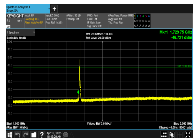
Band66-5MHz-QPSK-132322-1RB#24-1000~3000-PASS
