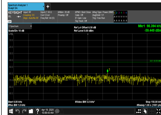
Band66-3MHz-16QAM-132657-1RB#14-0.009~0.15-PASS
