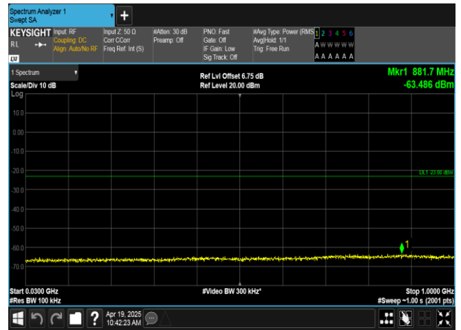
Band66-5MHz-QPSK-131997-1RB#24-30~1000-PASS
