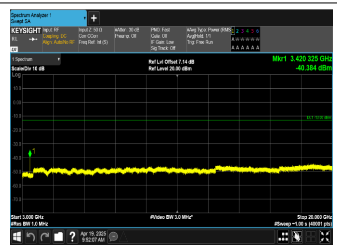
Band66-3MHz-16QAM-131987-1RB#0-3000~20000-PASS
