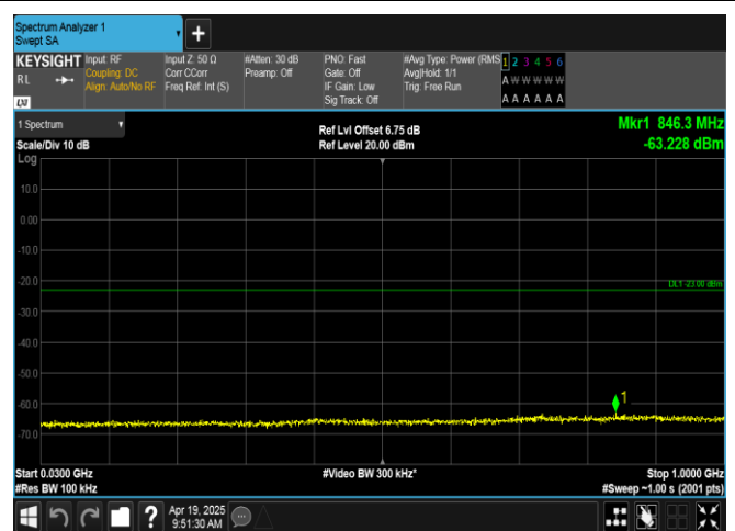
Band66-3MHz-16QAM-131987-1RB#0-30~1000-PASS
