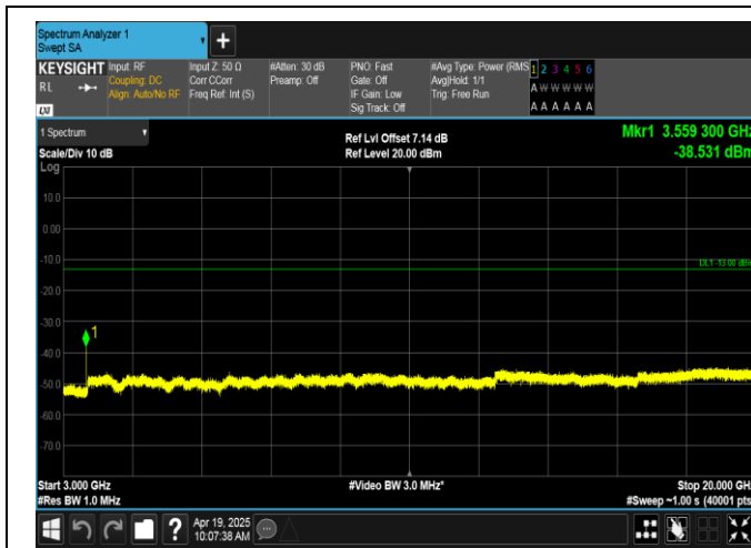
Band66-3MHz-16QAM-132657-1RB#14-3000~20000-PASS
