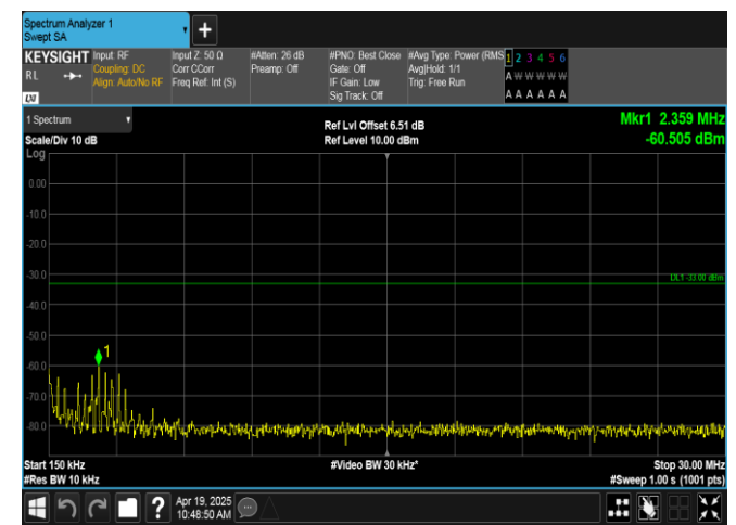
Band66-5MHz-QPSK-132322-1RB#24-0.15~30-PASS
