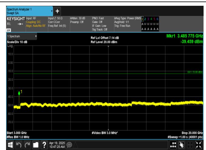
Band66-5MHz-QPSK-132322-1RB#0-3000~20000-PASS
