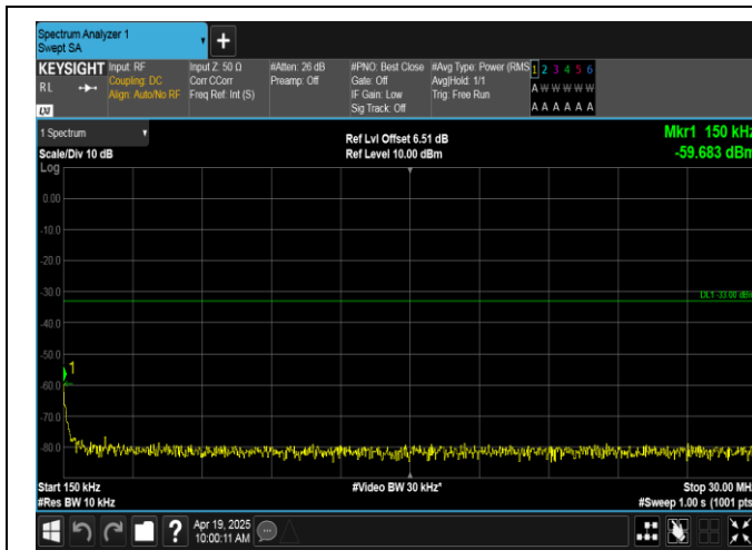
Band66-3MHz-16QAM-132322-1RB#14-0.15~30-PASS
