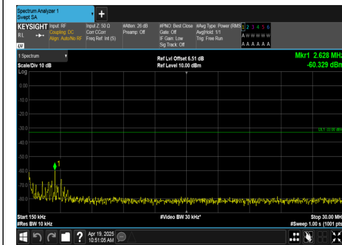
Band66-5MHz-QPSK-132322-25RB#0-0.15~30-PASS
