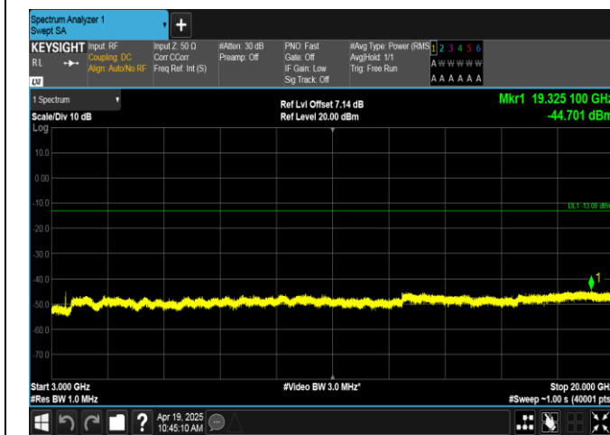
Band66-5MHz-QPSK-131997-25RB#0-3000~20000-PASS
