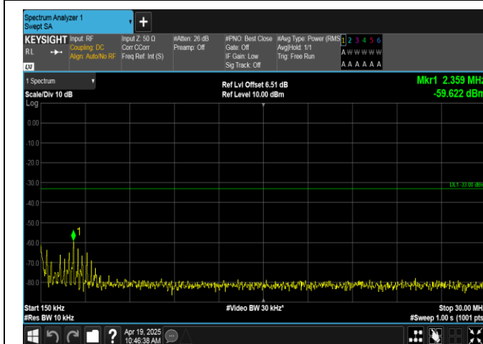
Band66-5MHz-QPSK-132322-1RB#0-0.15~30-PASS
