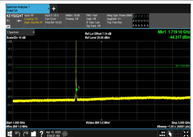
Band66-3MHz-16QAM-131987-1RB#14-1000~3000-PASS
