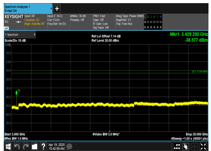
Band66-5MHz-QPSK-131997-1RB#24-3000~20000-PASS
