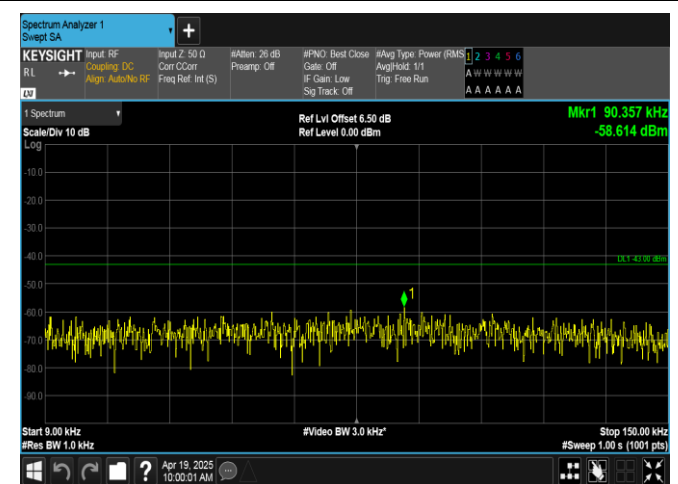
Band66-3MHz-16QAM-132322-1RB#14-0.009~0.15-PASS
