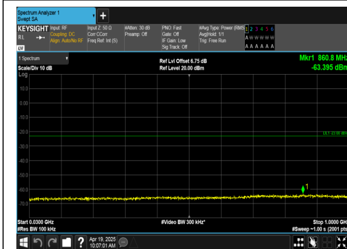
Band66-3MHz-16QAM-132657-1RB#14-30~1000-PASS
