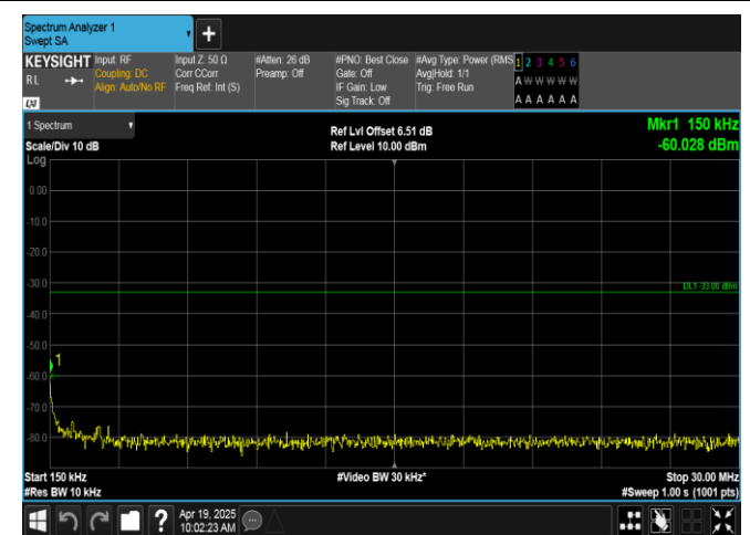
Band66-3MHz-16QAM-132322-15RB#0-0.15~30-PASS
