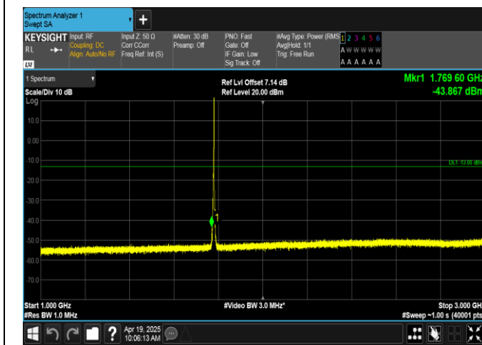
Band66-3MHz-QPSK-132657-1RB#14-1000~3000-PASS
