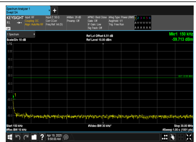
Band66-3MHz-16QAM-132322-1RB#0-0.15~30-PASS
