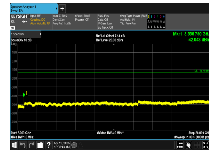
Band66-3MHz-QPSK-132657-15RB#0-3000~20000-PASS
