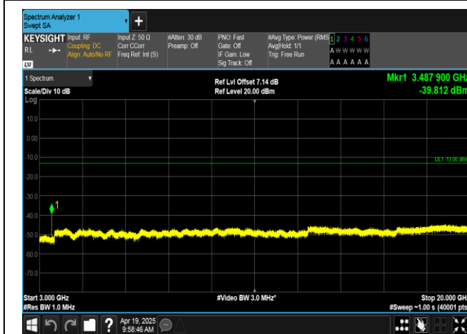
Band66-3MHz-16QAM-132322-1RB#0-3000~20000-PASS
