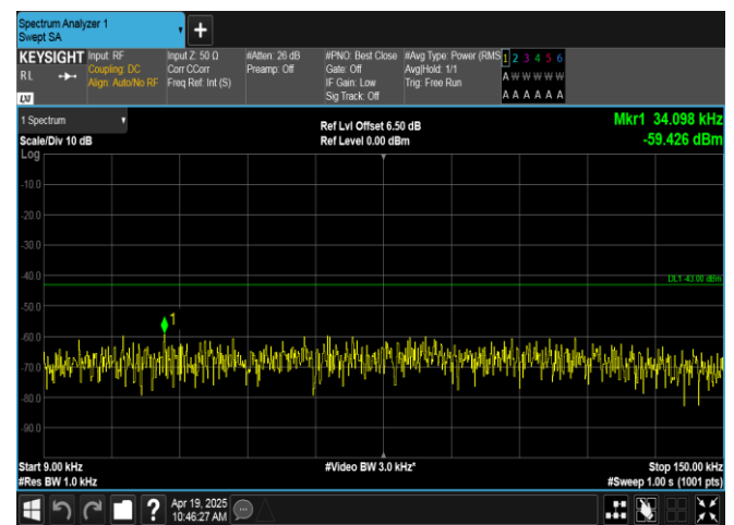
Band66-5MHz-QPSK-132322-1RB#0-0.009~0.15-PASS
