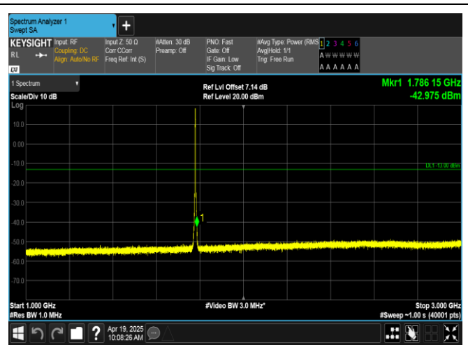
Band66-3MHz-QPSK-132657-15RB#0-1000~3000-PASS
