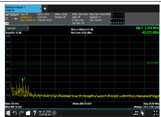
Band66-5MHz-QPSK-131997-1RB#0-0.15~30-PASS
