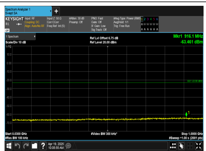
Band66-3MHz-QPSK-132657-1RB#14-30~1000-PASS
