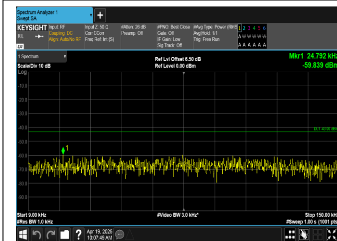
Band66-3MHz-QPSK-132657-15RB#0-0.009~0.15-PASS
