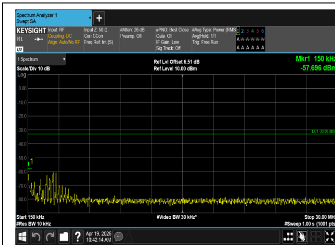
Band66-5MHz-QPSK-131997-1RB#24-0.15~30-PASS
