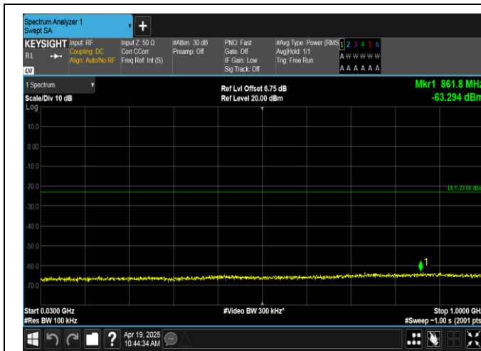
Band66-5MHz-QPSK-131997-25RB#0-30~1000-PASS
