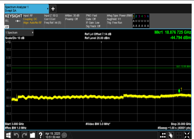
Band66-5MHz-QPSK-132322-25RB#0-3000~20000-PASS
