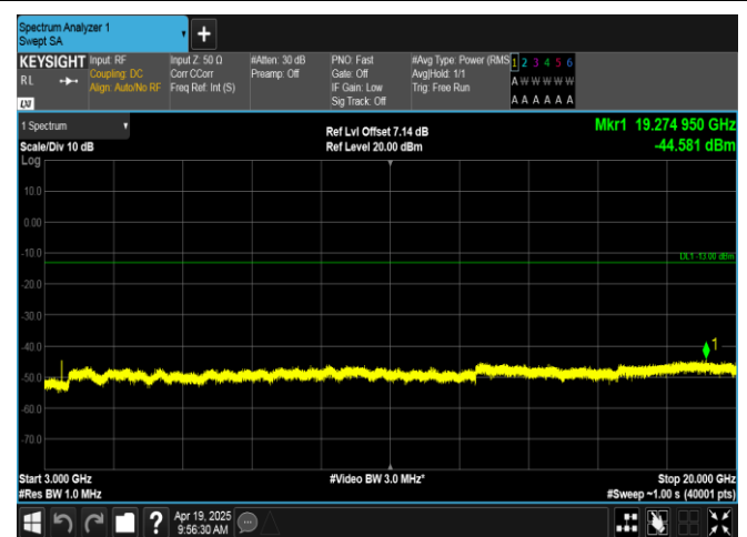
Band66-3MHz-16QAM-131987-15RB#0-3000~20000-PASS
