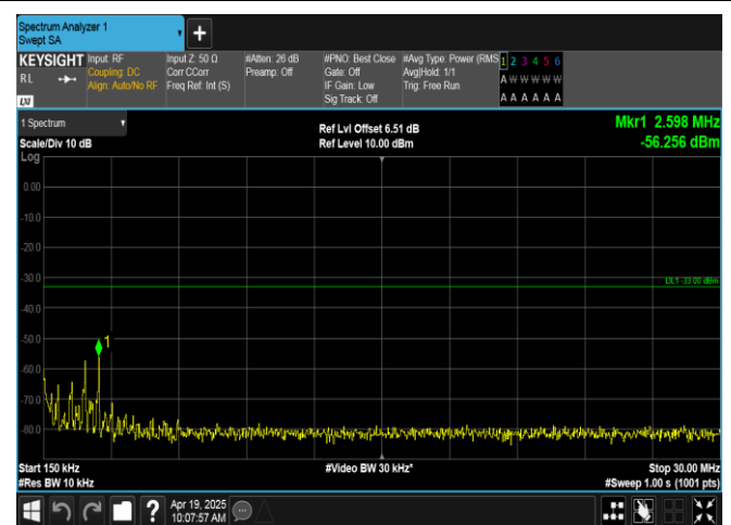
Band66-3MHz-QPSK-132657-15RB#0-0.15~30-PASS
