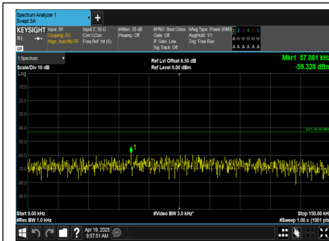
Band66-3MHz-16QAM-132322-1RB#0-0.009~0.15-PASS
