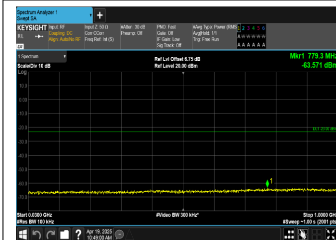
Band66-5MHz-QPSK-132322-1RB#24-30~1000-PASS
