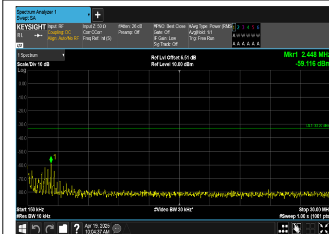
Band66-3MHz-16QAM-132657-1RB#0-0.15~30-PASS
