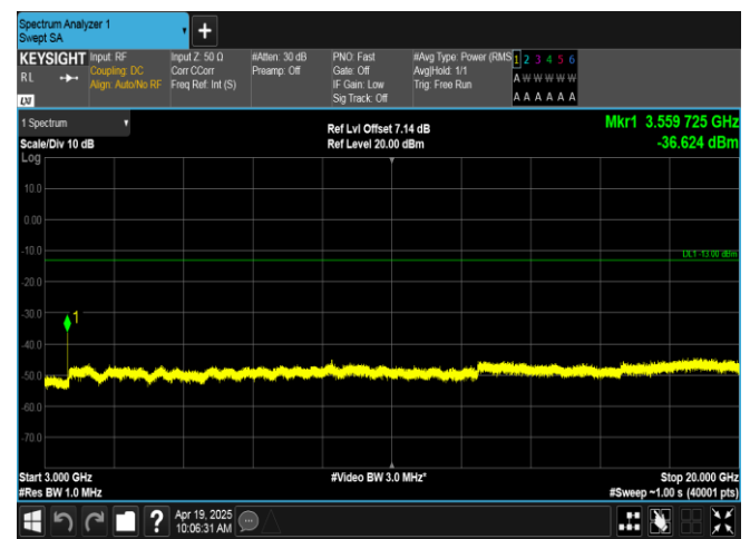
Band66-3MHz-QPSK-132657-1RB#14-3000~20000-PASS
