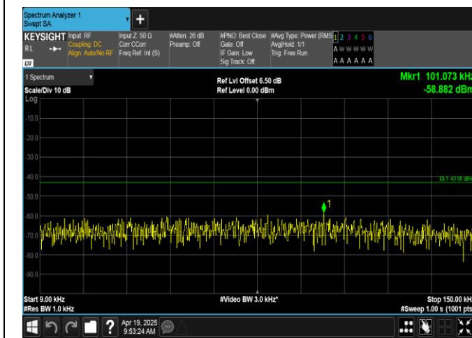
Band66-3MHz-16QAM-131987-1RB#14-0.009~0.15-PASS
