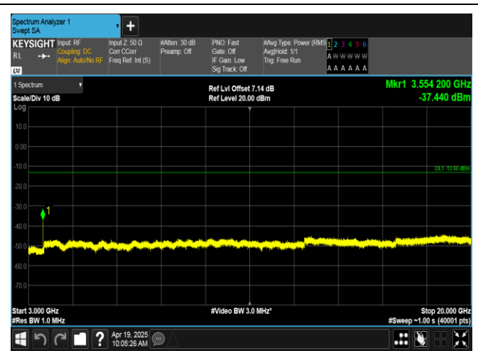
Band66-3MHz-16QAM-132657-1RB#0-3000~20000-PASS
