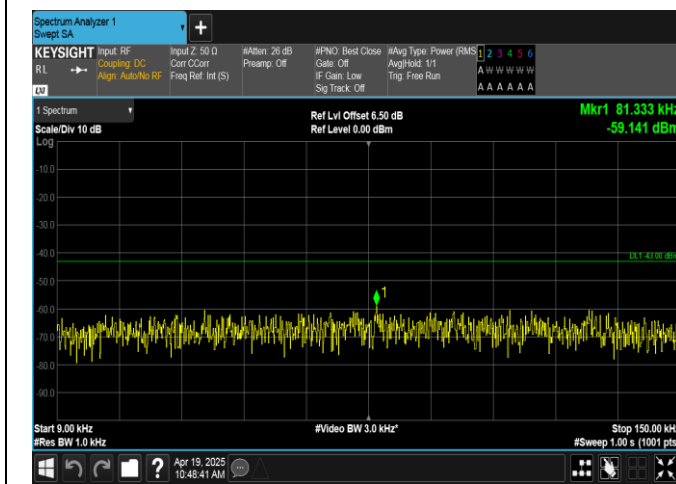
Band66-5MHz-QPSK-132322-1RB#24-0.009~0.15-PASS
