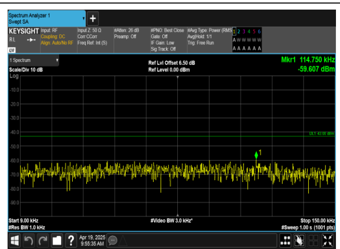
Band66-3MHz-16QAM-131987-15RB#0-0.009~0.15-PASS
