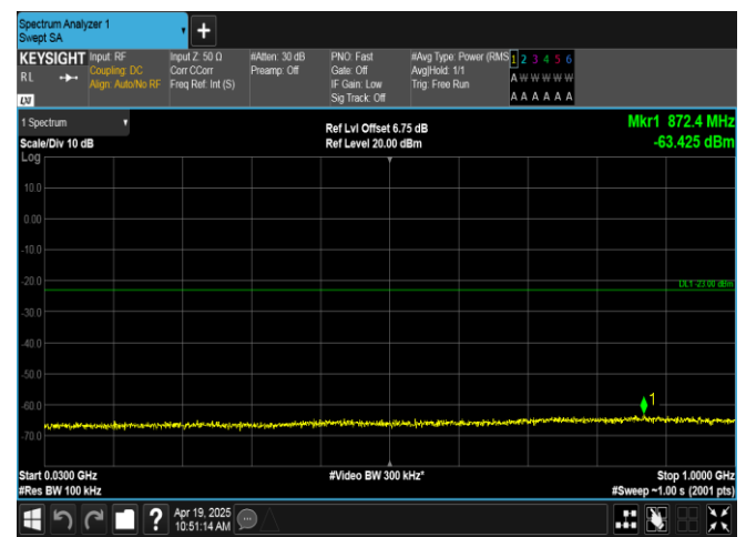
Band66-5MHz-QPSK-132322-25RB#0-30~1000-PASS
