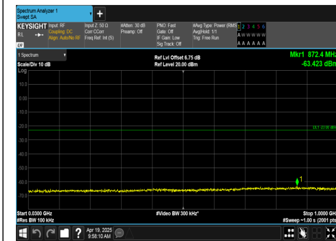
Band66-3MHz-16QAM-132322-1RB#0-30~1000-PASS
