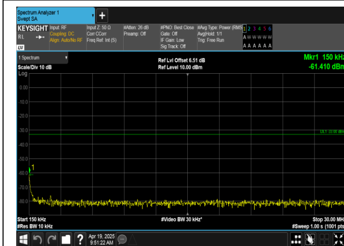
Band66-3MHz-16QAM-131987-1RB#0-0.15~30-PASS
