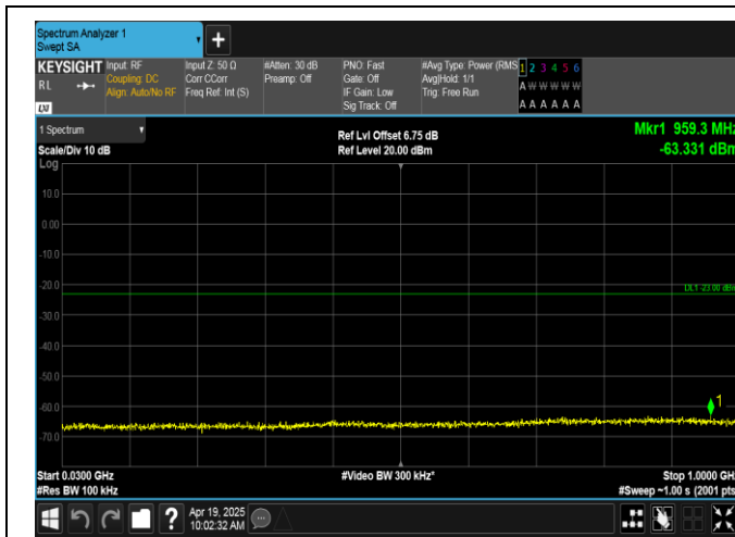
Band66-3MHz-16QAM-132322-15RB#0-30~1000-PASS
