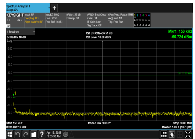
Band66-3MHz-16QAM-131987-1RB#14-0.15~30-PASS
