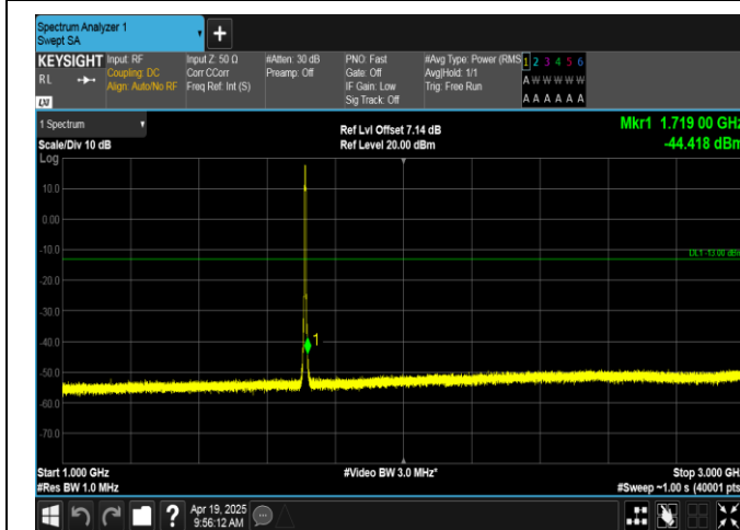
Band66-3MHz-16QAM-131987-15RB#0-1000~3000-PASS
