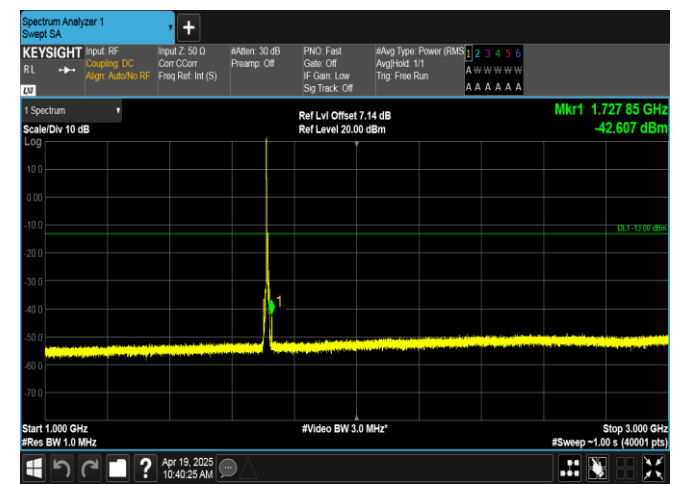
Band66-5MHz-QPSK-131997-1RB#0-1000~3000-PASS
