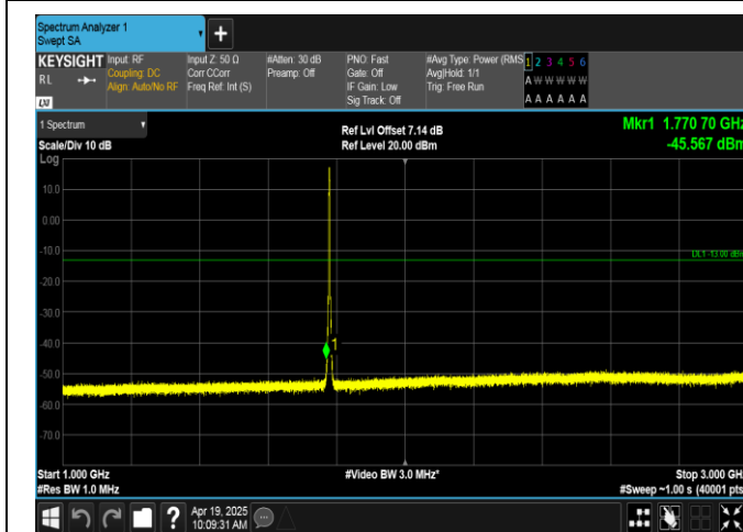
Band66-3MHz-16QAM-132657-15RB#0-1000~3000-PASS
