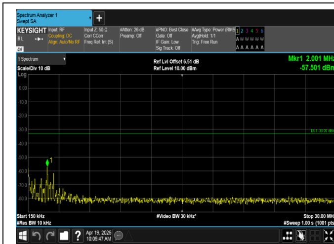
Band66-3MHz-QPSK-132657-1RB#14-0.15~30-PASS
