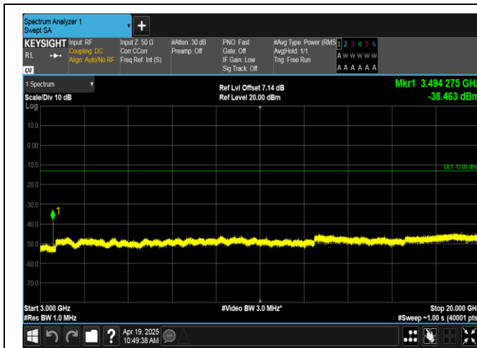
Band66-5MHz-QPSK-132322-1RB#24-3000~20000-PASS
