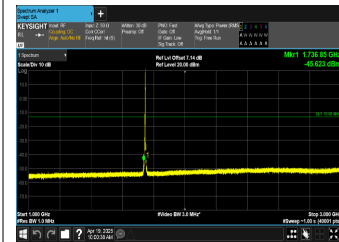
Band66-3MHz-16QAM-132322-1RB#14-1000~3000-PASS
