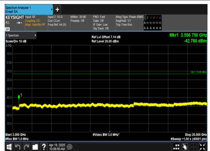
Band66-3MHz-16QAM-132657-15RB#0-3000~20000-PASS
