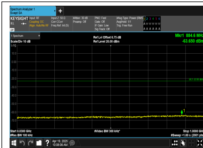
Band66-3MHz-QPSK-132657-15RB#0-30~1000-PASS
