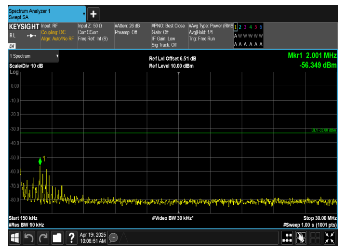
Band66-3MHz-16QAM-132657-1RB#14-0.15~30-PASS
