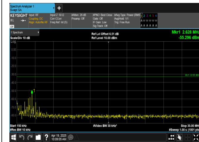
Band66-3MHz-16QAM-132657-15RB#0-0.15~30-PASS
