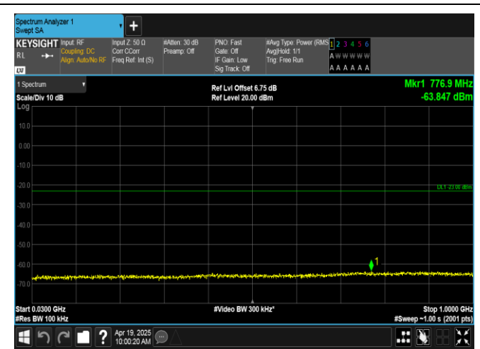
Band66-3MHz-16QAM-132322-1RB#14-30~1000-PASS
