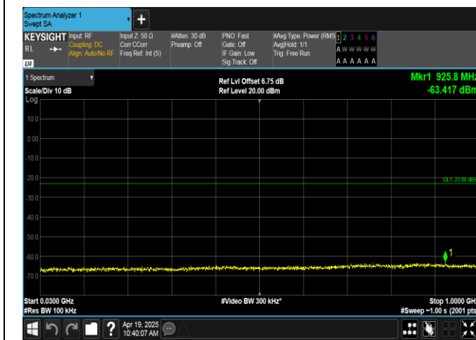
Band66-5MHz-QPSK-131997-1RB#0-30~1000-PASS
