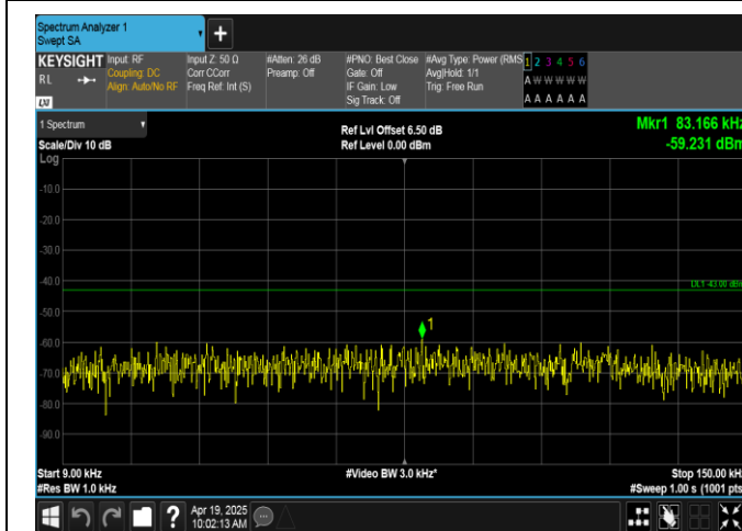
Band66-3MHz-16QAM-132322-15RB#0-0.009~0.15-PASS
