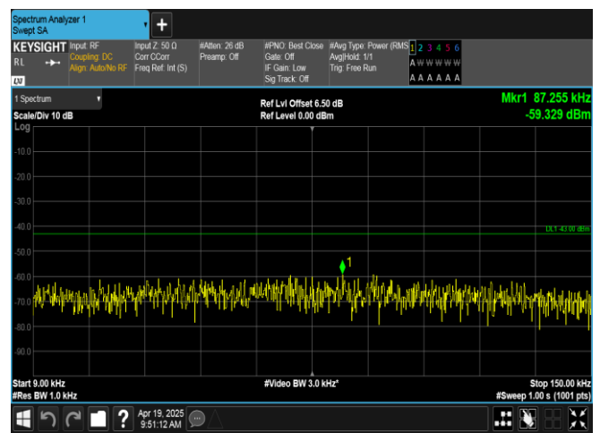
Band66-3MHz-16QAM-131987-1RB#0-0.009~0.15-PASS
