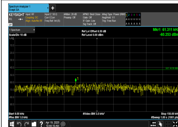
Band66-5MHz-QPSK-131997-25RB#0-0.009~0.15-PASS
