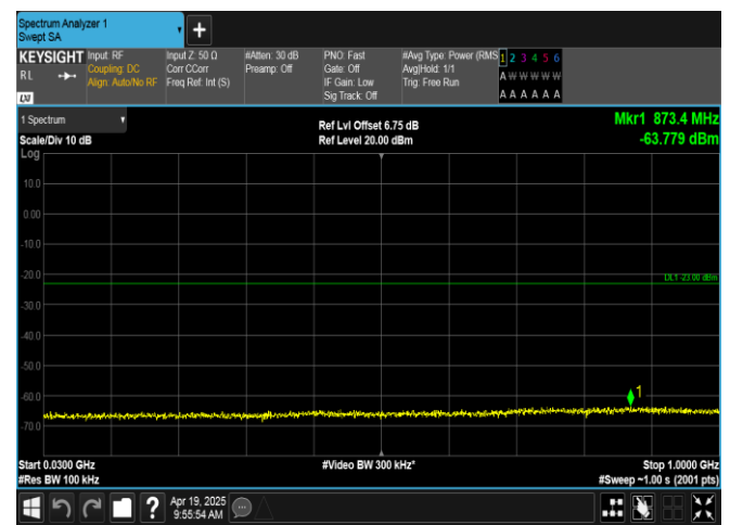
Band66-3MHz-16QAM-131987-15RB#0-30~1000-PASS
