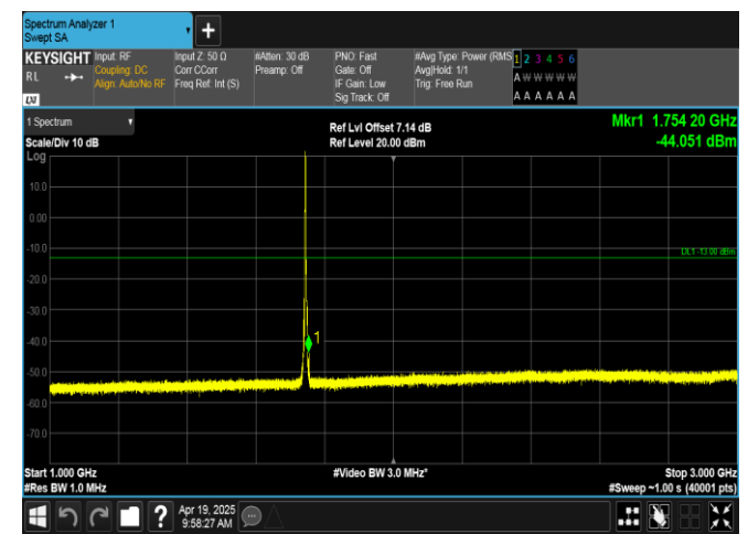
Band66-3MHz-16QAM-132322-1RB#0-1000~3000-PASS
