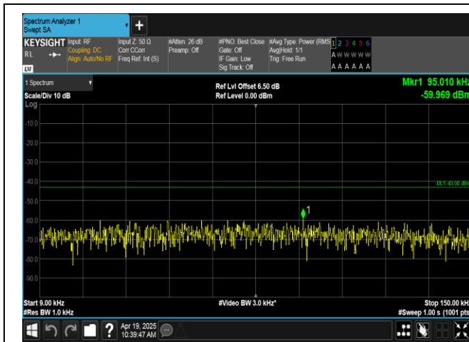
Band66-5MHz-QPSK-131997-1RB#0-0.009~0.15-PASS
