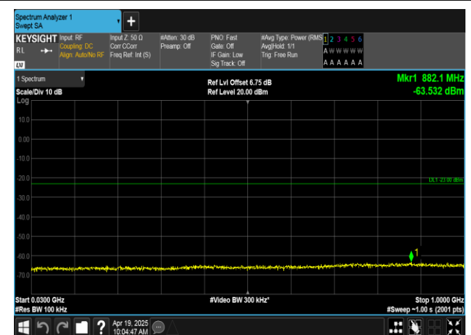
Band66-3MHz-16QAM-132657-1RB#0-30~1000-PASS
