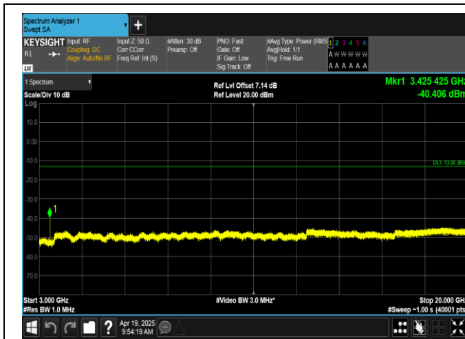
Band66-3MHz-16QAM-131987-1RB#14-3000~20000-PASS
