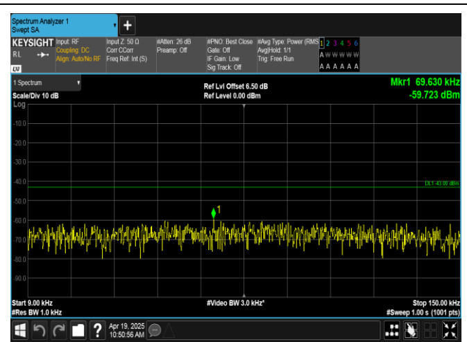
Band66-5MHz-QPSK-132322-25RB#0-0.009~0.15-PASS
