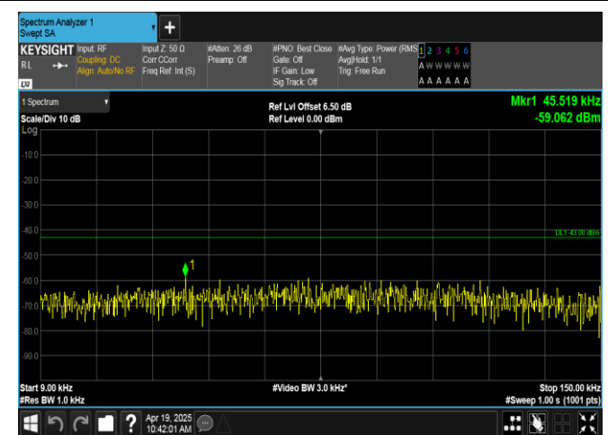
Band66-5MHz-QPSK-131997-1RB#24-0.009~0.15-PASS
