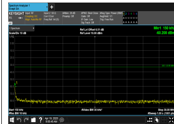
Band66-3MHz-16QAM-131987-15RB#0-0.15~30-PASS
