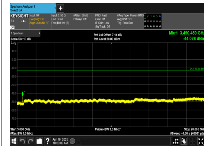
Band66-3MHz-16QAM-132322-15RB#0-3000~20000-PASS
