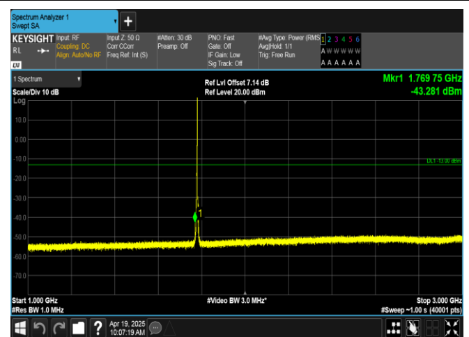
Band66-3MHz-16QAM-132657-1RB#14-1000~3000-PASS
