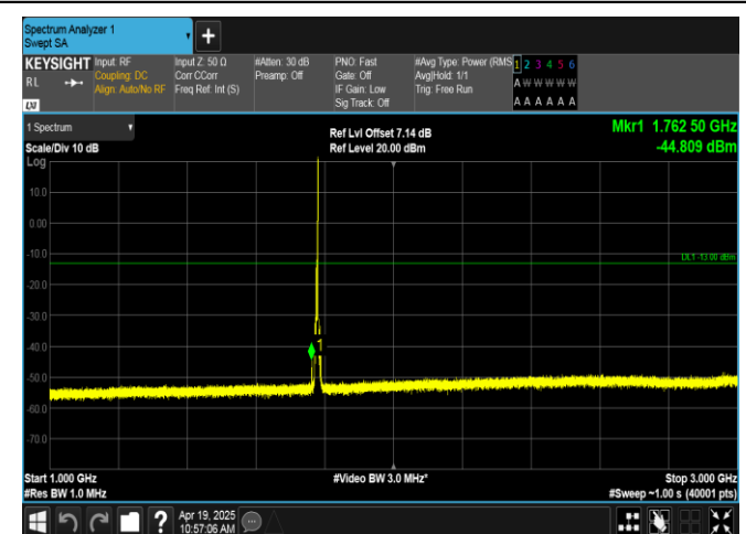
Band66-5MHz-16QAM-132647-1RB#24-1000~3000-PASS
