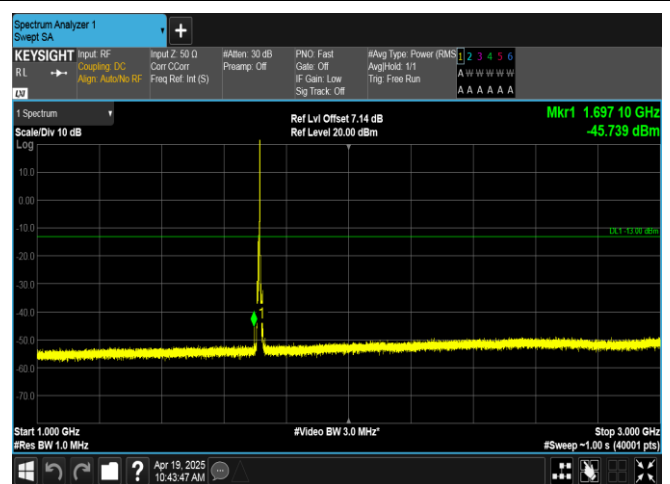
Band66-5MHz-16QAM-131997-1RB#24-1000~3000-PASS
