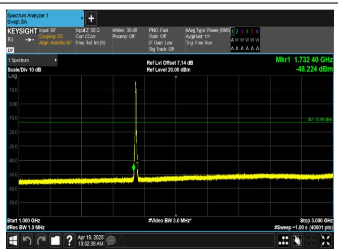
Band66-5MHz-16QAM-132322-25RB#0-1000~3000-PASS
