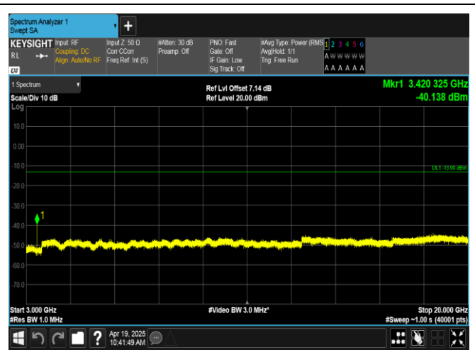
Band66-5MHz-16QAM-131997-1RB#0-3000~20000-PASS
