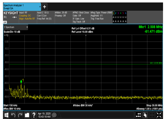
Band66-5MHz-16QAM-131997-1RB#24-0.15~30-PASS
