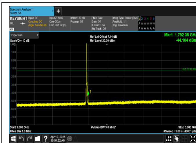
Band66-5MHz-16QAM-132647-1RB#0-1000~3000-PASS
