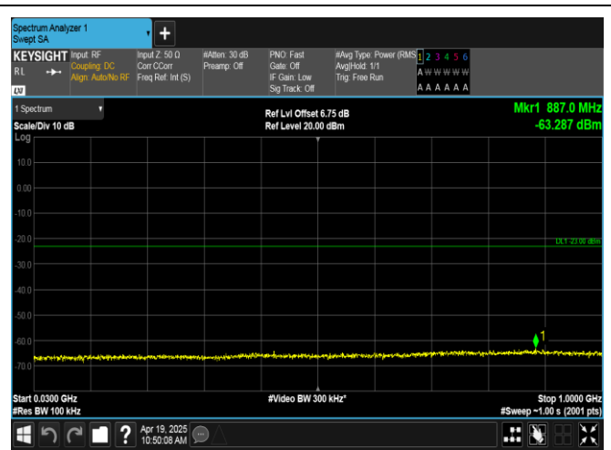
Band66-5MHz-16QAM-132322-1RB#24-30~1000-PASS
