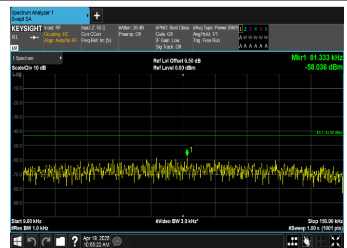
Band66-5MHz-QPSK-132647-1RB#24-0.009~0.15-PASS
