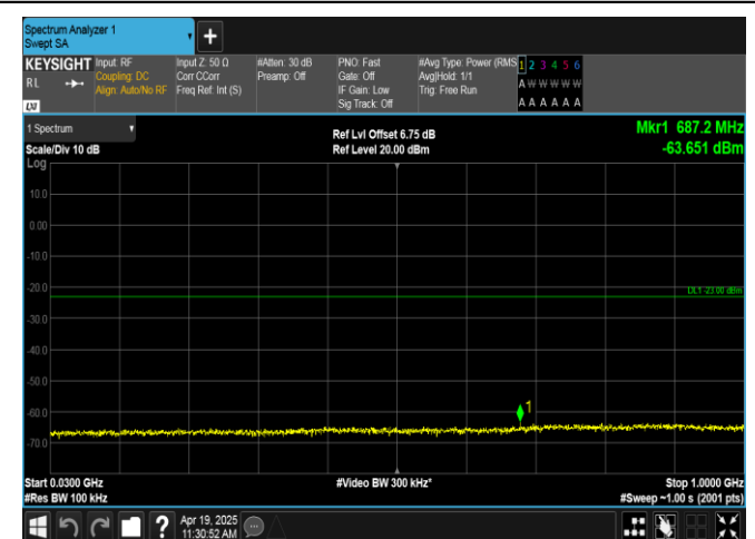
Band66-10MHz-QPSK-132322-1RB#0-30~1000-PASS
