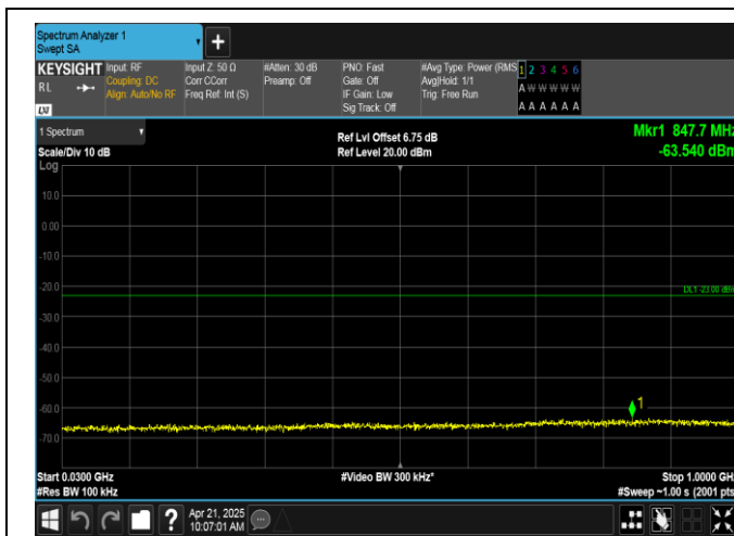
Band66-10MHz-QPSK-132022-50RB#0-30~1000-PASS
