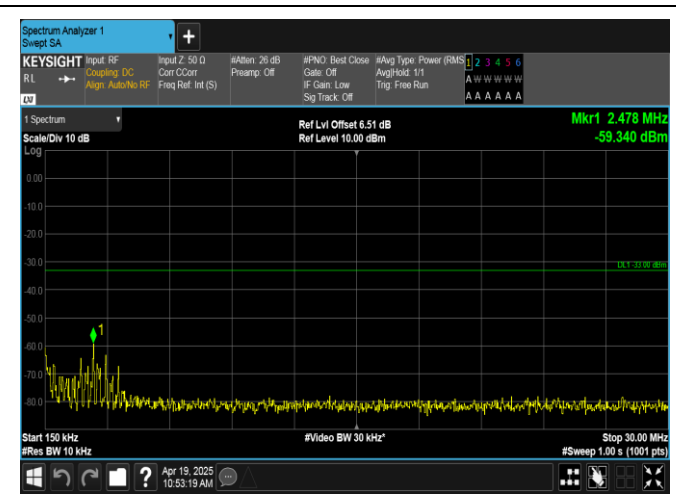
Band66-5MHz-QPSK-132647-1RB#0-0.15~30-PASS
