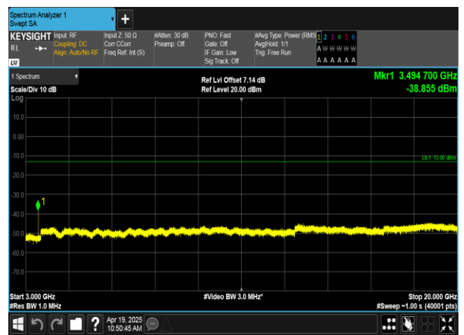
Band66-5MHz-16QAM-132322-1RB#24-3000~20000-PASS
