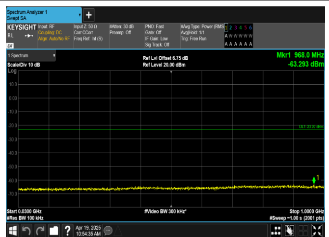
Band66-5MHz-16QAM-132647-1RB#0-30~1000-PASS
