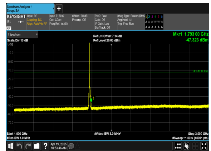
Band66-5MHz-QPSK-132647-1RB#0-1000~3000-PASS
