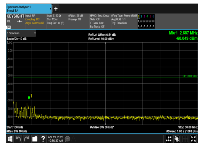
Band66-5MHz-16QAM-132647-1RB#24-0.15~30-PASS
