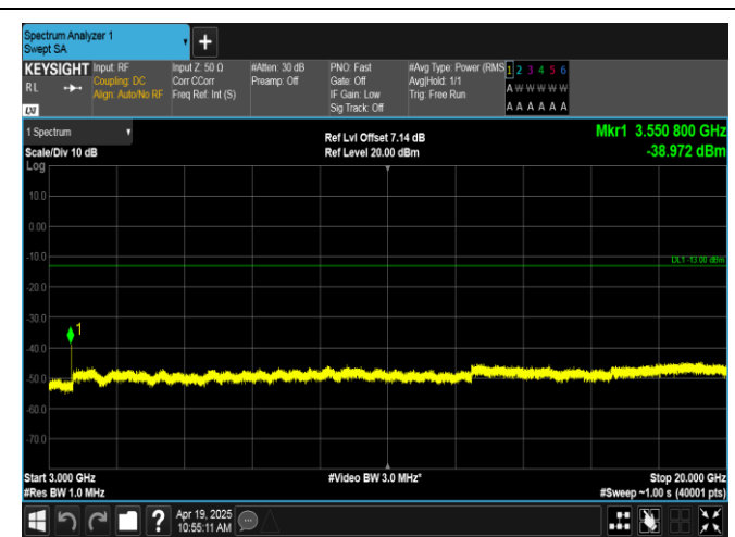
Band66-5MHz-16QAM-132647-1RB#0-3000~20000-PASS
