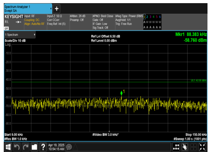
Band66-5MHz-16QAM-132647-1RB#0-0.009~0.15-PASS
