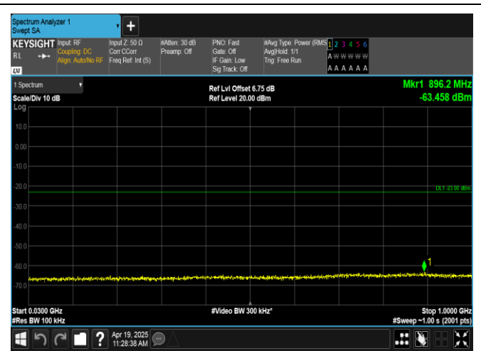
Band66-10MHz-QPSK-132022-1RB#49-30~1000-PASS
