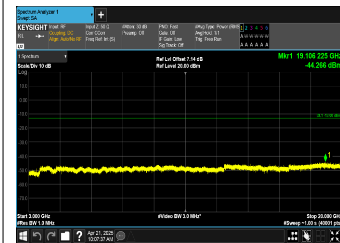
Band66-10MHz-QPSK-132022-50RB#0-3000~20000-PASS
