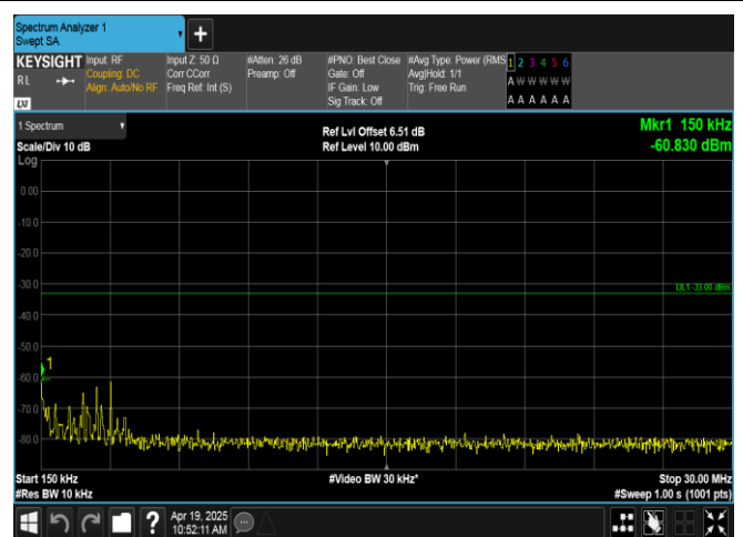
Band66-5MHz-16QAM-132322-25RB#0-0.15~30-PASS
