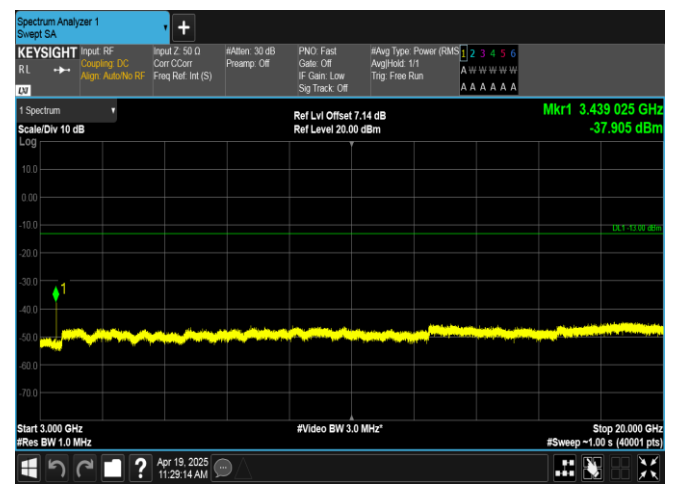
Band66-10MHz-QPSK-132022-1RB#49-3000~20000-PASS
