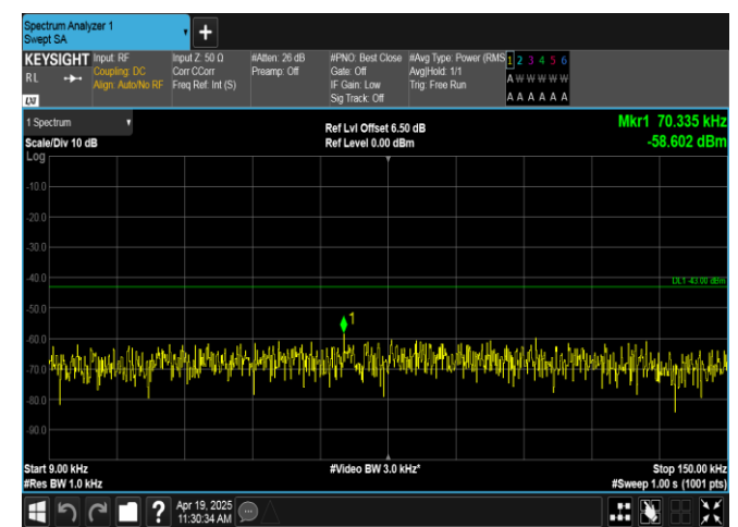
Band66-10MHz-QPSK-132322-1RB#0-0.009~0.15-PASS
