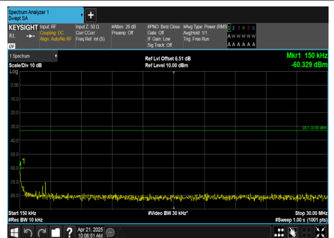
Band66-10MHz-QPSK-132022-50RB#0-0.15~30-PASS
