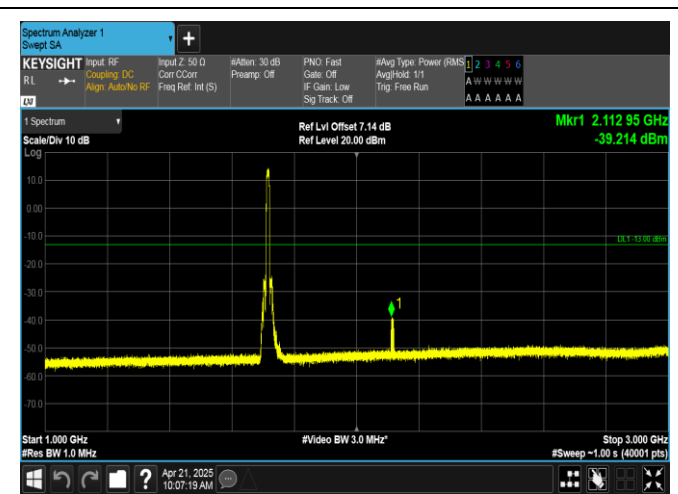
Band66-10MHz-QPSK-132022-50RB#0-1000~3000-PASS
