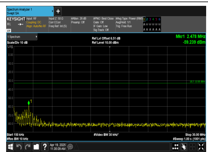
Band66-10MHz-QPSK-132622-1RB#0-0.15~30-PASS
