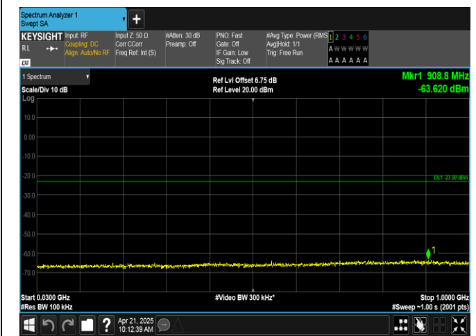
Band66-10MHz-16QAM-132622-50RB#0-30~1000-PASS
