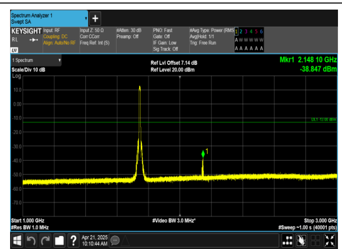
Band66-10MHz-16QAM-132322-50RB#0-1000~3000-PASS
