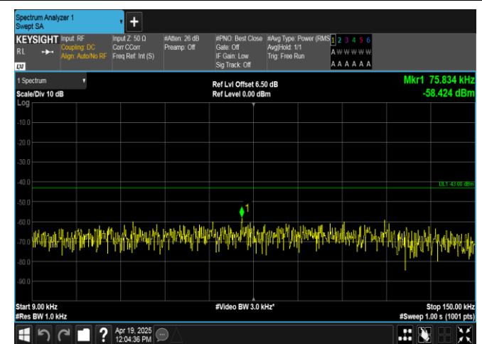
Band66-15MHz-QPSK-132047-1RB#74-0.009~0.15-PASS
