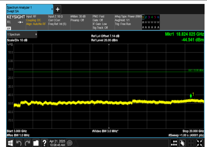
Band66-10MHz-16QAM-132022-50RB#0-3000~20000-PASS
