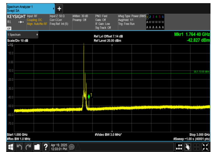
Band66-15MHz-QPSK-132047-1RB#0-1000~3000-PASS
