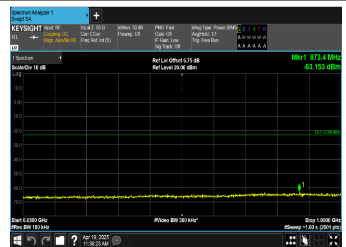
Band66-10MHz-16QAM-132622-1RB#0-30~1000-PASS
