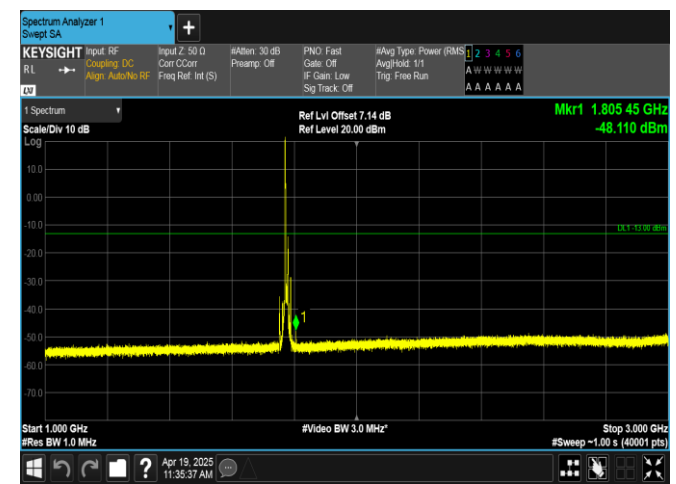
Band66-10MHz-QPSK-132622-1RB#0-1000~3000-PASS
