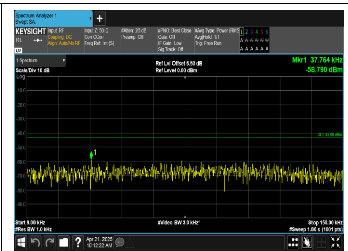
Band66-10MHz-16QAM-132622-50RB#0-0.009~0.15-PASS
