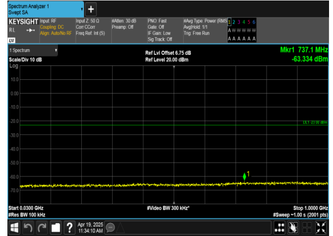
Band66-10MHz-16QAM-132322-1RB#49-30~1000-PASS
