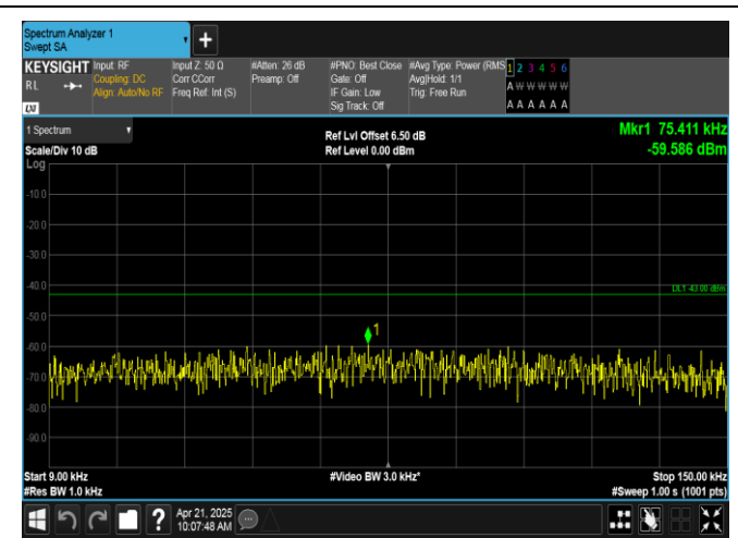
Band66-10MHz-16QAM-132022-50RB#0-0.009~0.15-PASS
