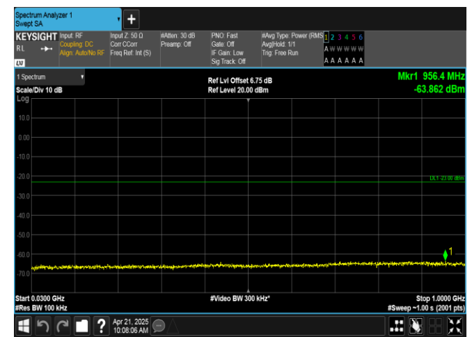
Band66-10MHz-16QAM-132022-50RB#0-30~1000-PASS
