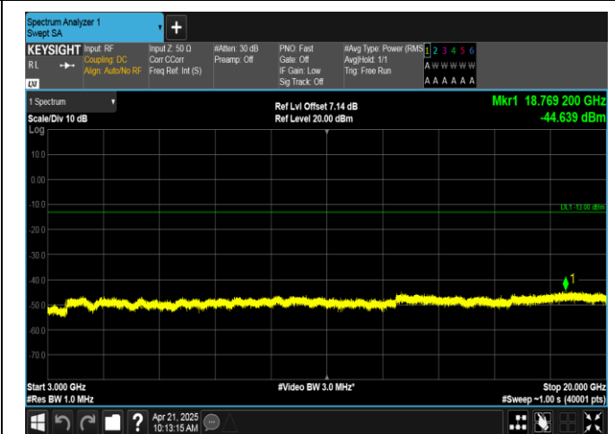
Band66-10MHz-16QAM-132622-50RB#0-3000~20000-PASS
