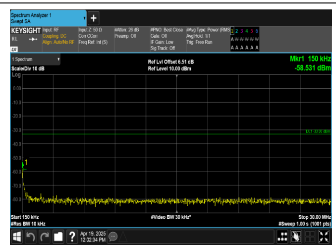
Band66-15MHz-QPSK-132047-1RB#0-0.15~30-PASS
