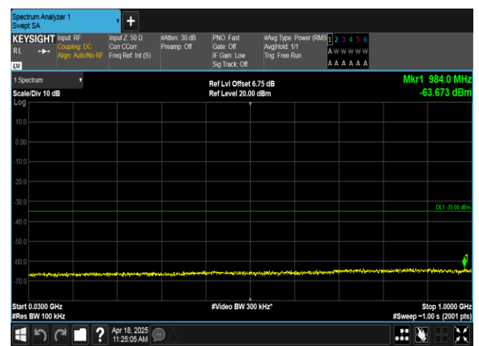
Band7-10MHz-16QAM-21400-1RB#0-30~1000-PASS
