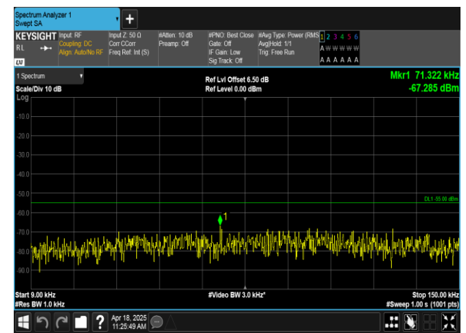
Band7-10MHz-QPSK-21400-1RB#49-0.009~0.15-PASS
