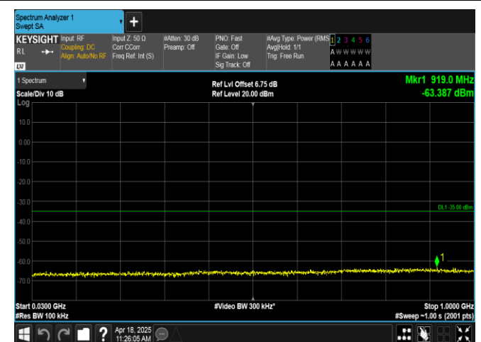
Band7-10MHz-QPSK-21400-1RB#49-30~1000-PASS
