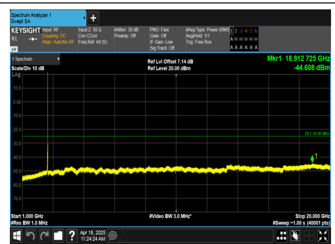
Band7-10MHz-QPSK-21400-1RB#0-1000~20000-PASS
