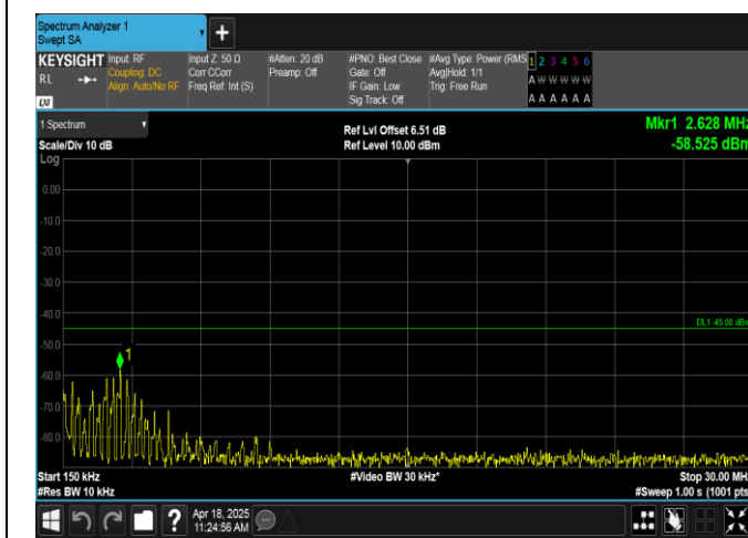
Band7-10MHz-16QAM-21400-1RB#0-0.15~30-PASS
