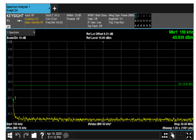
Band7-10MHz-QPSK-20800-50RB#0-0.15~30-PASS
