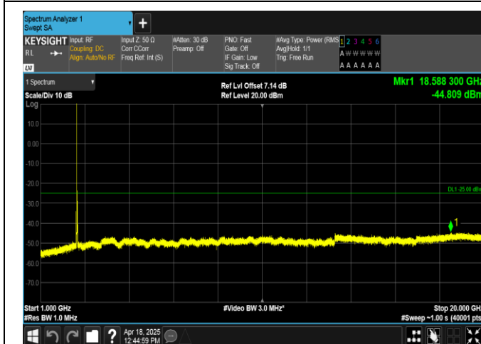
Band7-20MHz-16QAM-21350-1RB#0-1000~20000-PASS
