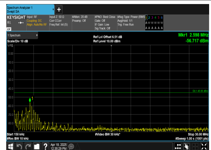
Band7-20MHz-QPSK-20850-1RB#0-0.15~30-PASS
