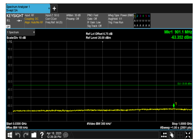
Band7-20MHz-QPSK-21100-1RB#0-30~1000-PASS
