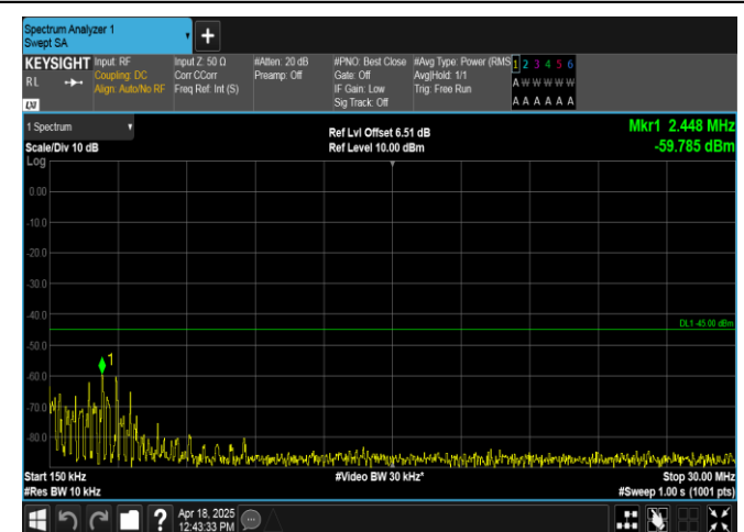
Band7-20MHz-QPSK-21350-1RB#0-0.15~30-PASS
