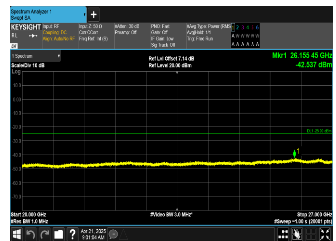
Band7-20MHz-QPSK-21100-100RB#0-20000~27000-PASS
