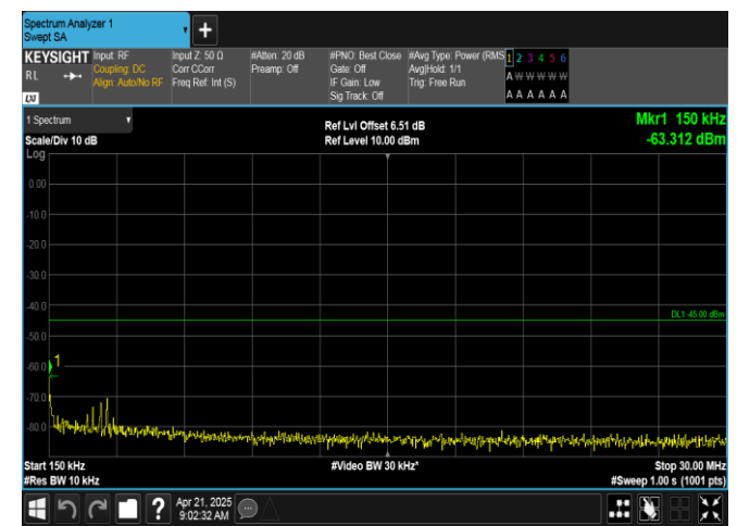
Band7-20MHz-QPSK-21350-100RB#0-0.15~30-PASS
