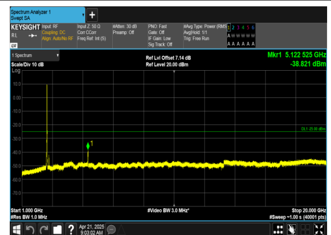
Band7-20MHz-QPSK-21350-100RB#0-1000~20000-PASS
