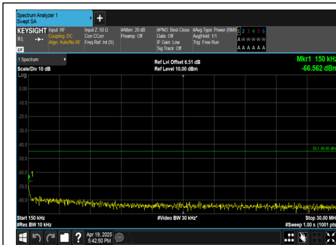
Band7-15MHz-16QAM-21375-75RB#0-0.15~30-PASS
