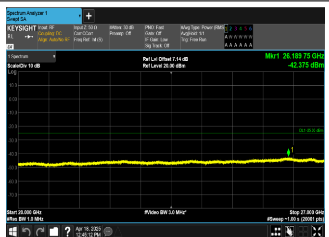
Band7-20MHz-16QAM-21350-1RB#0-20000~27000-PASS
