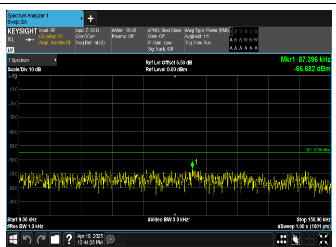
Band7-20MHz-16QAM-21350-1RB#0-0.009~0.15-PASS
