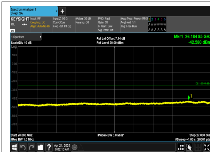
Band7-20MHz-16QAM-21100-100RB#0-20000~27000-PASS
