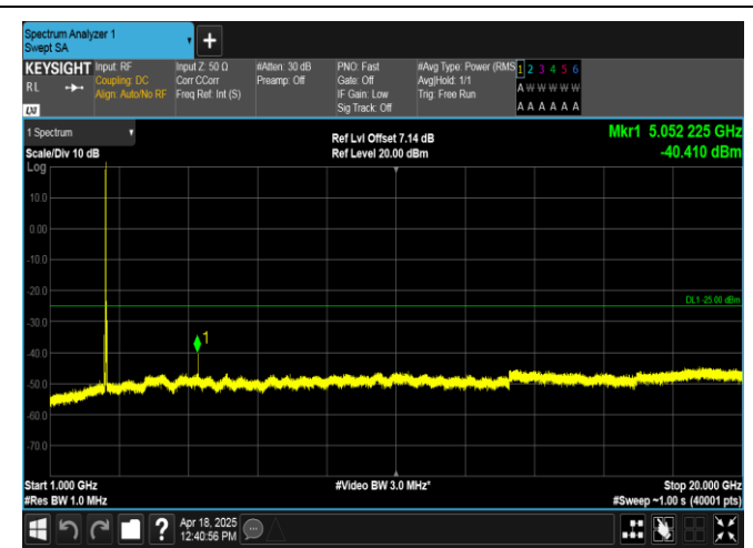
Band7-20MHz-16QAM-21100-1RB#0-1000~20000-PASS
