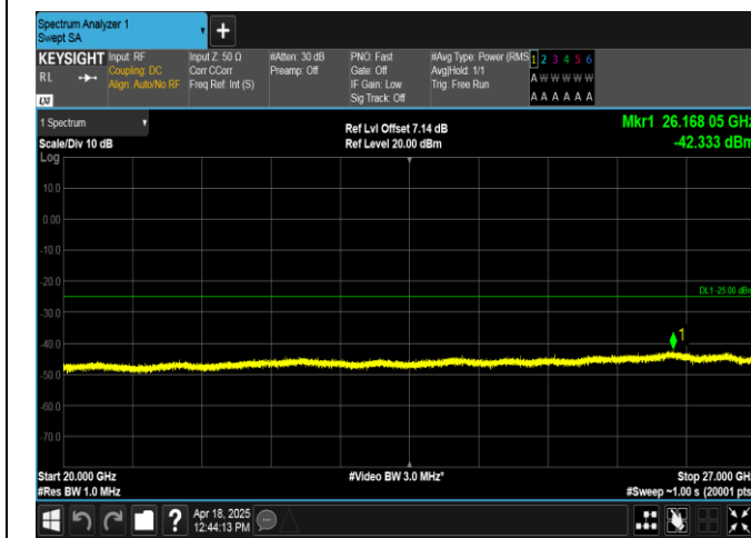
Band7-20MHz-QPSK-21350-1RB#0-20000~27000-PASS
