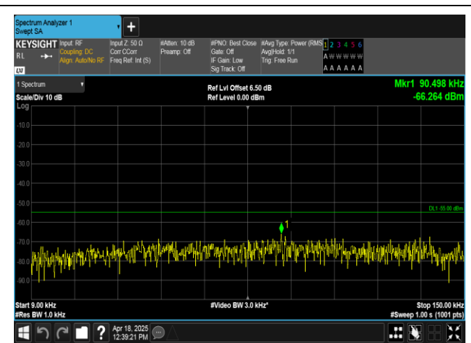
Band7-20MHz-QPSK-21100-1RB#0-0.009~0.15-PASS
