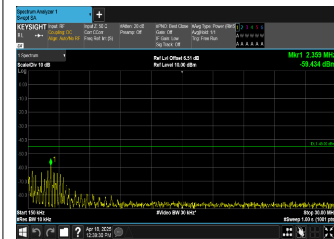
Band7-20MHz-QPSK-21100-1RB#0-0.15~30-PASS
