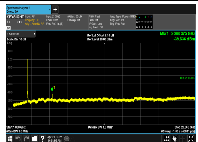
Band7-20MHz-16QAM-21100-100RB#0-1000~20000-PASS
