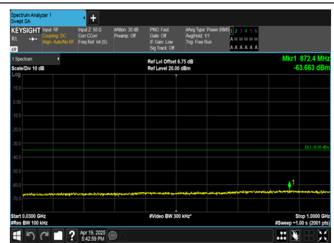
Band7-15MHz-16QAM-21375-75RB#0-30~1000-PASS
