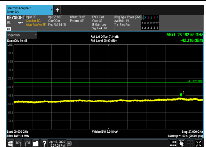
Band7-20MHz-16QAM-20850-1RB#0-20000~27000-PASS
