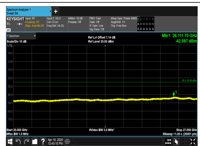
Band7-20MHz-16QAM-21100-1RB#99-20000~27000-PASS
