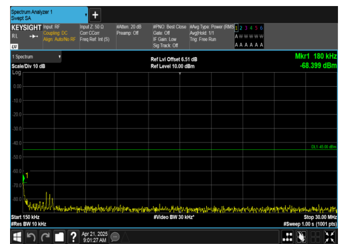
Band7-20MHz-16QAM-21100-100RB#0-0.15~30-PASS
