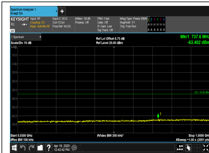
Band7-20MHz-QPSK-21350-1RB#0-30~1000-PASS
