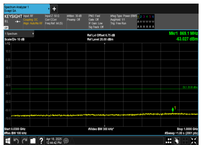
Band7-20MHz-16QAM-21350-1RB#0-30~1000-PASS
