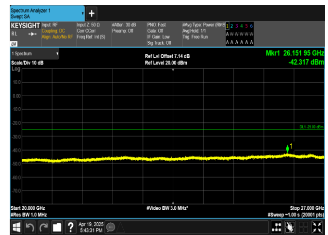
Band7-15MHz-16QAM-21375-75RB#0-20000~27000-PASS
