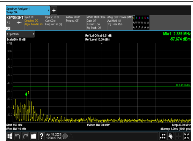
Band7-20MHz-16QAM-20850-1RB#99-0.15~30-PASS
