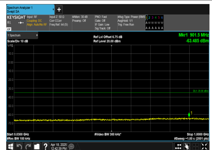
Band7-20MHz-16QAM-21100-1RB#99-30~1000-PASS
