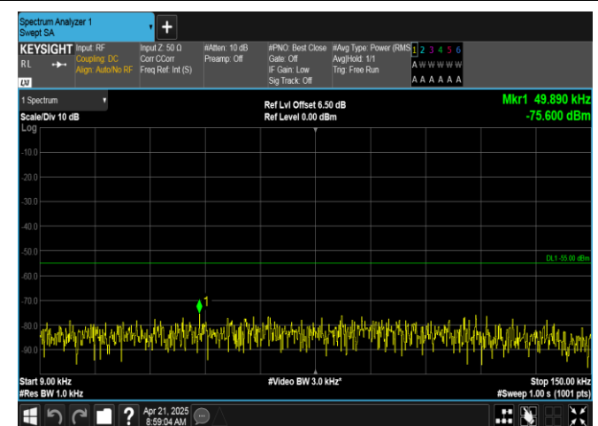
Band7-20MHz-16QAM-20850-100RB#0-0.009~0.15-PASS
