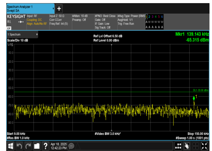
Band7-20MHz-16QAM-21100-1RB#99-0.009~0.15-PASS
