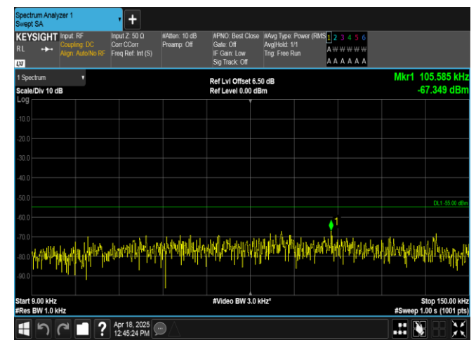
Band7-20MHz-QPSK-21350-1RB#99-0.009~0.15-PASS
