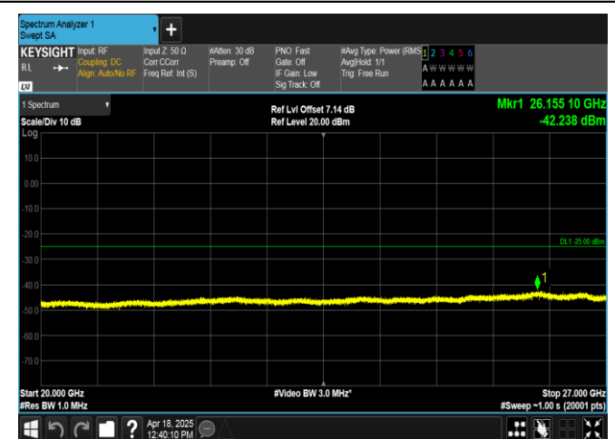
Band7-20MHz-QPSK-21100-1RB#0-20000~27000-PASS
