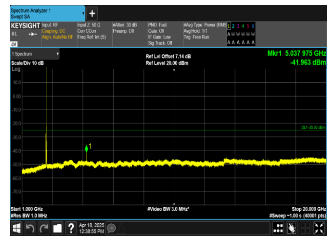
Band7-20MHz-16QAM-20850-1RB#99-1000~20000-PASS
