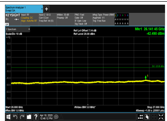
Band7-20MHz-QPSK-21350-1RB#99-20000~27000-PASS
