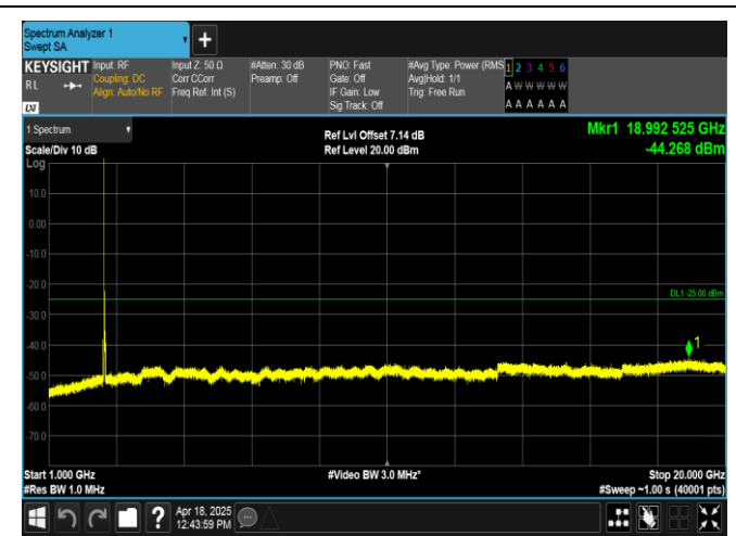
Band7-20MHz-QPSK-21350-1RB#0-1000~20000-PASS
