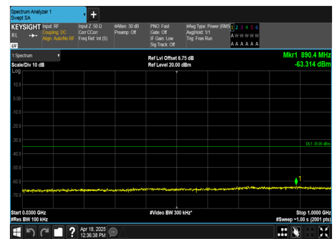
Band7-20MHz-16QAM-20850-1RB#0-30~1000-PASS
