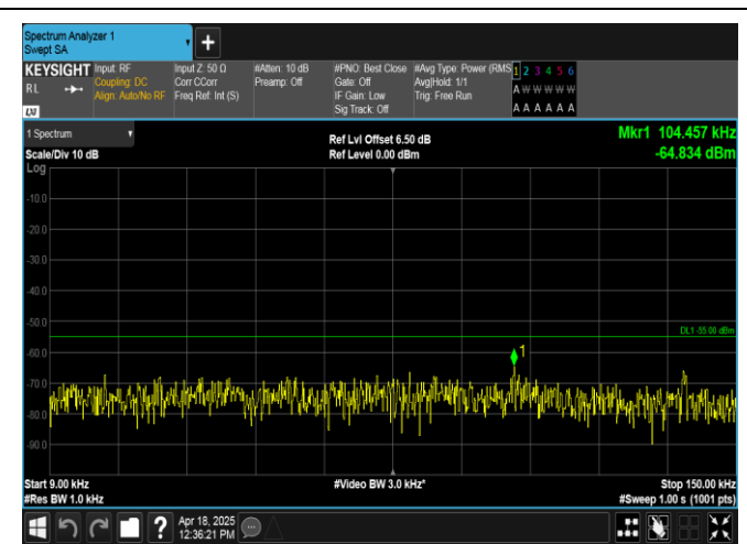
Band7-20MHz-16QAM-20850-1RB#0-0.009~0.15-PASS
