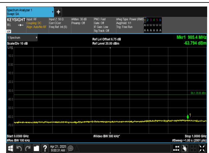
Band7-20MHz-QPSK-21100-100RB#0-30~1000-PASS
