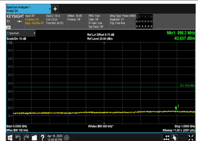
Band7-20MHz-QPSK-21350-1RB#99-30~1000-PASS
