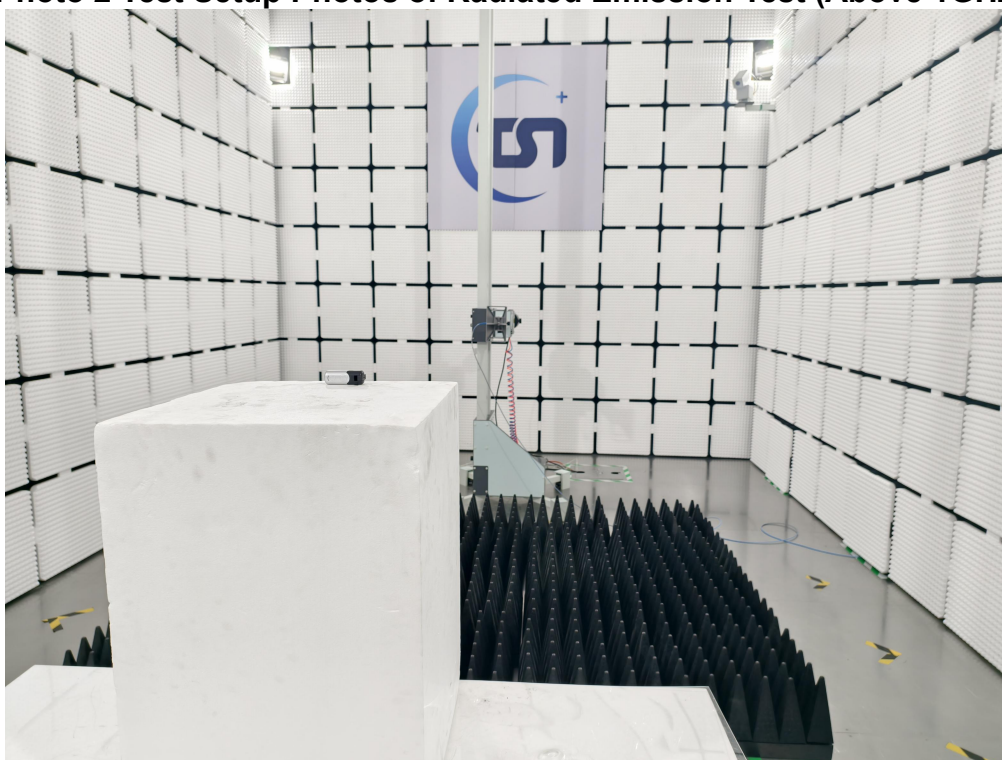
Photo 2 Test Setup Photos of Radiated Emission Test (Above 1GHz)
