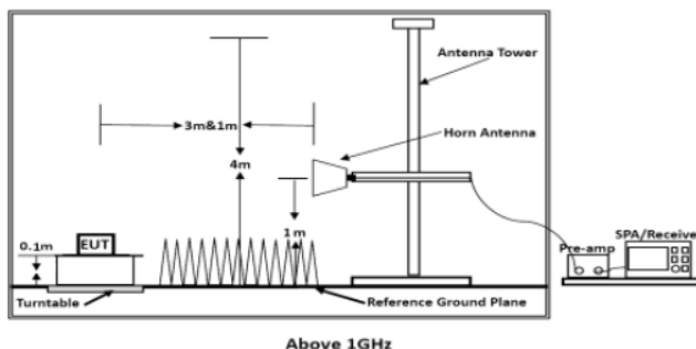
Figure 3. Above 1GHz
