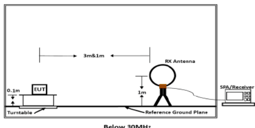
Figure 1. Below 30MHz
